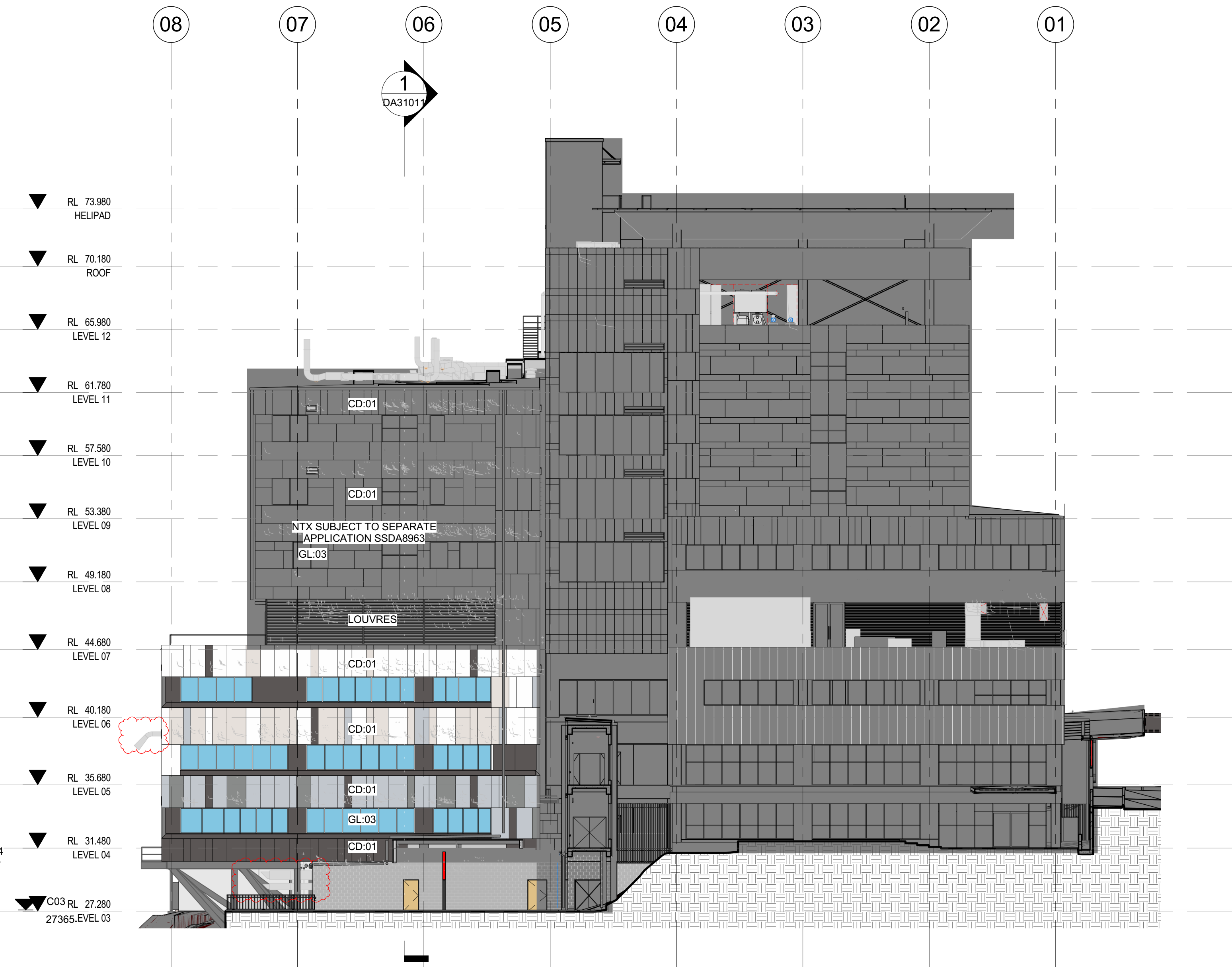
2 Building Elevation - West 3B2 1 : 200
