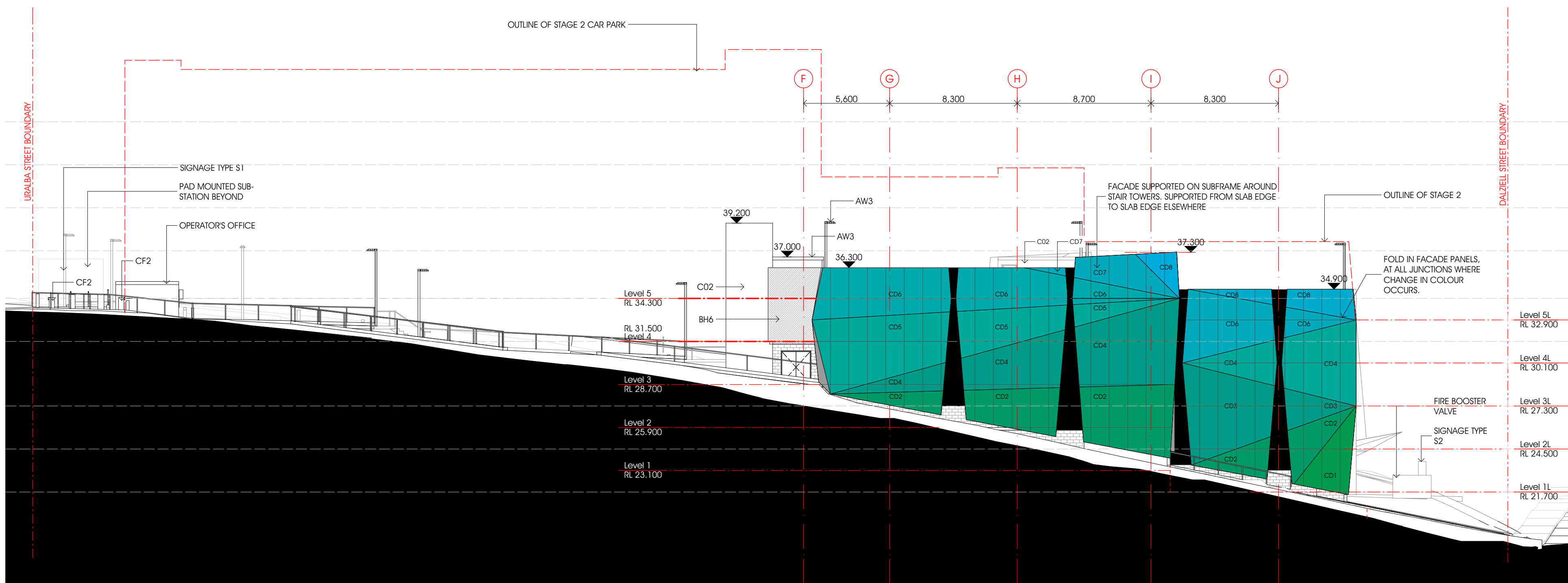
4 WESTERN ELEVATION 1:200
