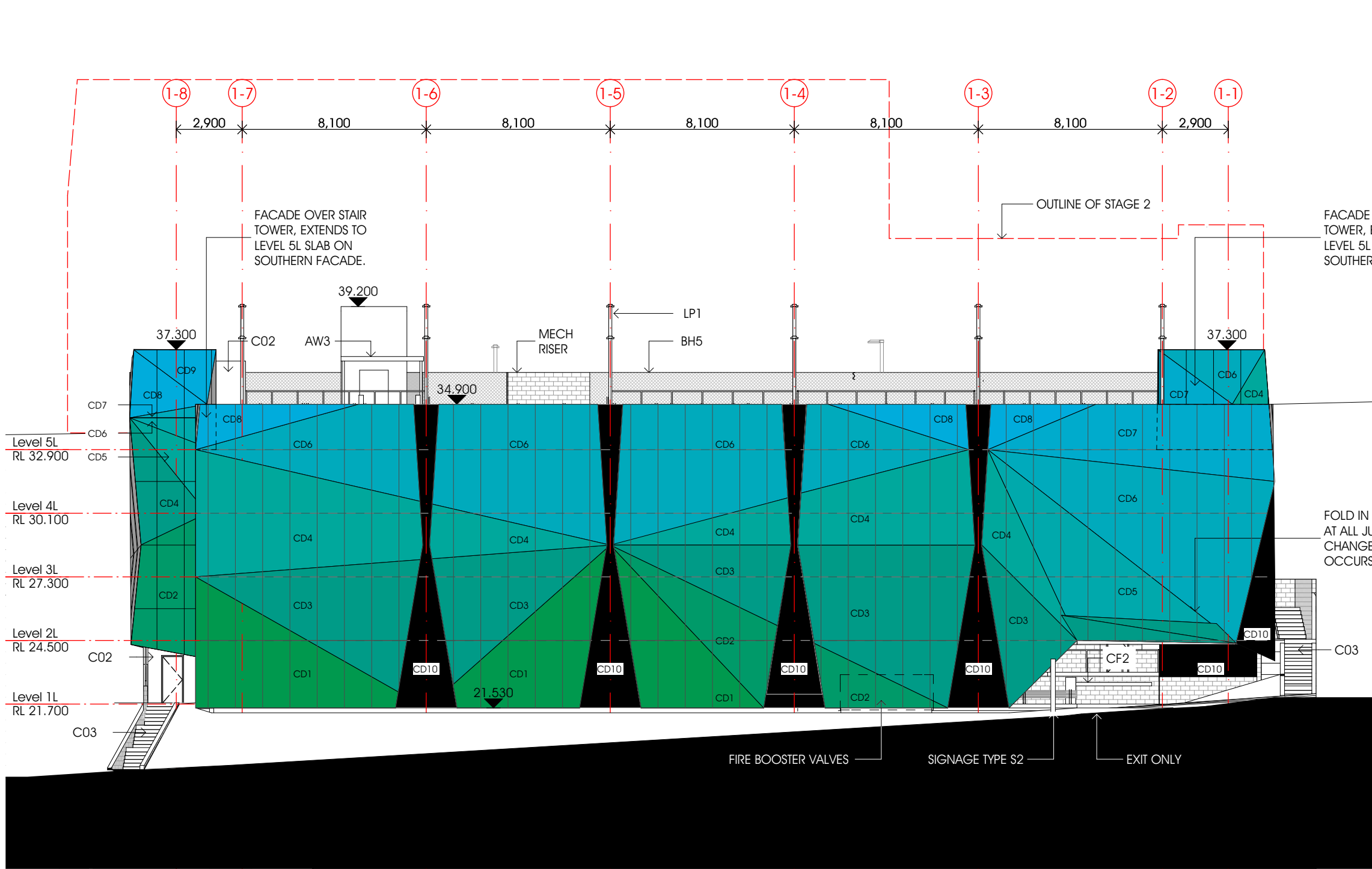
1 SOUTHERN ELEVATION 1:200
