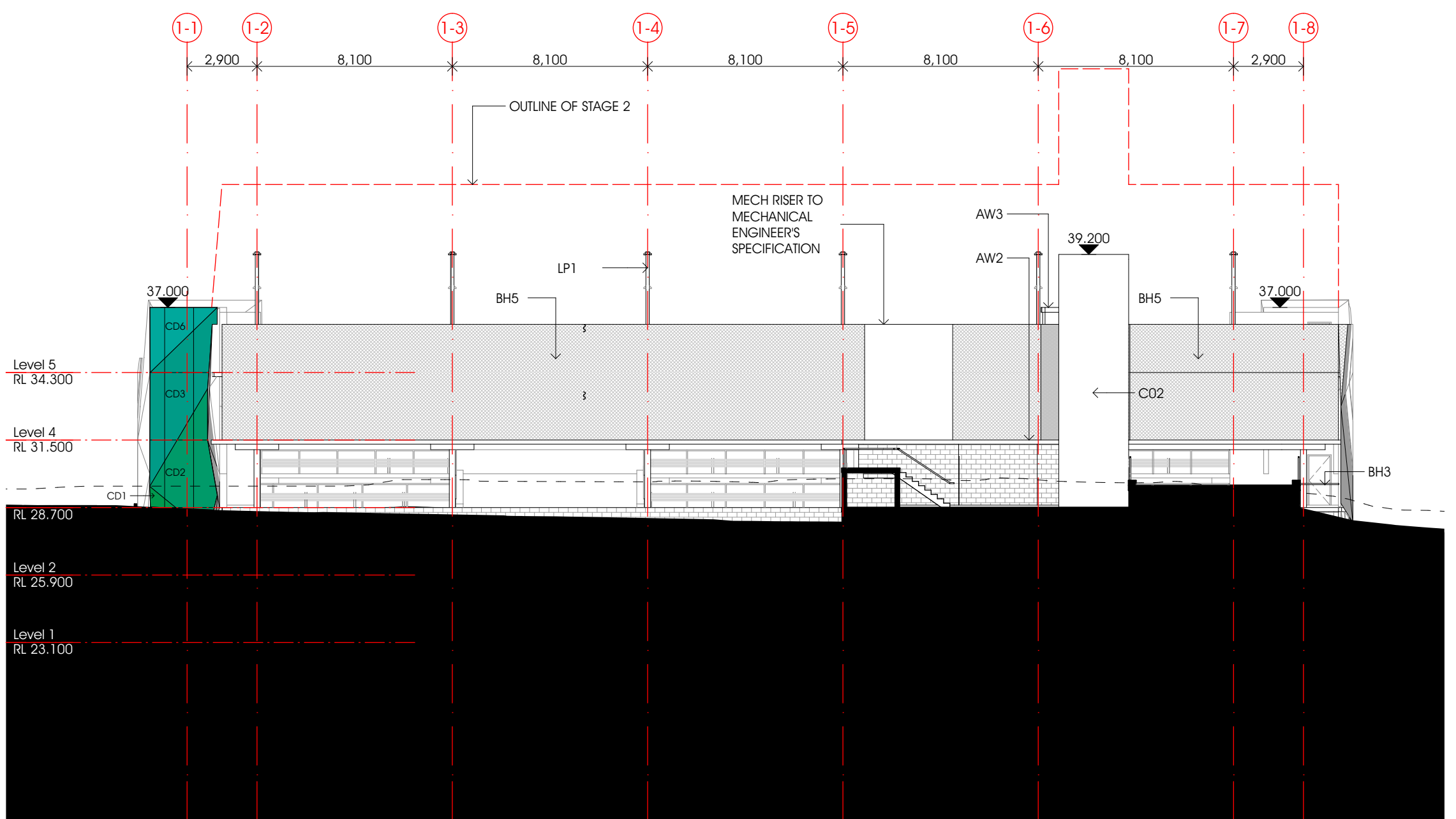
2 NORTHERN ELEVATION 1:200
