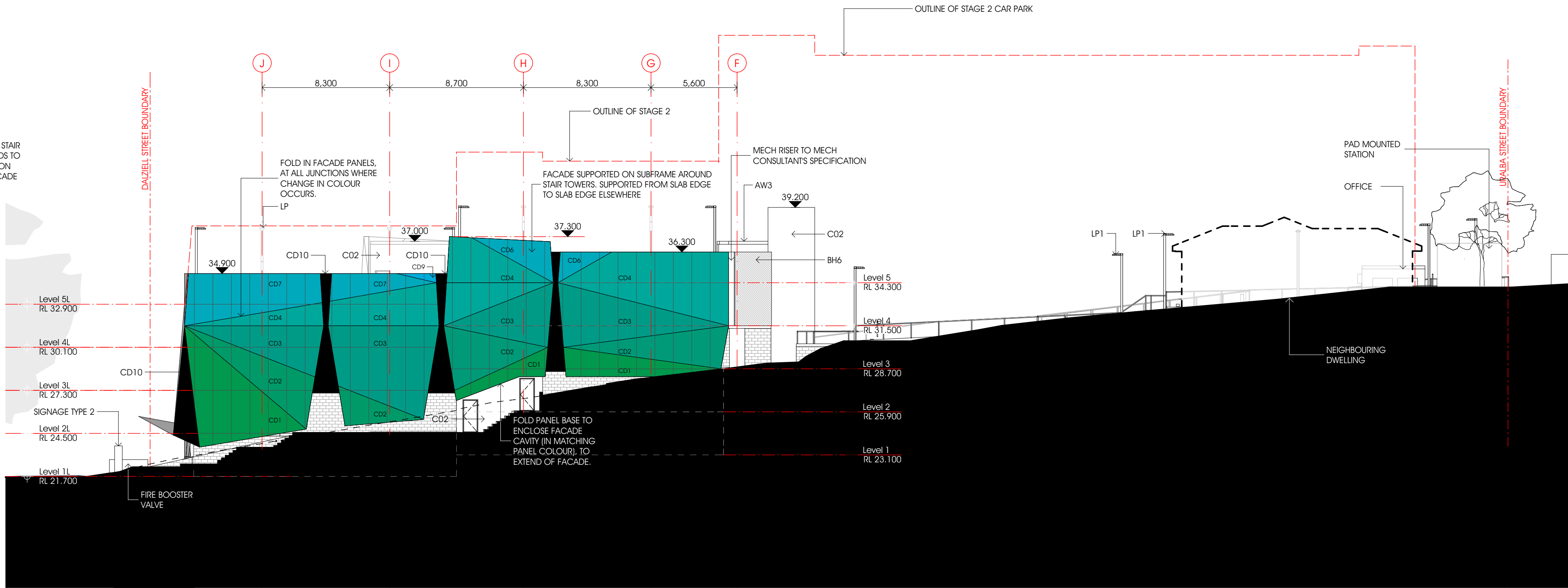
3 EASTERN ELEVATION 1:200
