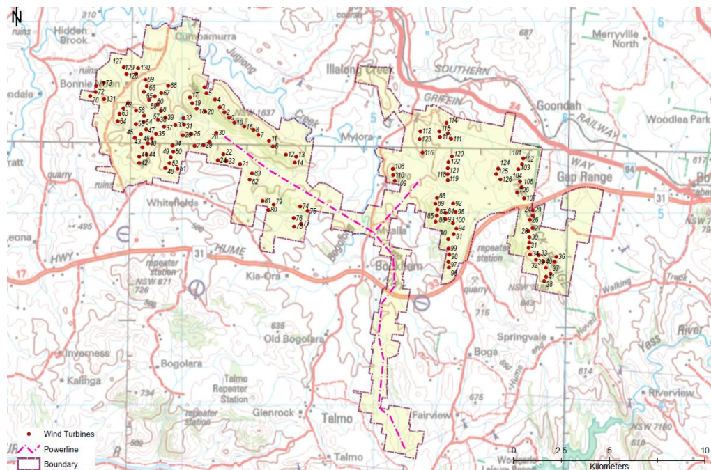
Site layout - EA Application
