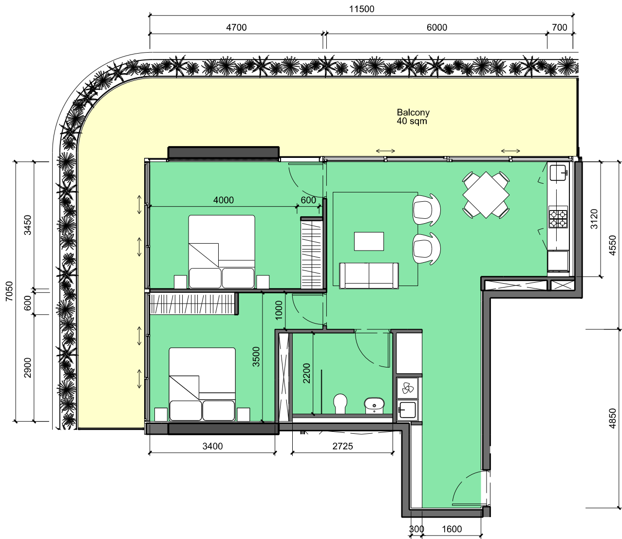
01 Level 11 - 2-Bed Adaptable Apartment - Pre-Adaptable 1:100
