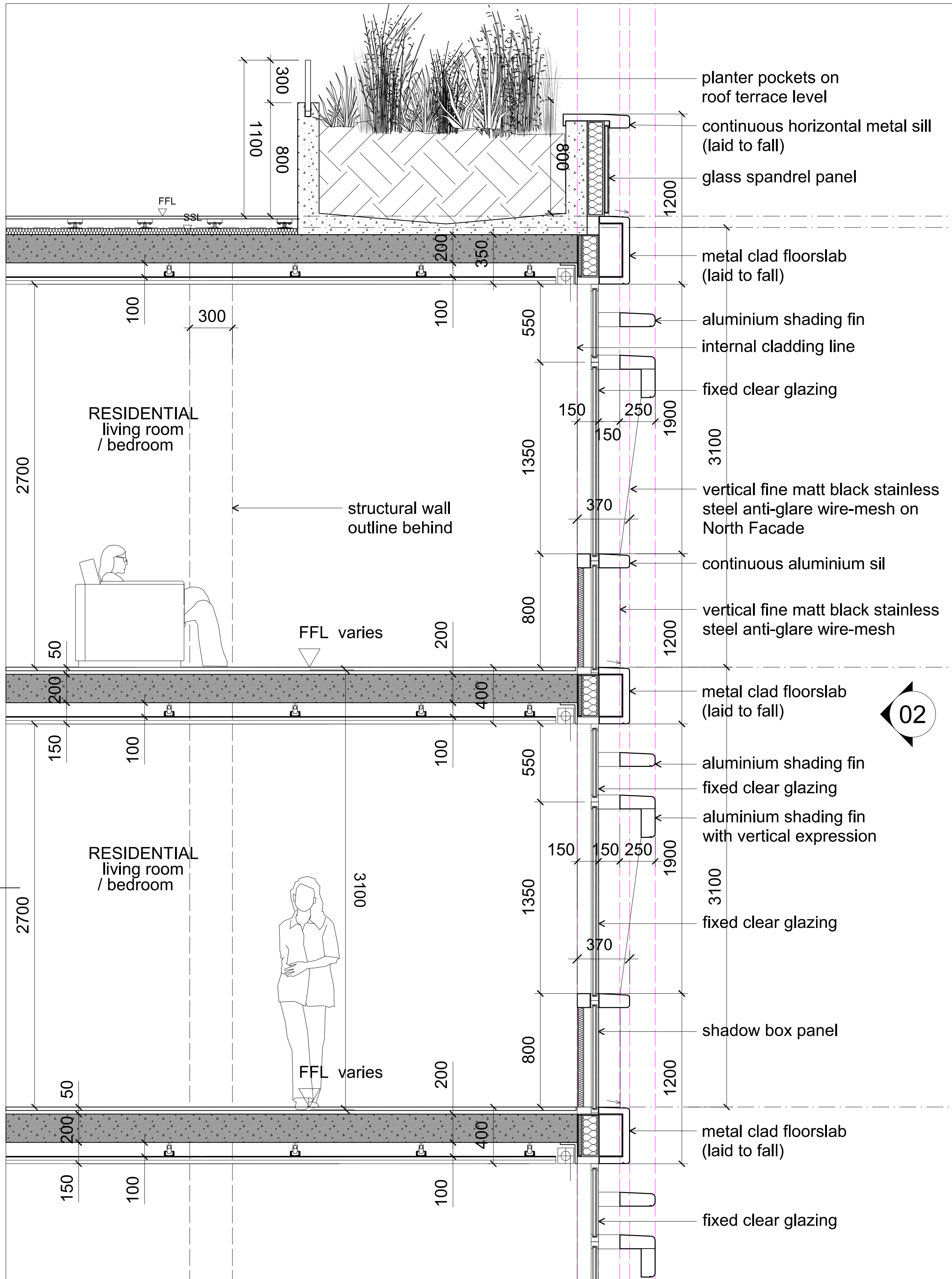
01 Cladding Type R1 - Typical Residential Facade - Section
