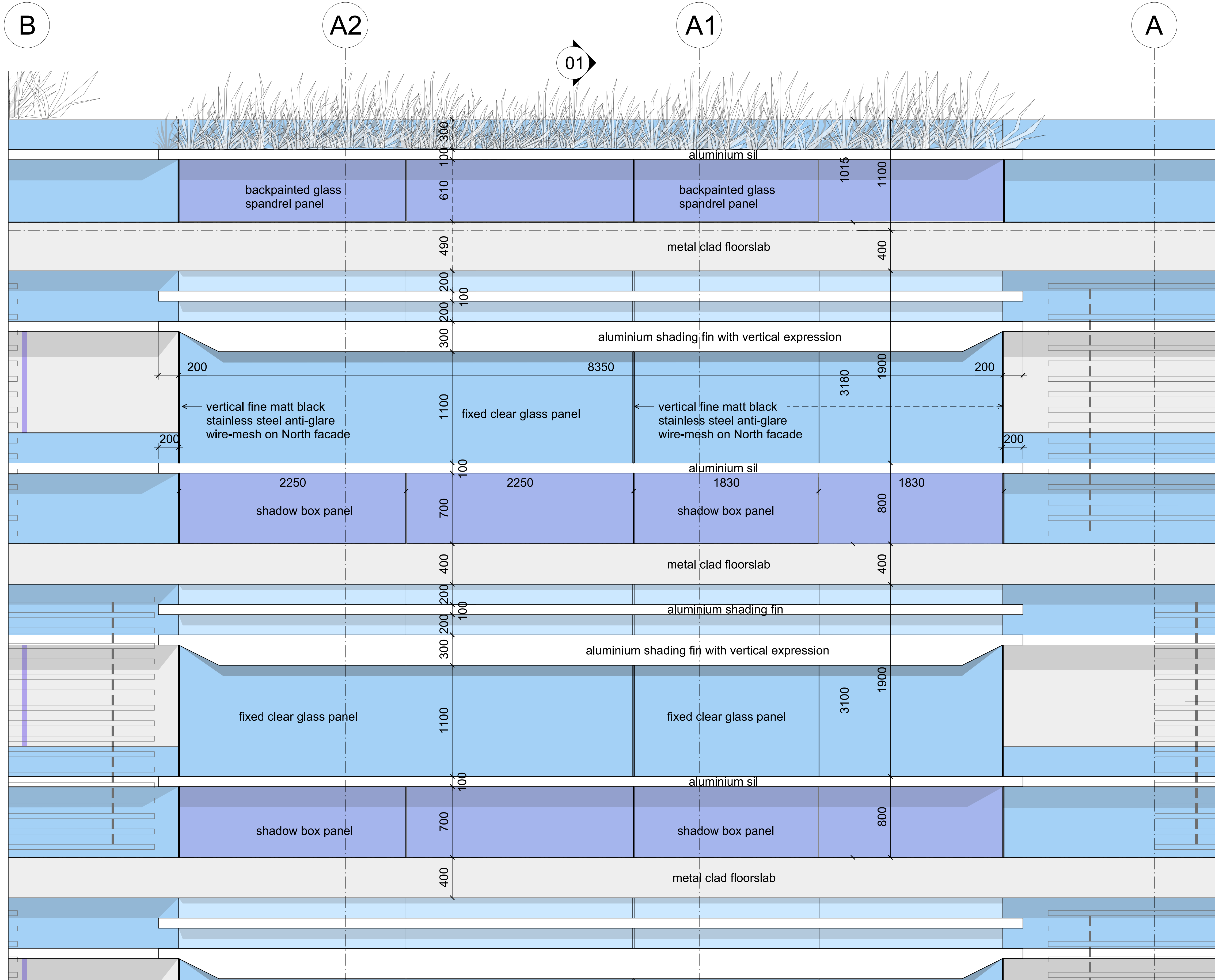
02 Cladding Type R1 - Typical Residential Facade - Elevation
