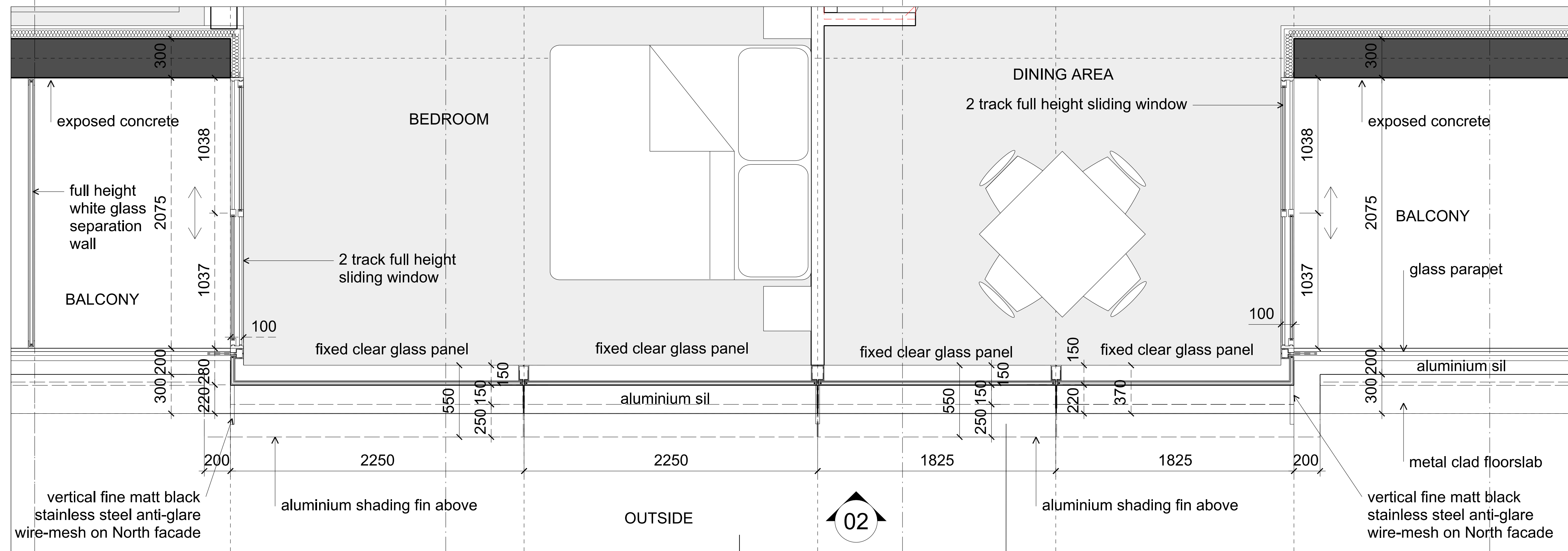
03 Cladding Type R1 - Typical Residential Facade - Plan
