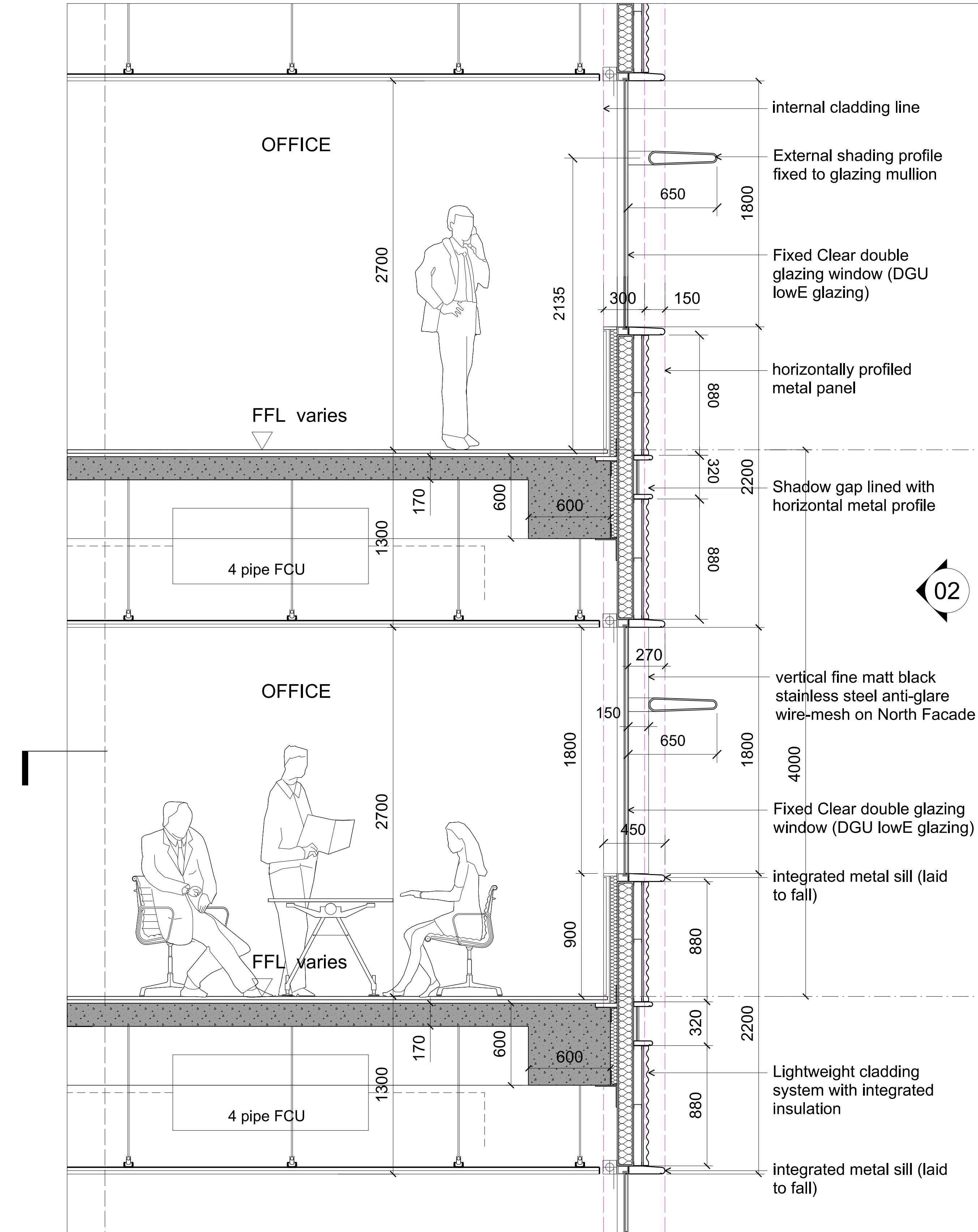
01 Cladding Type O1 - Typical Office / Childcare Facade - Section
