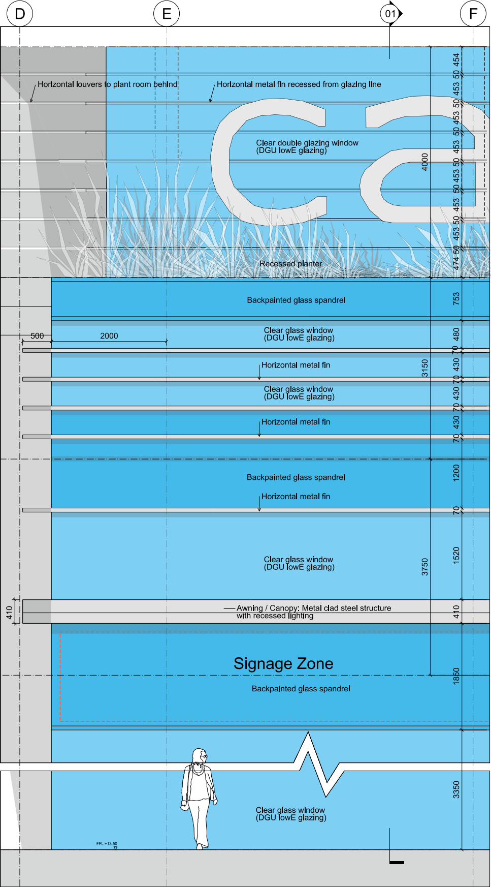
Typical Section and Elevation through Podium Façade - Hotel Entrance lobby with Hotel Rooms above, NTS
