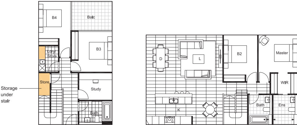
Type 4C Storage volume provided within apartment: 5.9m³ Storage cage provided in basement: Yes - 4m³ Total storage volume compliant with SEPP 65 / SOPA guidelines (10.0 m³): Yes
