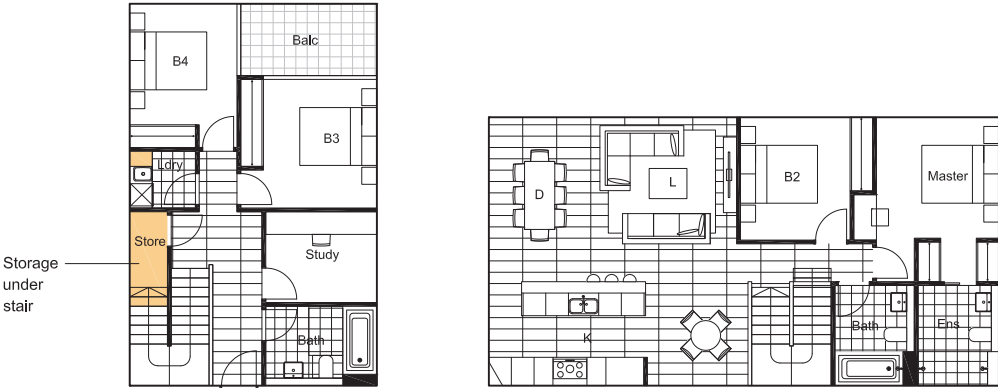
Type 4E Storage volume provided within apartment: 5.5m³ Storage cage provided in basement: Yes - 4m³ Total storage volume compliant with SEPP 65 / SOPA guidelines (10.0 m³): Yes
