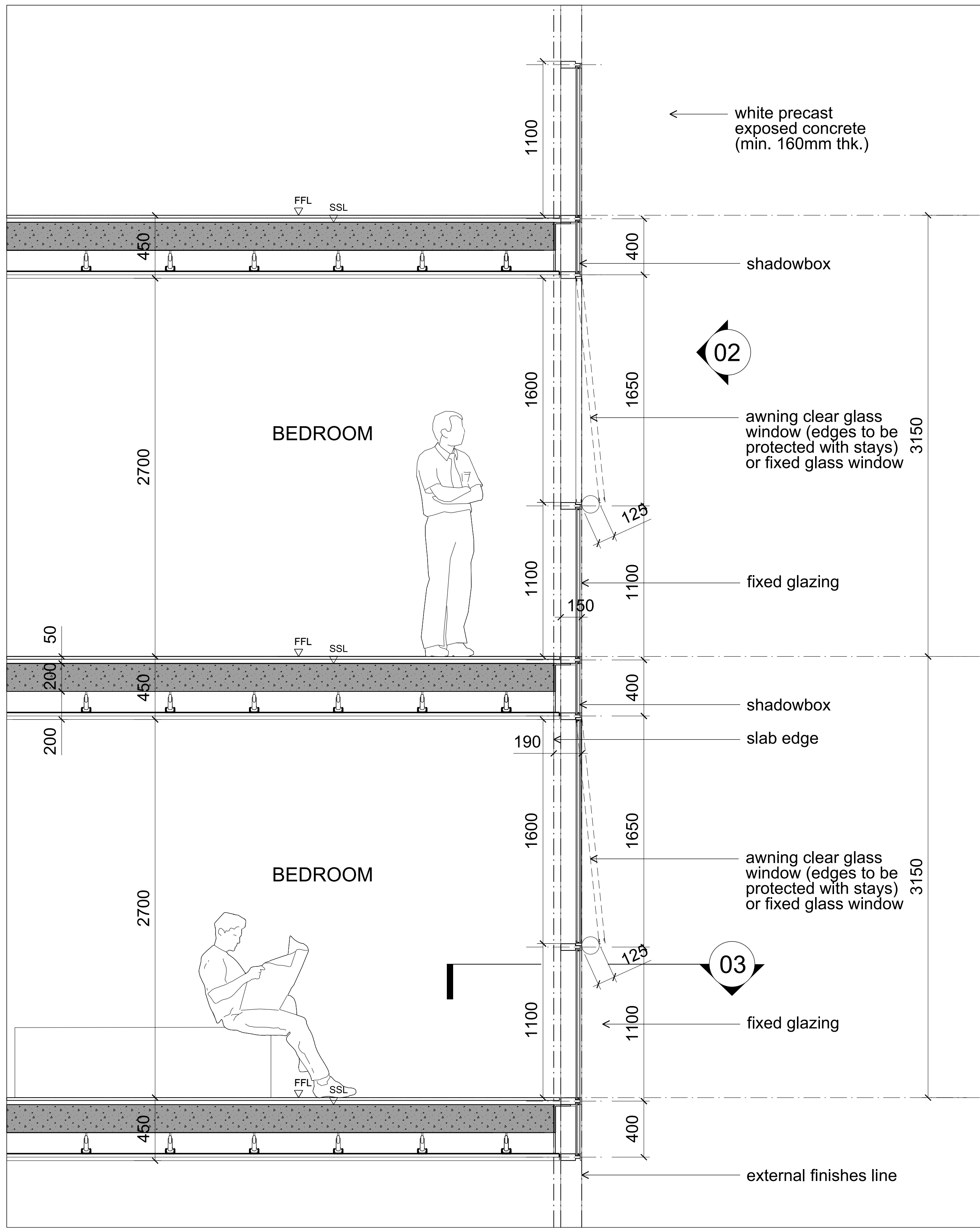
01 Cladding Type D - Typical Bedroom Slot Facade - Section 1:20
