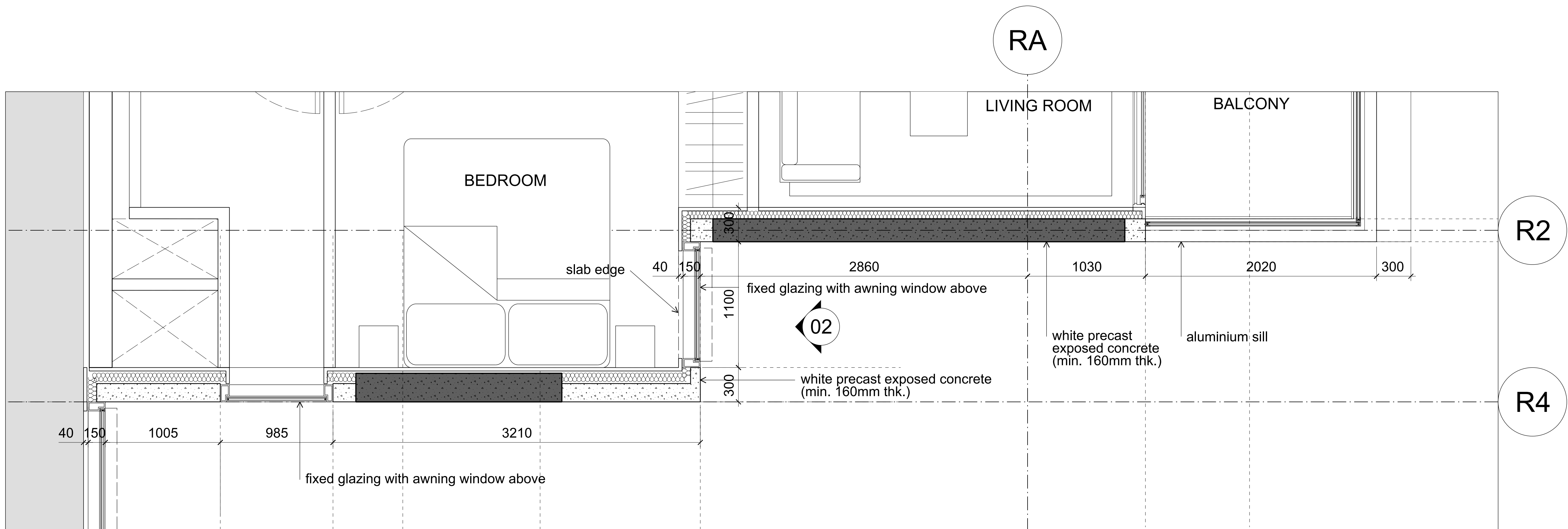
03 Cladding Type D - Typical Bedroom Slot Facade - Plan 1:20
