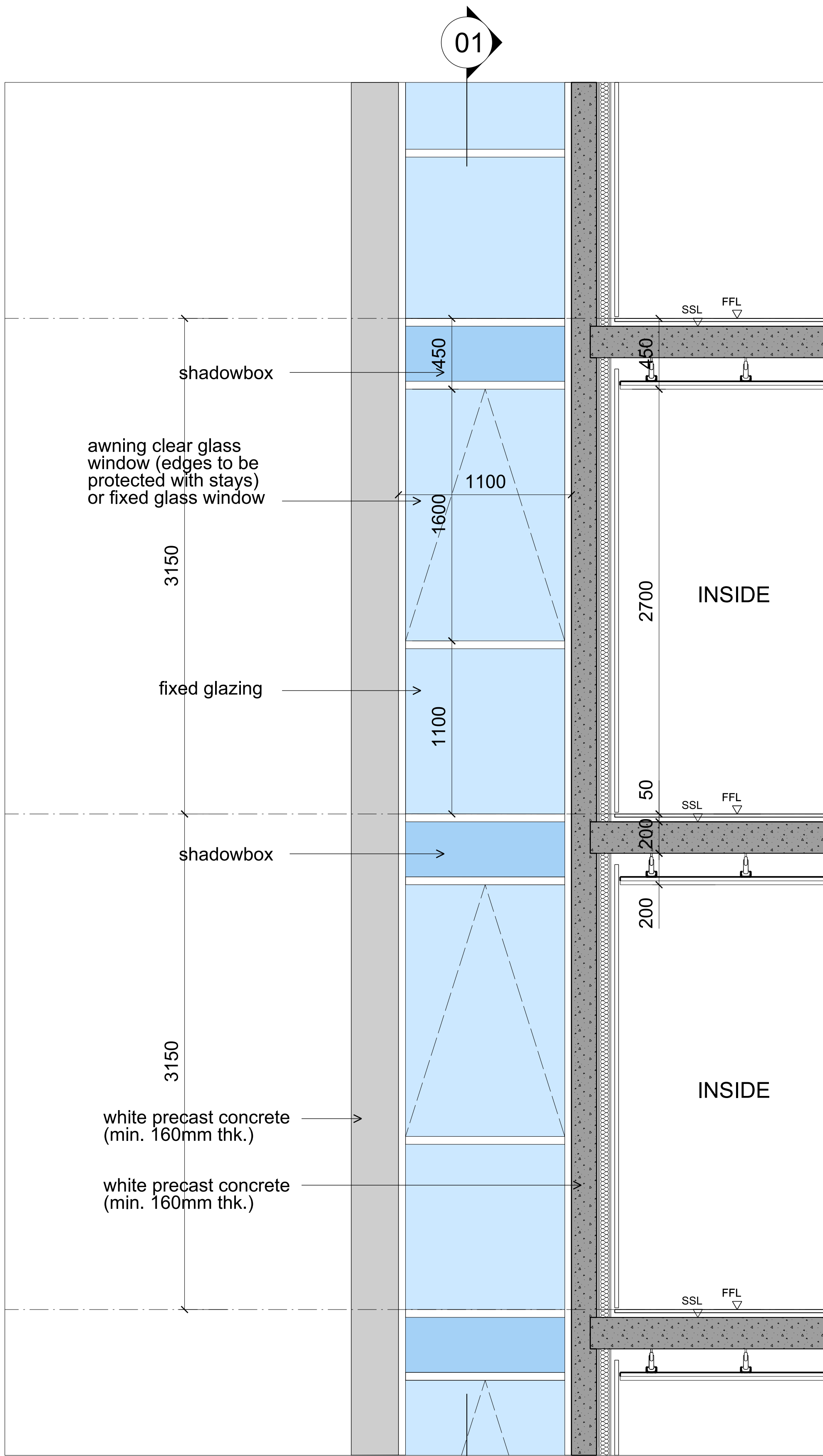
02 Cladding Type D - Typical Bedroom Slot Facade - Elevation 1:20
