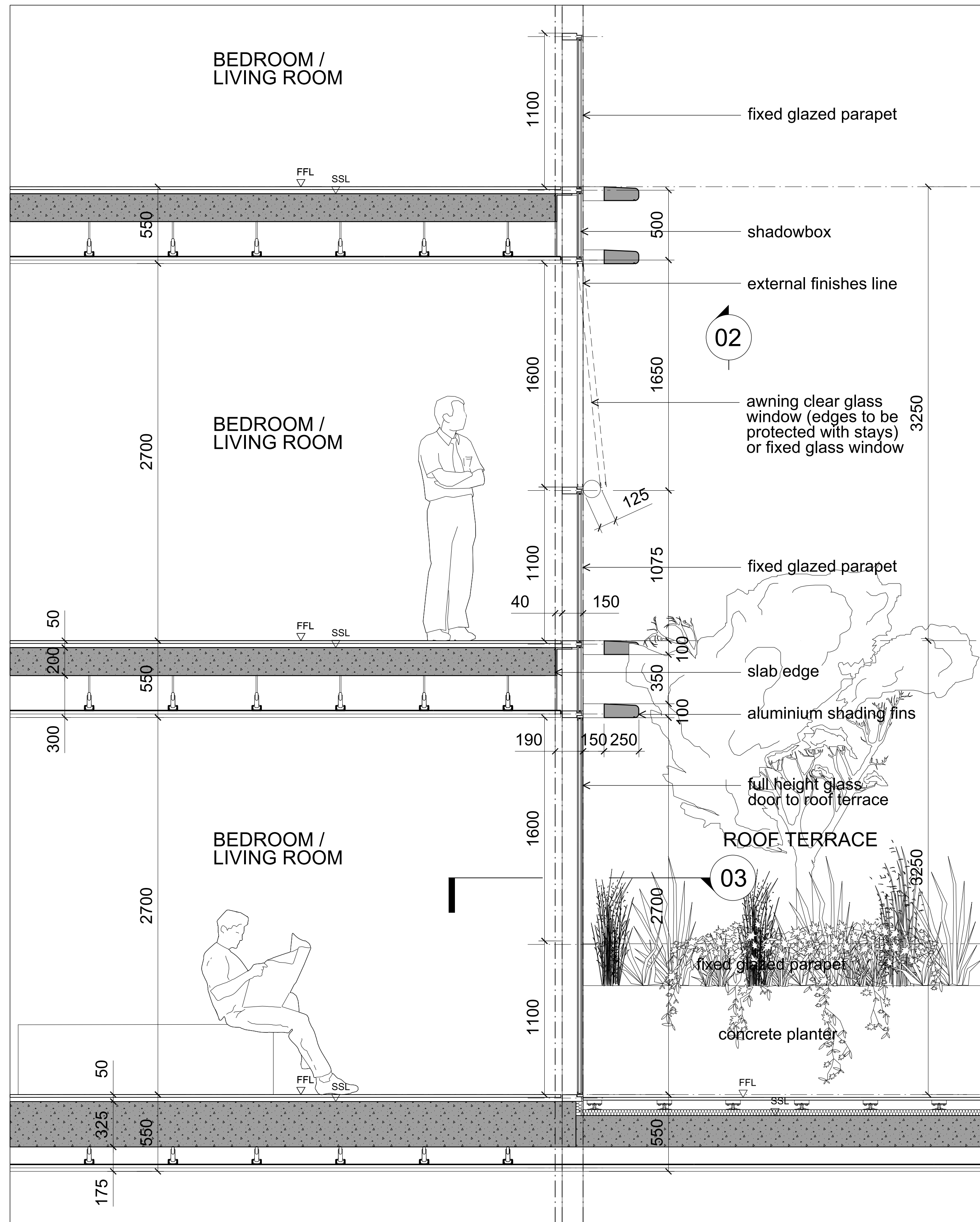
01 Cladding Type F - Typical Top of Building - Section 1:20
