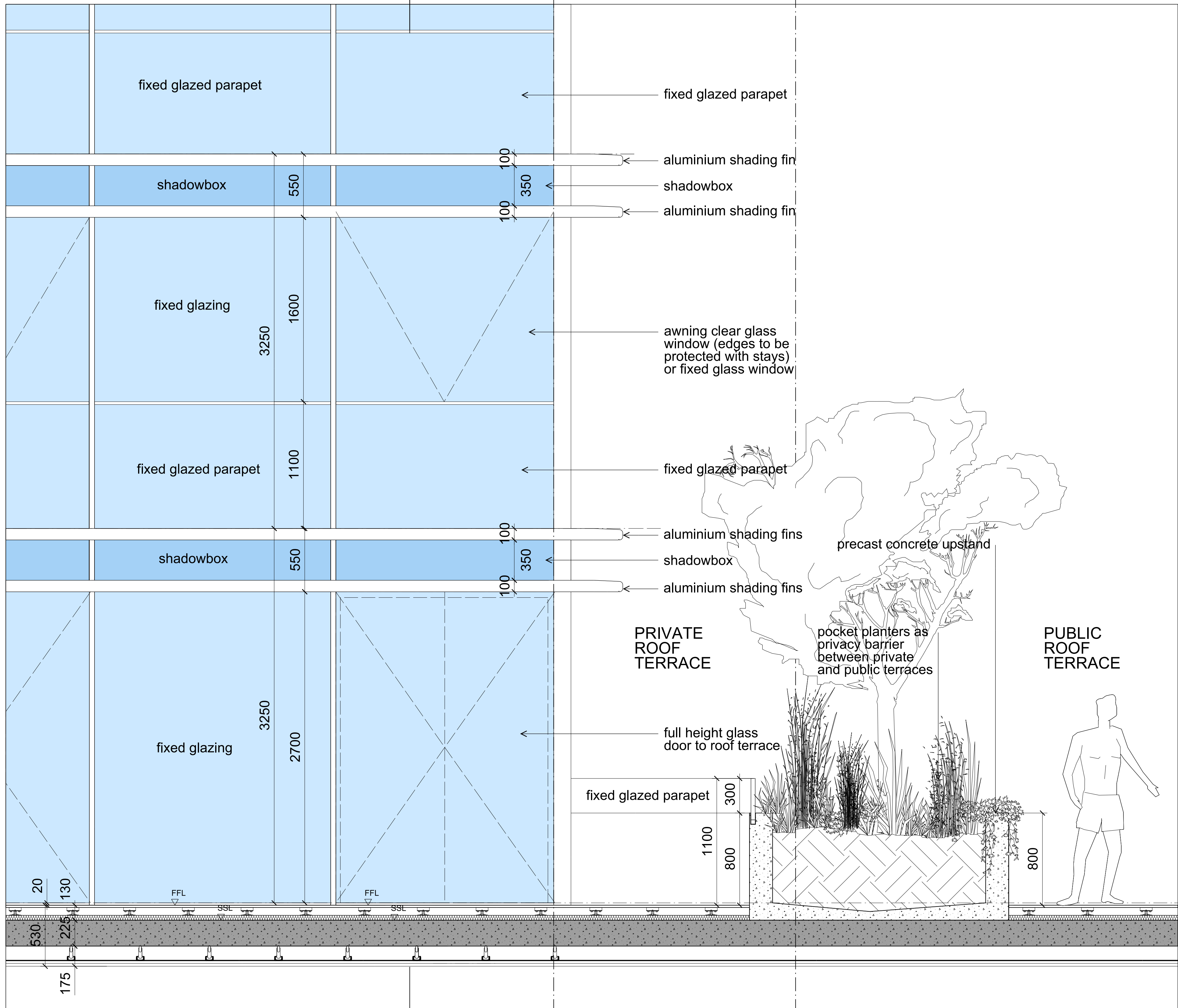
02 Cladding Type F - Typical Top of Building - Elevation 1:20
