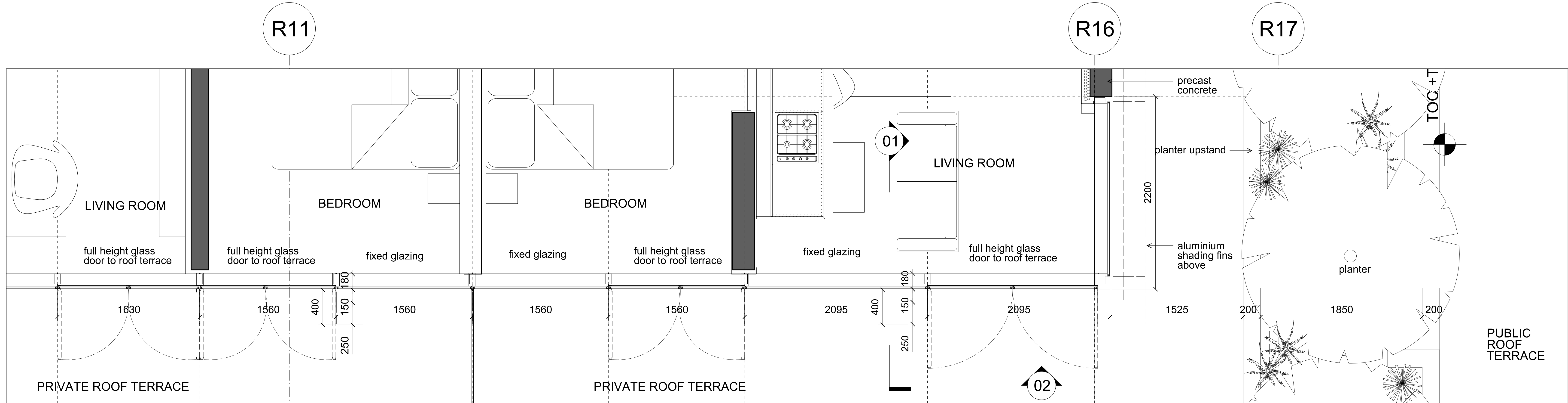
03 Cladding Type F - Typical Top of Building - Plan L16 1:20
