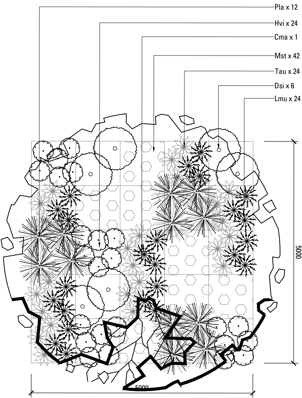
01 LOW LEVEL GROUNDCOVER MATRIX (G1) - 5m x 5m SCALE 1:50
