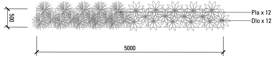
04 PLANTING MATRIX - NATIVE GRASS STREET VERGE (P1) - 5m x 0.5m SCALE 1:50
