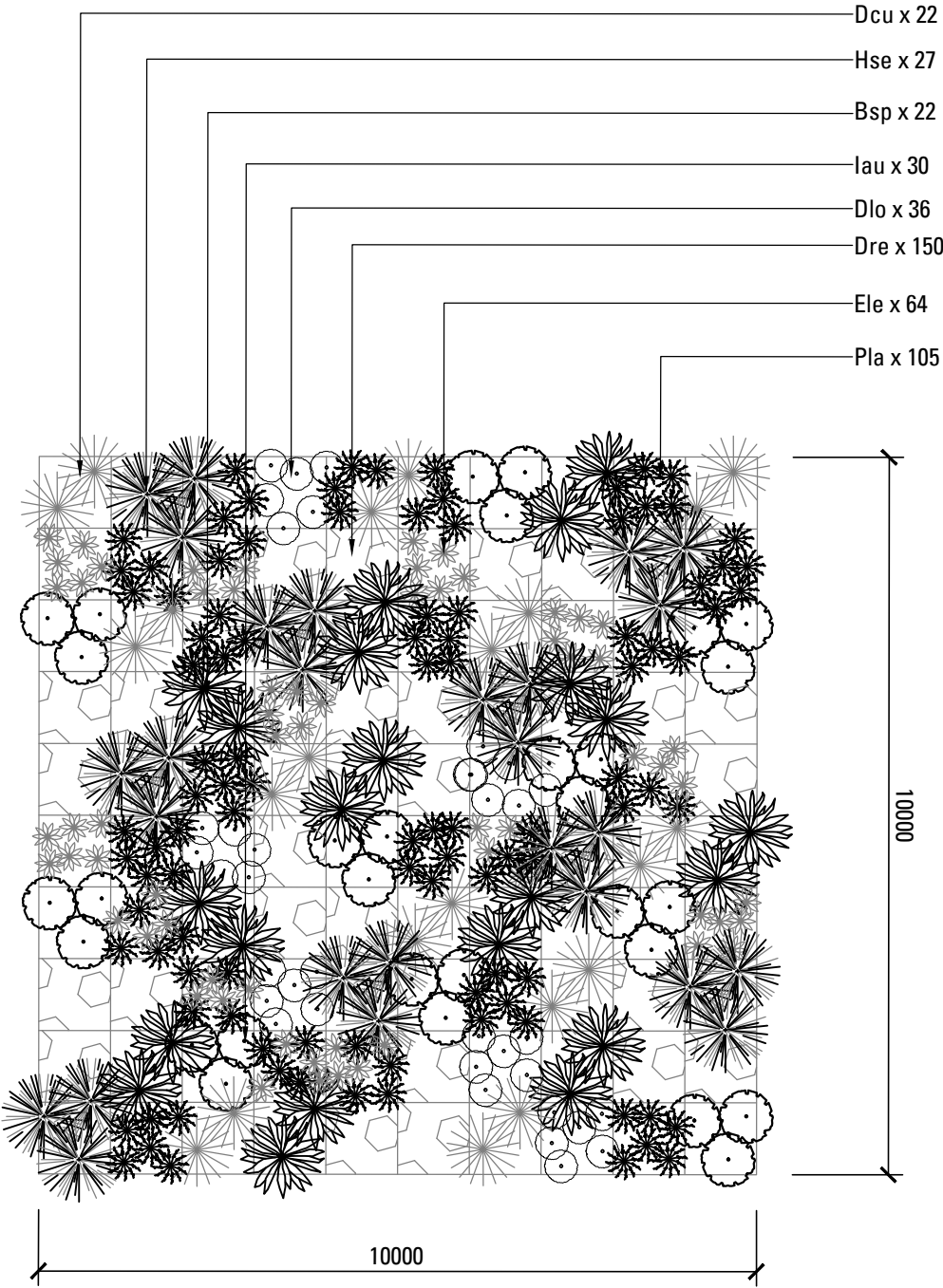
02 NATIVE GRASSES & SHRUBS MATRIX (G2) - 10m x 10m SCALE 1:50
