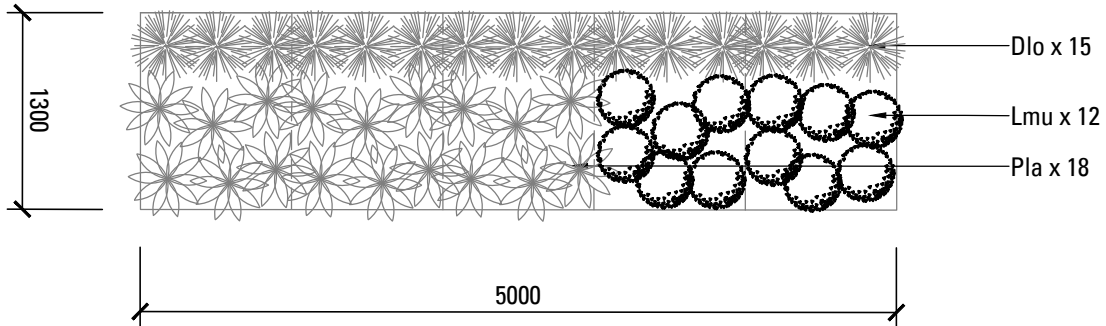
03 PLANTING MATRIX - NATIVE GRASS STREET VERGE (P2) - 5m x 1.3m SCALE 1:50
