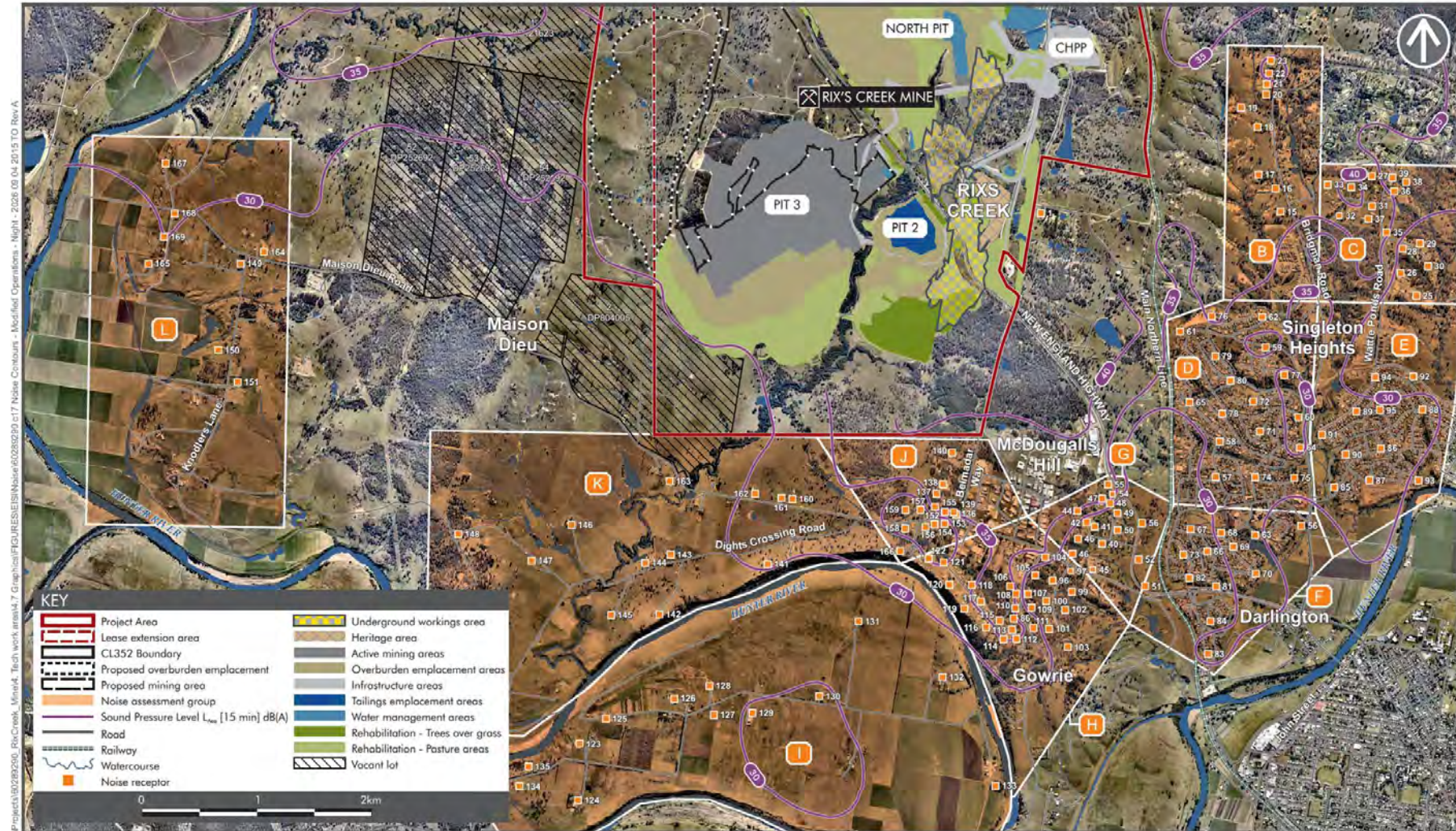
90TH PERCENTILE NOISE CONTOURS - MODIFIED OPERATIONS SCENARIO - NIGHT PERIOD - YEAR 2026 - SOUTH Rix's Creek Continuation of Mining Environmental Impact Statement
