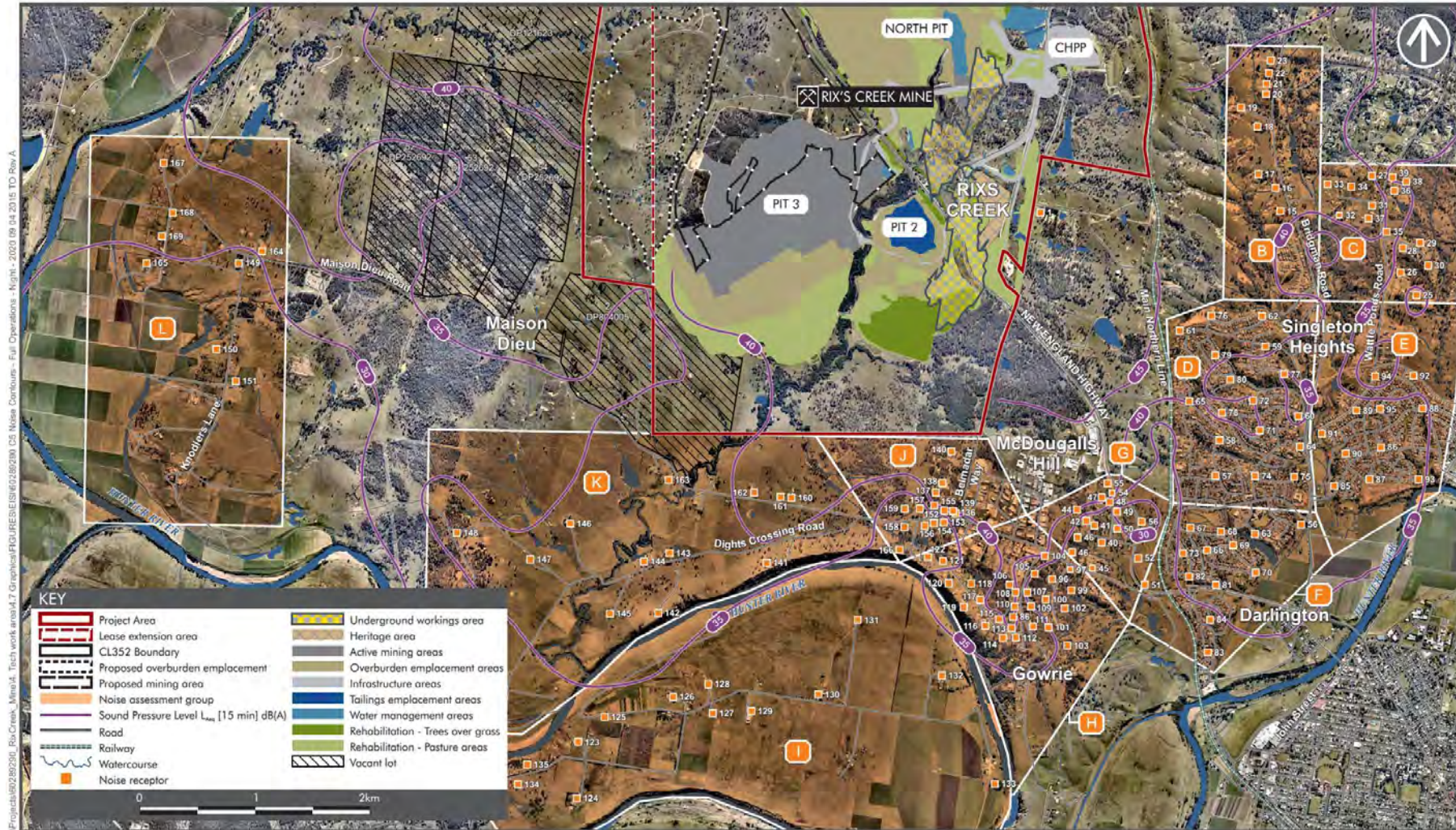
90TH PERCENTILE NOISE CONTOURS - FULL OPERATIONS SCENARIO - NIGHT PERIOD - YEAR 2020 - SOUTH Rix's Creek Continuation of Mining Environmental Impact Statement
