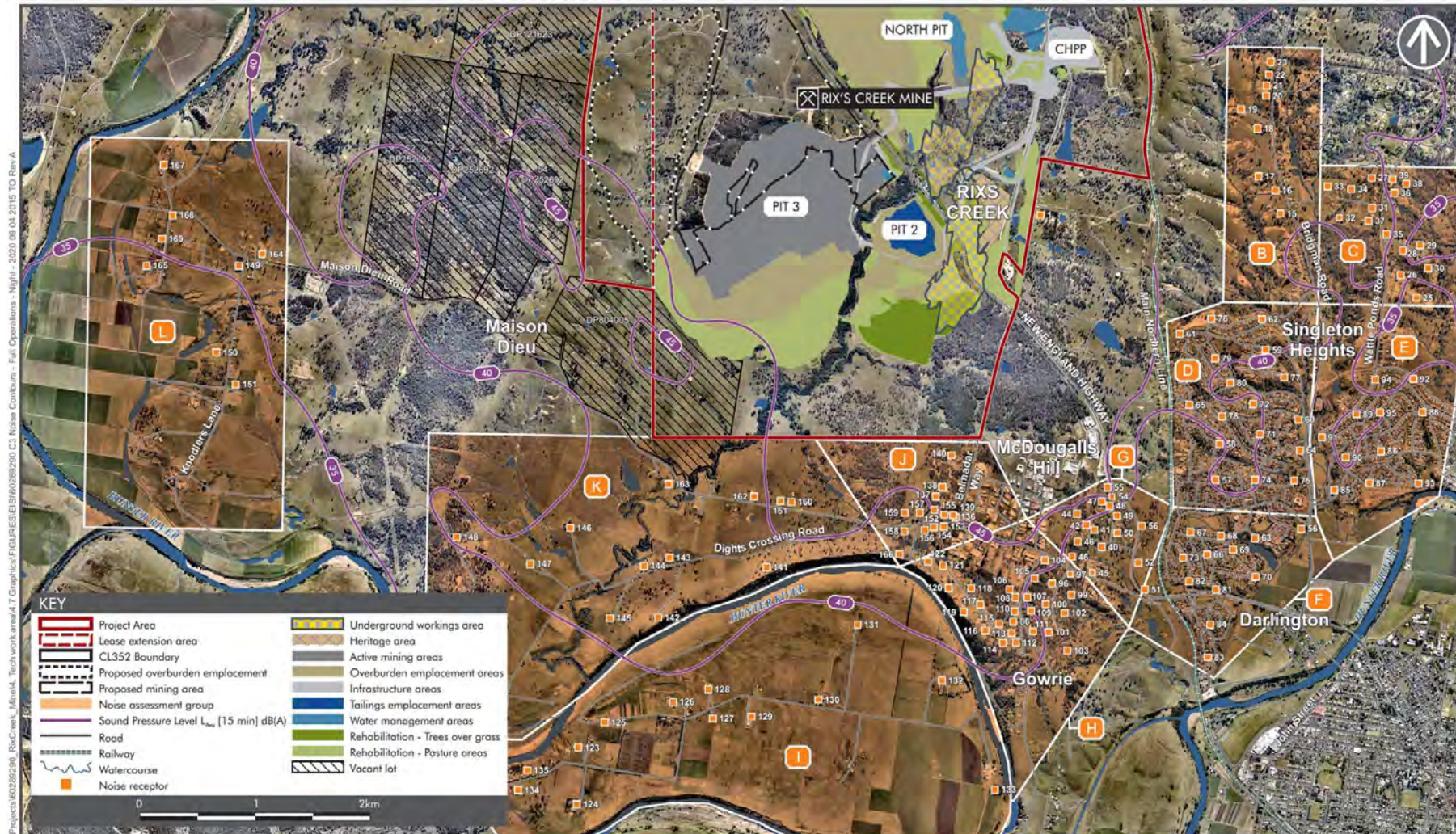
90TH PERCENTILE NOISE CONTOURS - FULL OPERATIONS SCENARIO - NIGHT PERIOD - YEAR 2017 - SOUTH Rix's Creek Continuation of Mining Environmental Impact Statement
