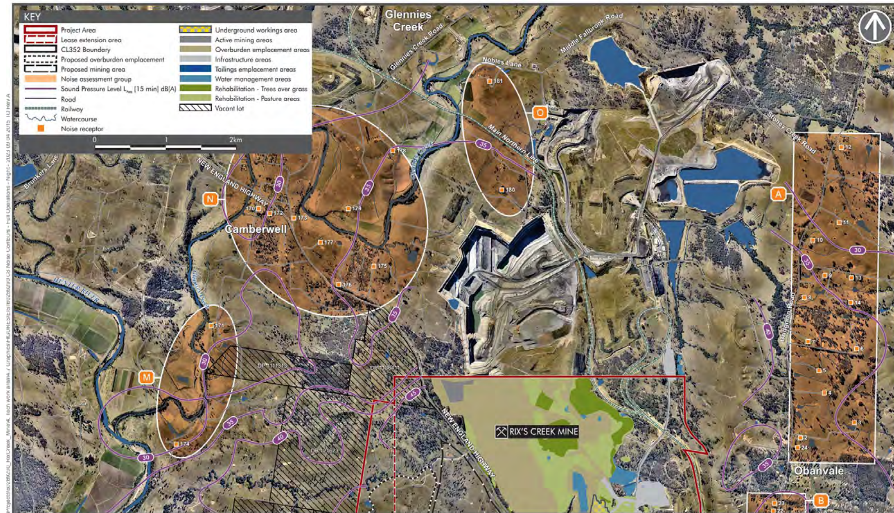
90TH PERCENTILE NOISE CONTOURS - FULL OPERATIONS SCENARIO - NIGHT PERIOD - YEAR 2023 - NORTH Rix's Creek Continuation of Mining Environmental Impact Statement
