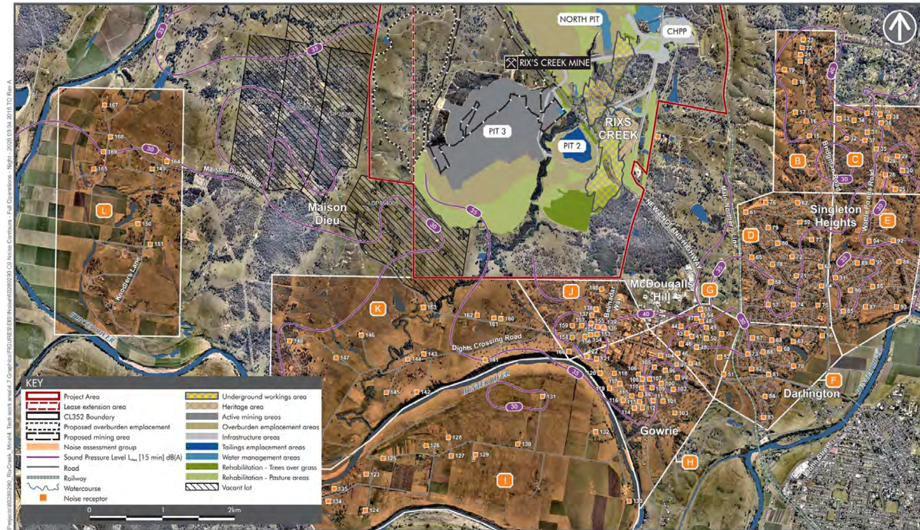
90TH PERCENTILE NOISE CONTOURS - FULL OPERATIONS SCENARIO - NIGHT PERIOD - YEAR 2026 - SOUTH Rix's Creek Continuation of Mining Environmental Impact Statement
