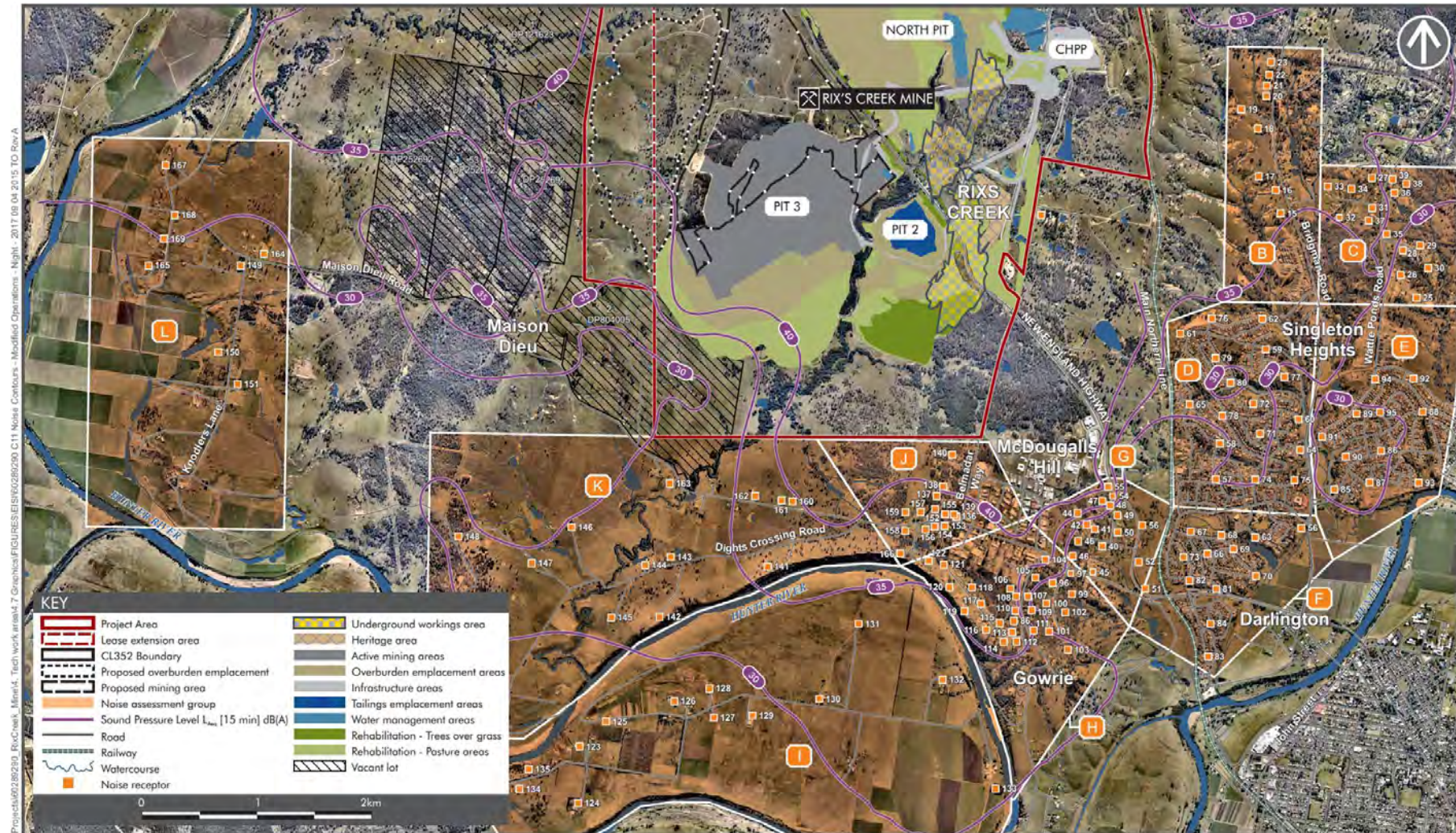
90TH PERCENTILE NOISE CONTOURS - MODIFIED OPERATIONS SCENARIO - NIGHT PERIOD - YEAR 2017 - SOUTH Rix's Creek Continuation of Mining Environmental Impact Statement
