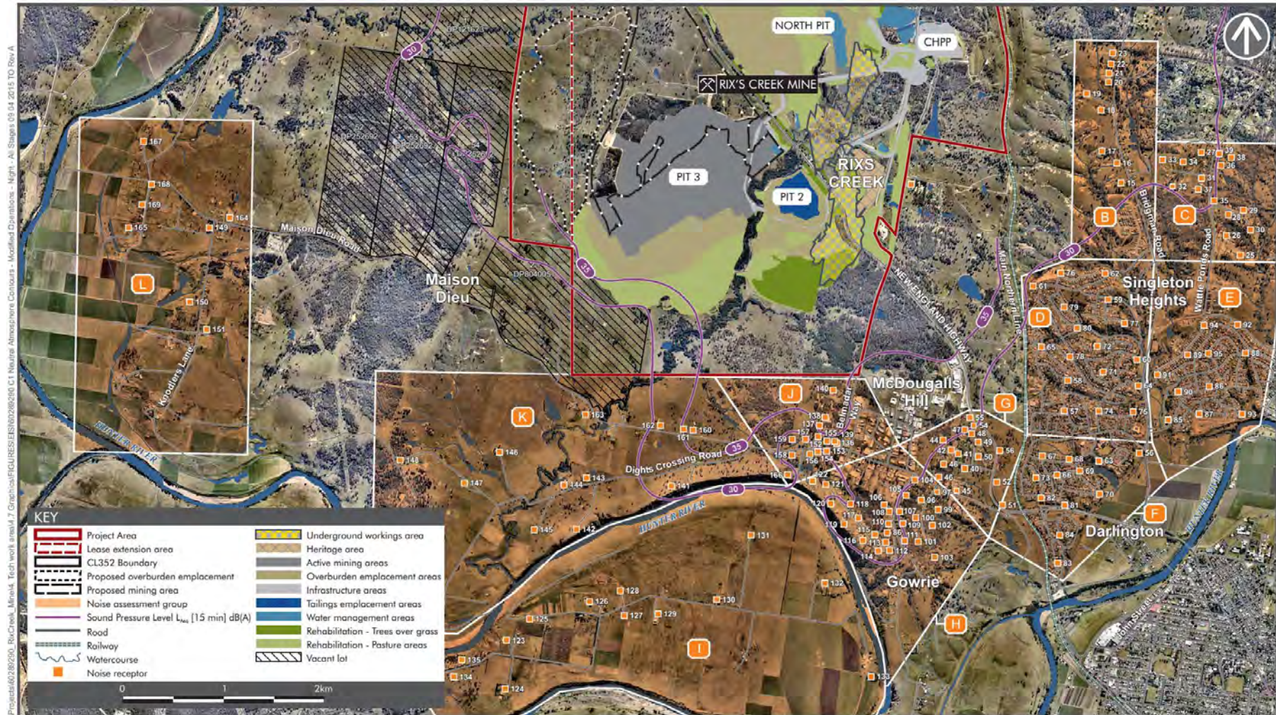
NEUTRAL ATMOSPHERE NOISE CONTOURS - FULL OPERATIONS SCENARIO - NIGHT PERIOD - MAXIMUM ENVELOPE - ALL STAGES - SOUTH
