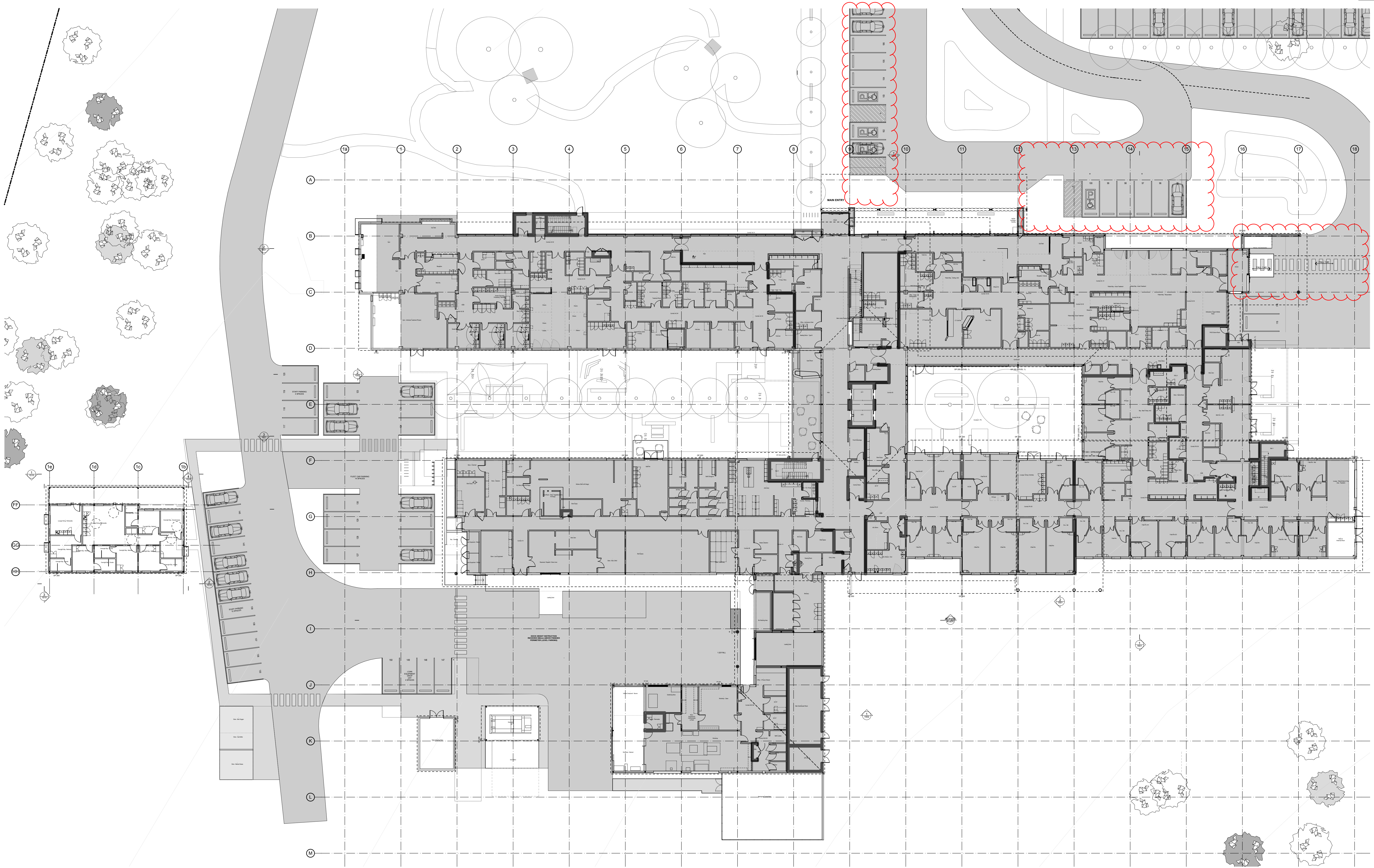
1 PLAN GROUND FLOOR
