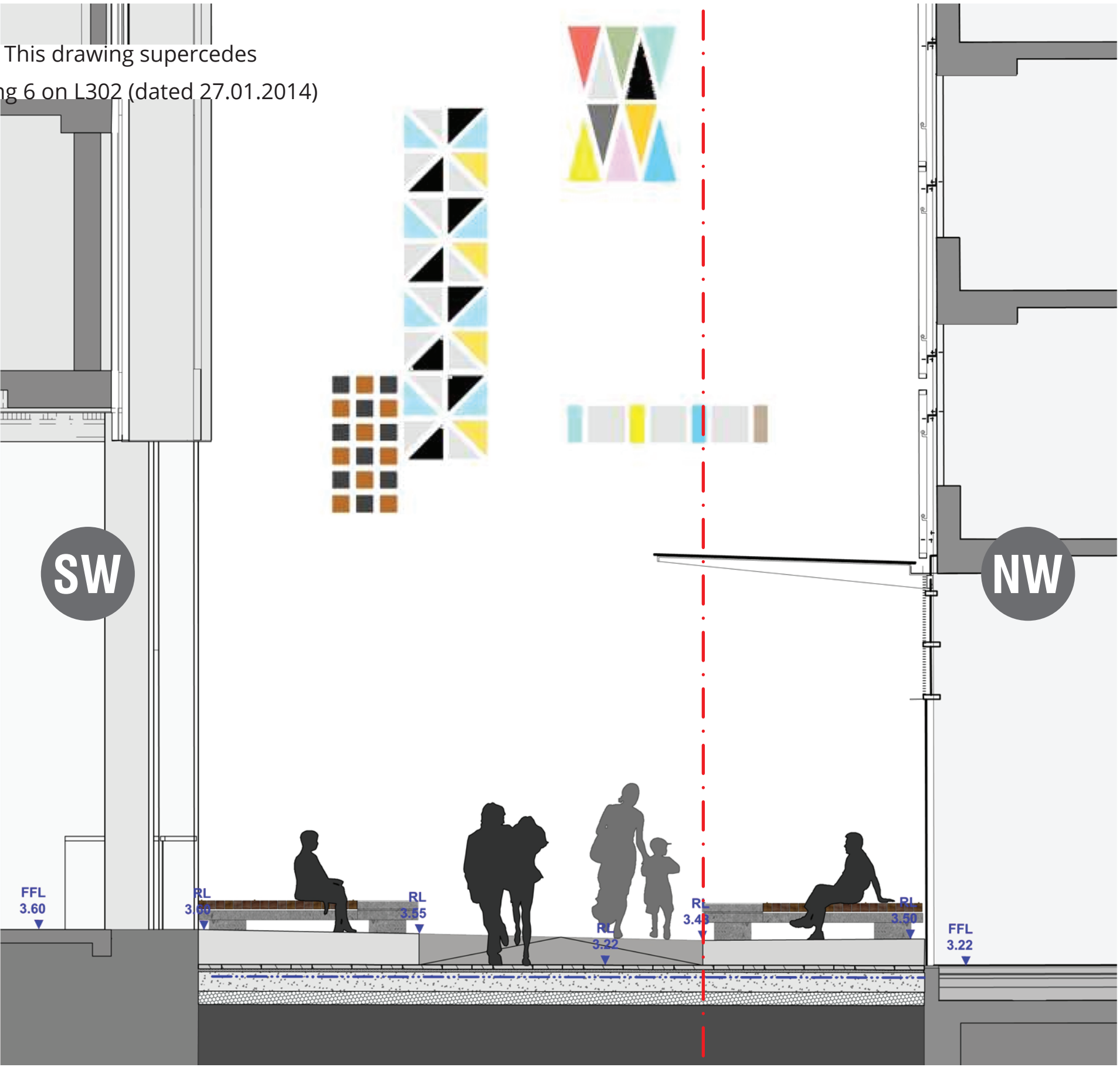
SECTION 1 (ZONE 1) - DAY VIEW
