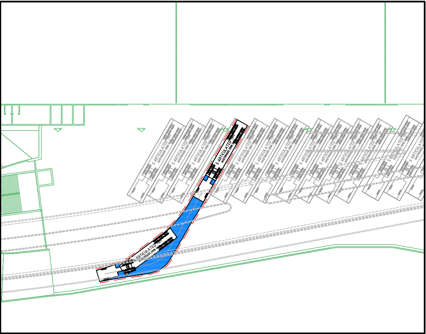
AUSTROADS 2006 19.0m SEMI - 11 IN @ 5km/hr 1 : 500
