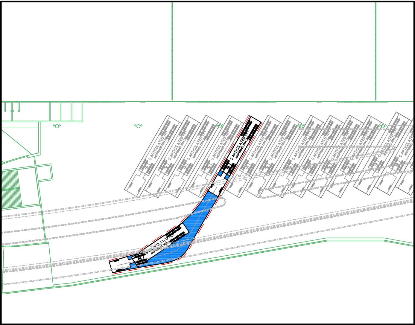
AUSTROADS 2006 19.0m SEMI - 10 IN @ 5km/hr 1 : 500
