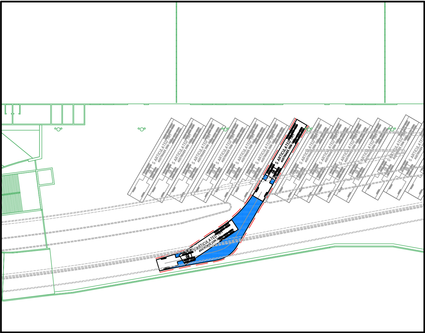
AUSTROADS 2006 19.0m SEMI - 08 IN @ 5km/hr 1 : 500
