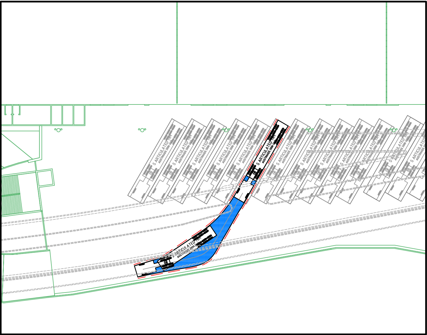
AUSTROADS 2006 19.0m SEMI - 09 IN @ 5km/hr 1 : 500
