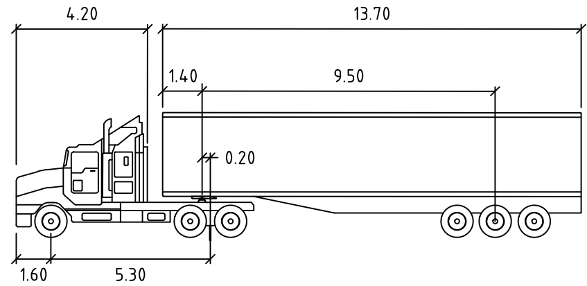
AUSTROADS 2006 19.0m SEMI - 09 OUT @ 5km/hr 1 : 500
