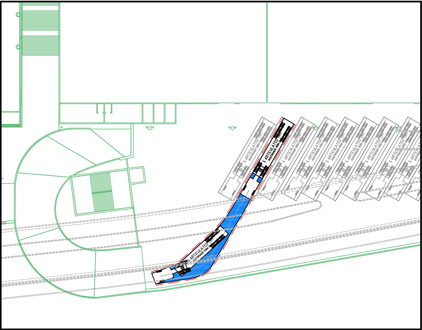
AUSTROADS 2006 19.0m SEMI - 13 IN @ 5km/hr 1 : 500
