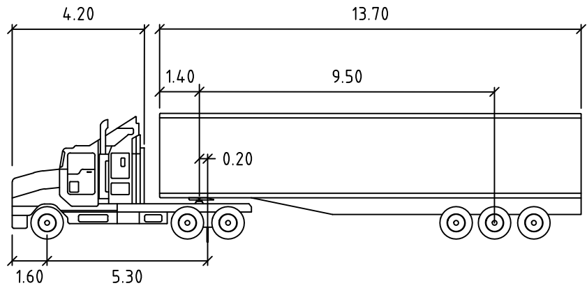
AUSTROADS 2006 19.0m SEMI - 13 OUT @ 5km/hr 1 : 500
