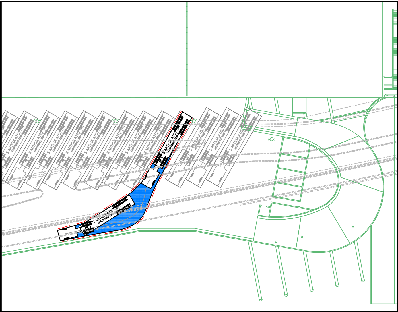
AUSTROADS 2006 19.0m SEMI - 04 IN @ 5km/hr 1 : 500
