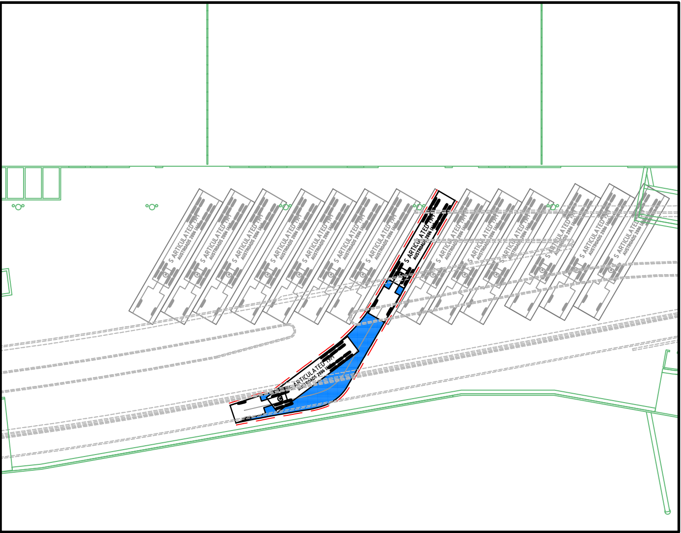
AUSTROADS 2006 19.0m SEMI - 07 IN @ 5km/hr 1 : 500
