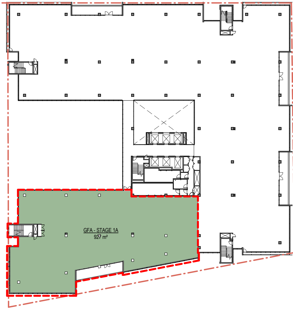
7 Level 6 1: 500
