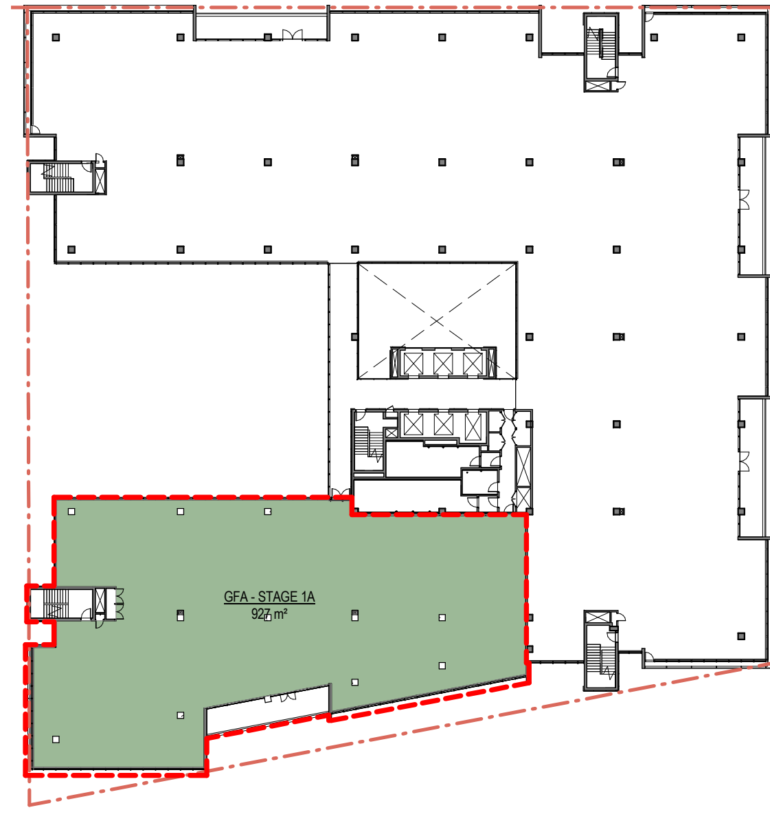
4 Level 3 1: 500
