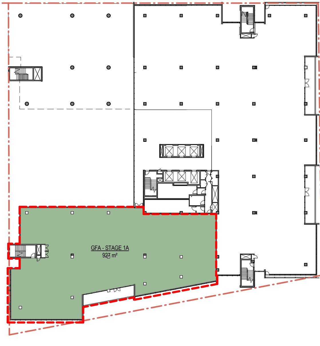
3 Level 2 1: 500
