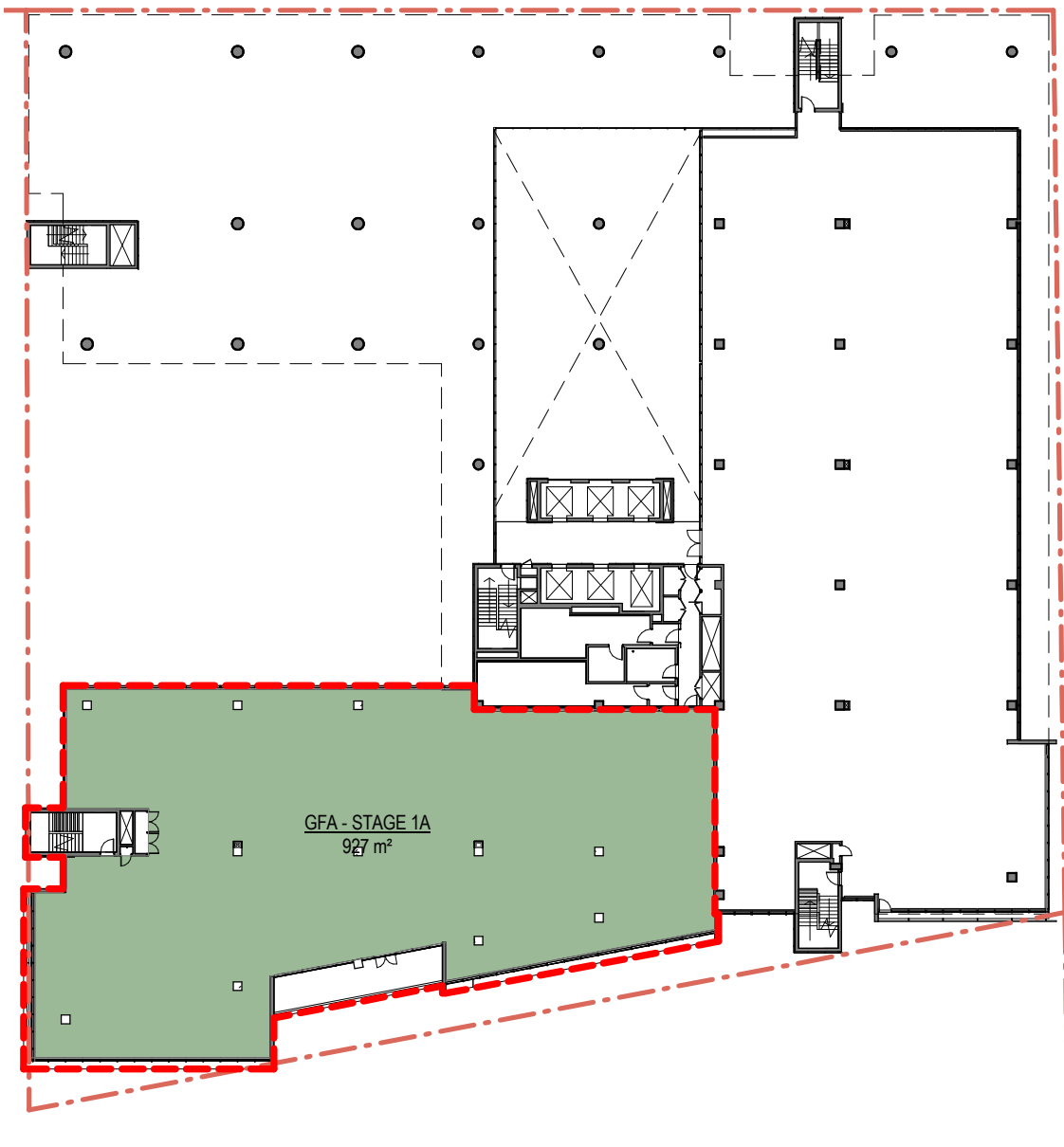
2 Level 1 1: 500
