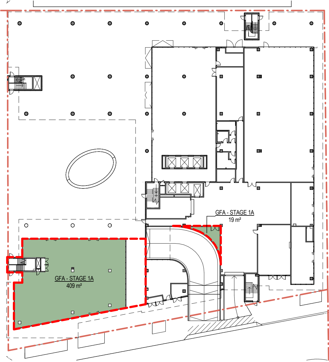
1 Ground Floor 1: 500
