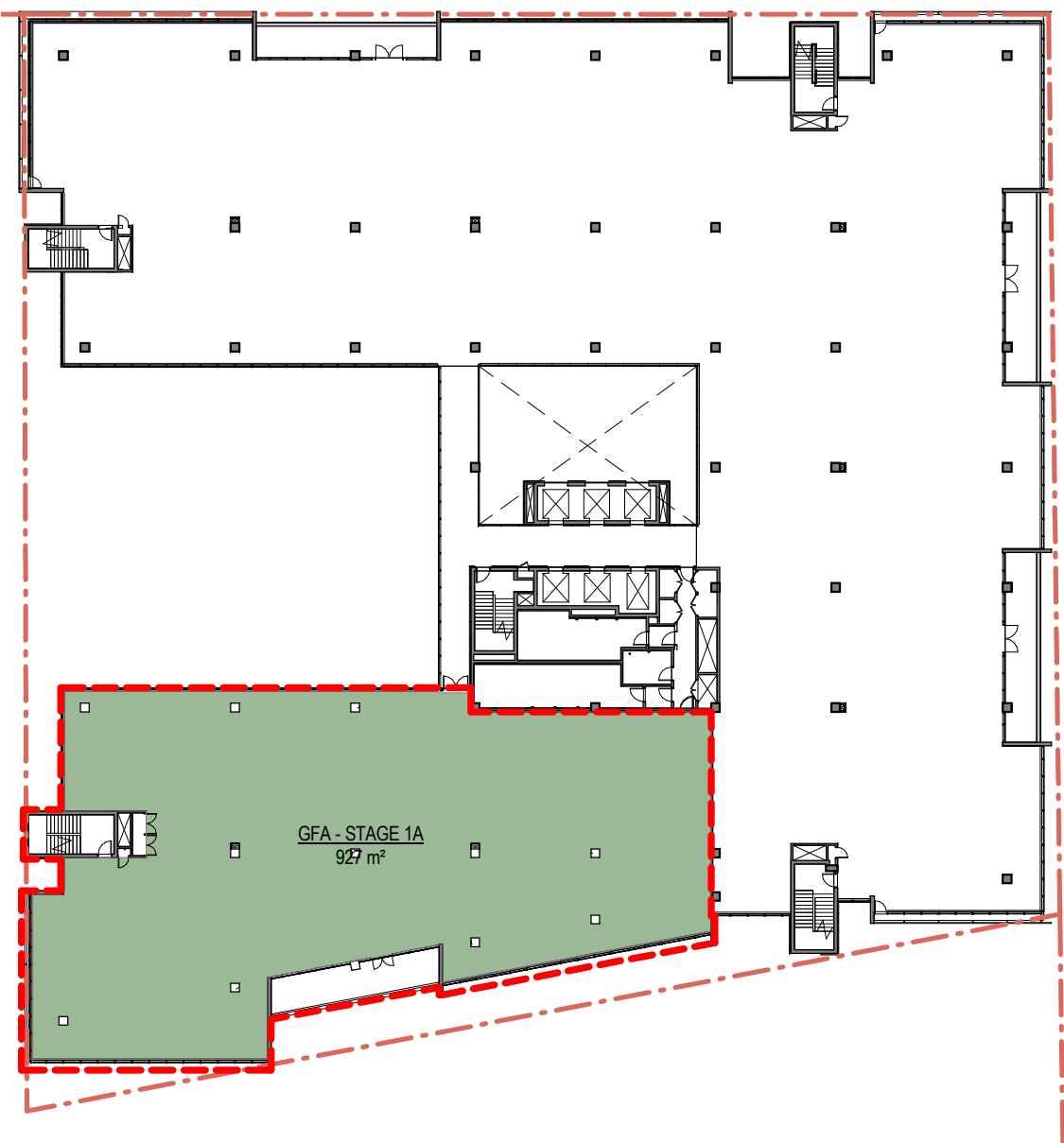
5 Level 4 1: 500
