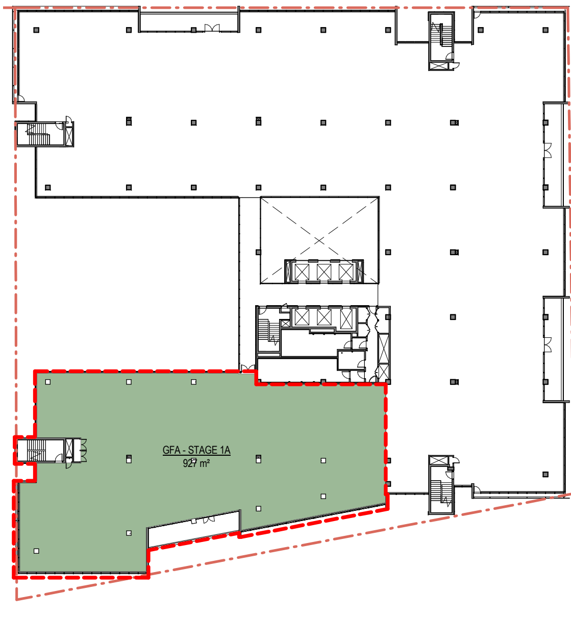
7 Level 6 1: 500
