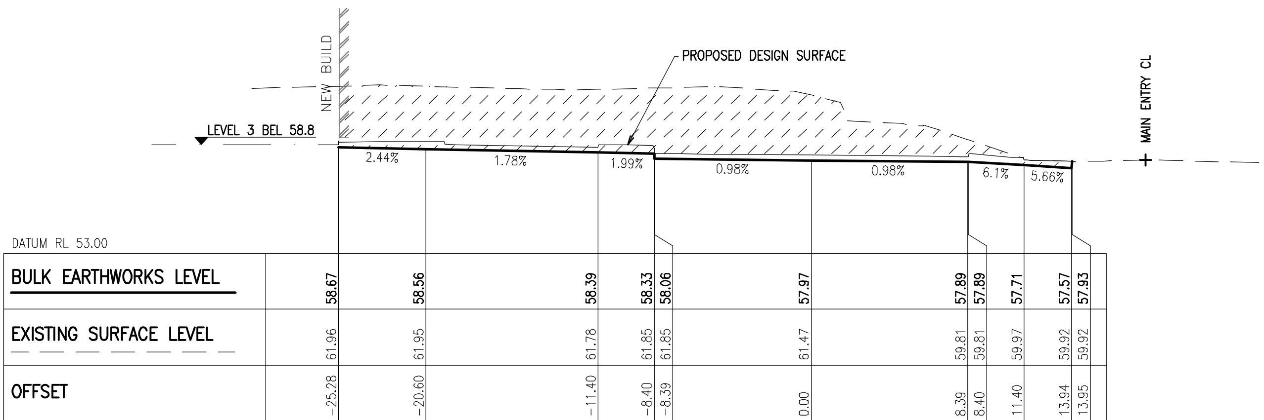
SECTION XS2 SCALE H: 1:200 V: 1:200
