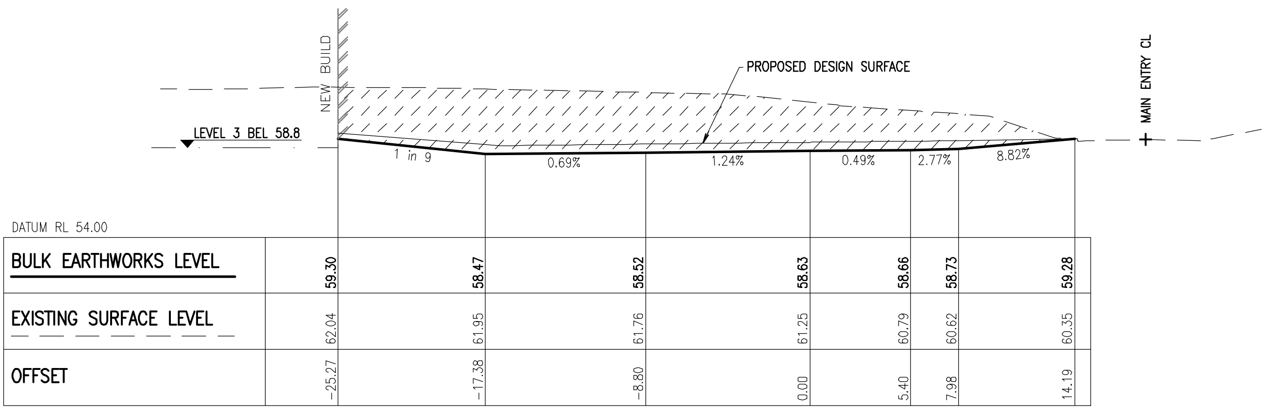
SECTION XS3 SCALE H: 1:200 V: 1:200
