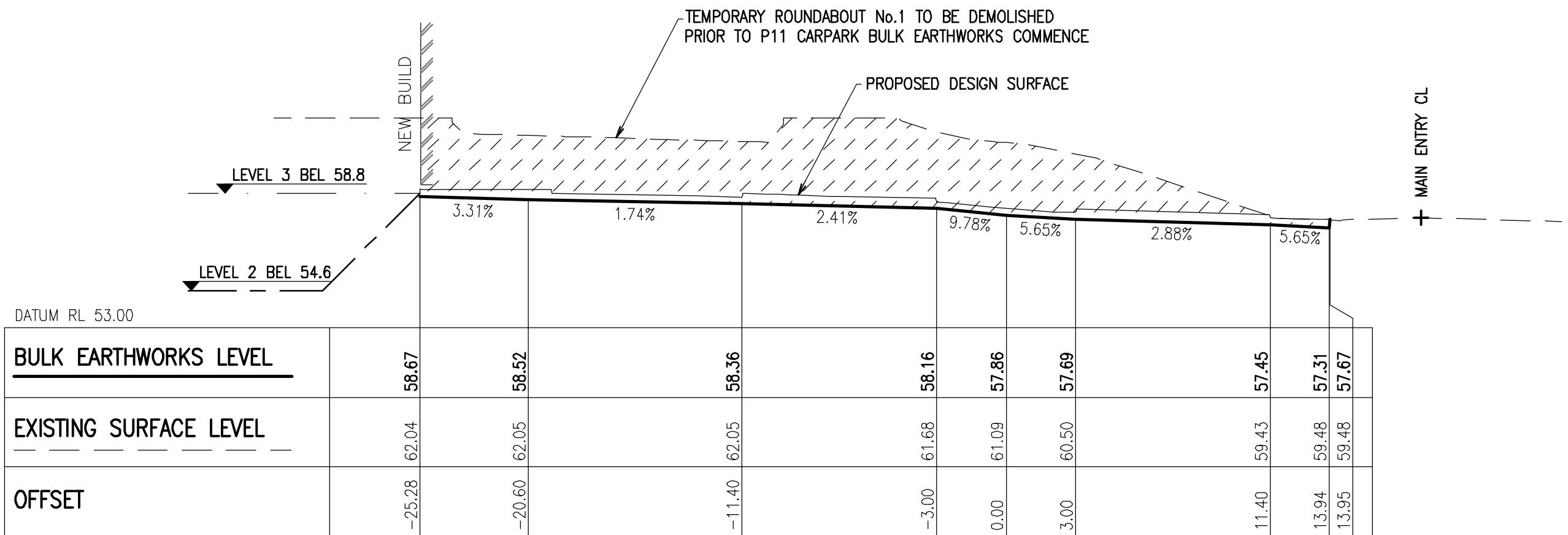
SECTION XS1 SCALE H: 1:200 V: 1:200
