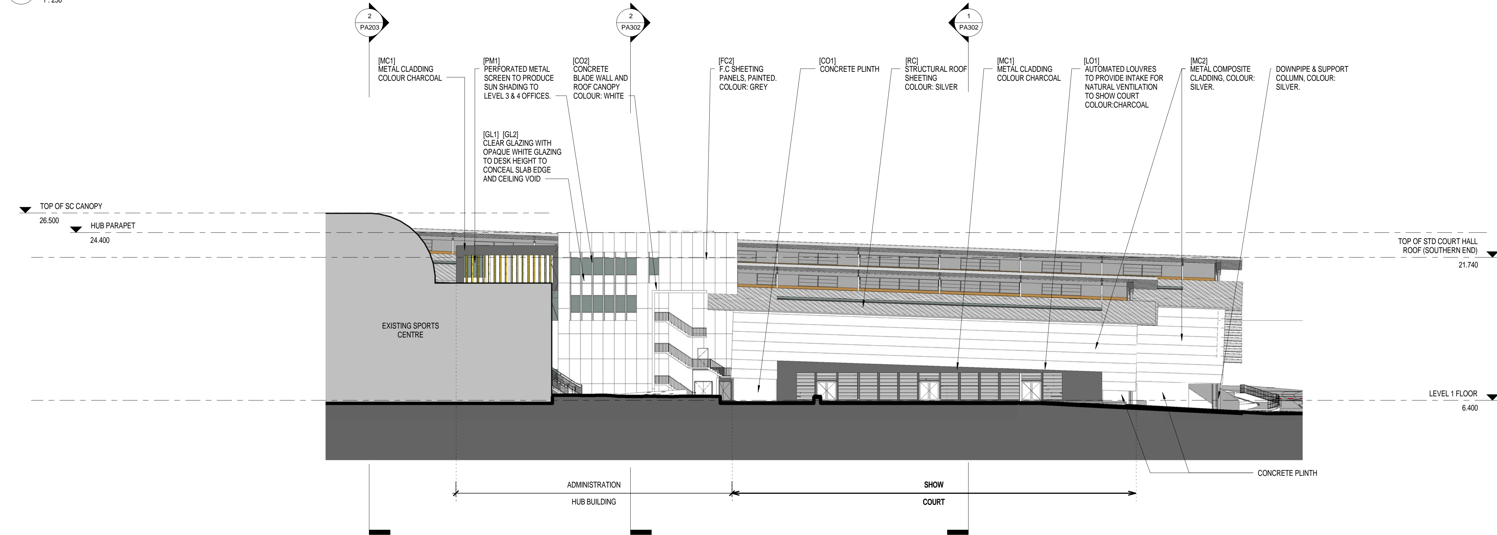
1 South Elevation (Court Halls) 1 : 250
