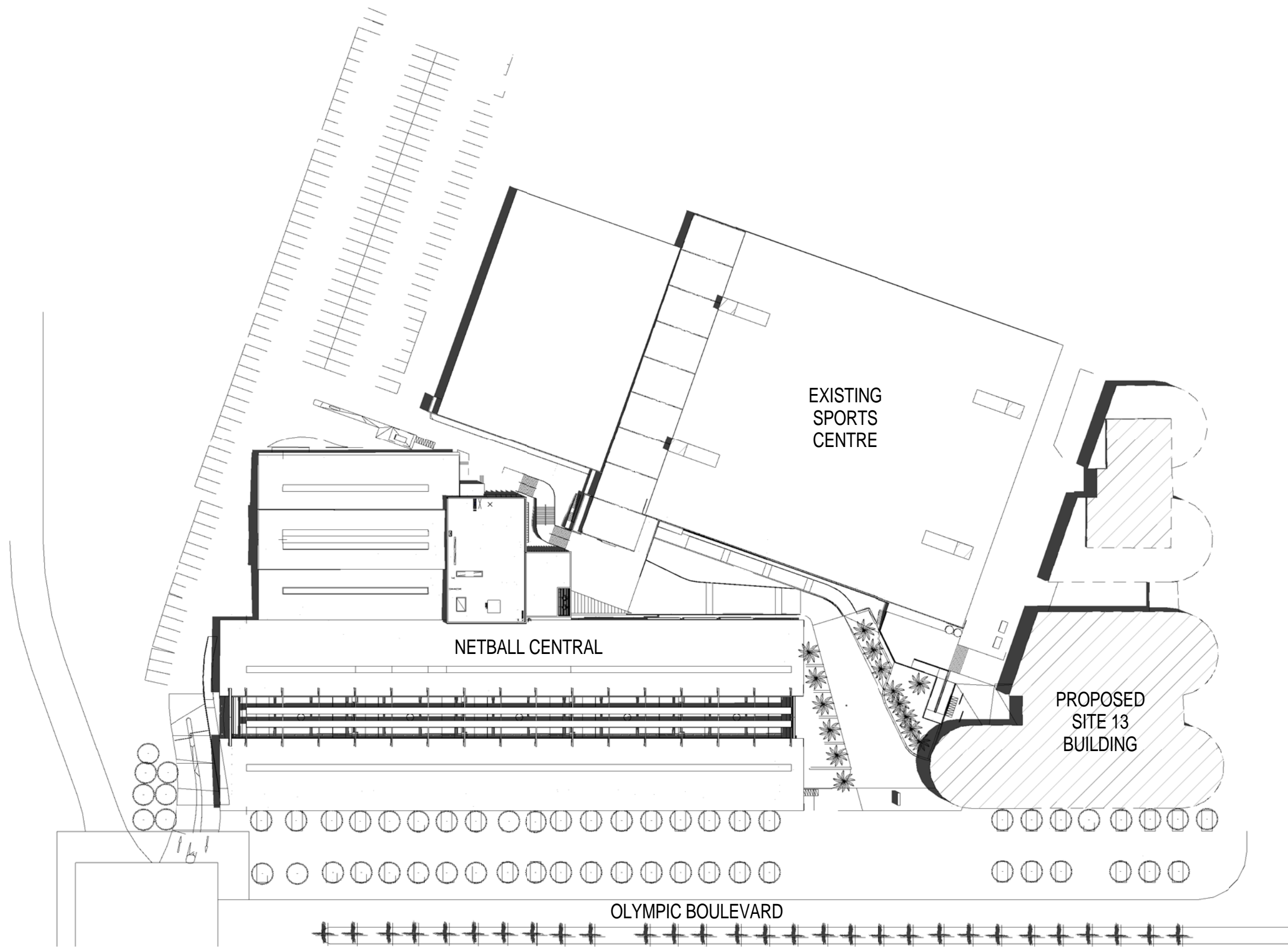
2 Shadow Diagram - 12pm December 21 1:1000
