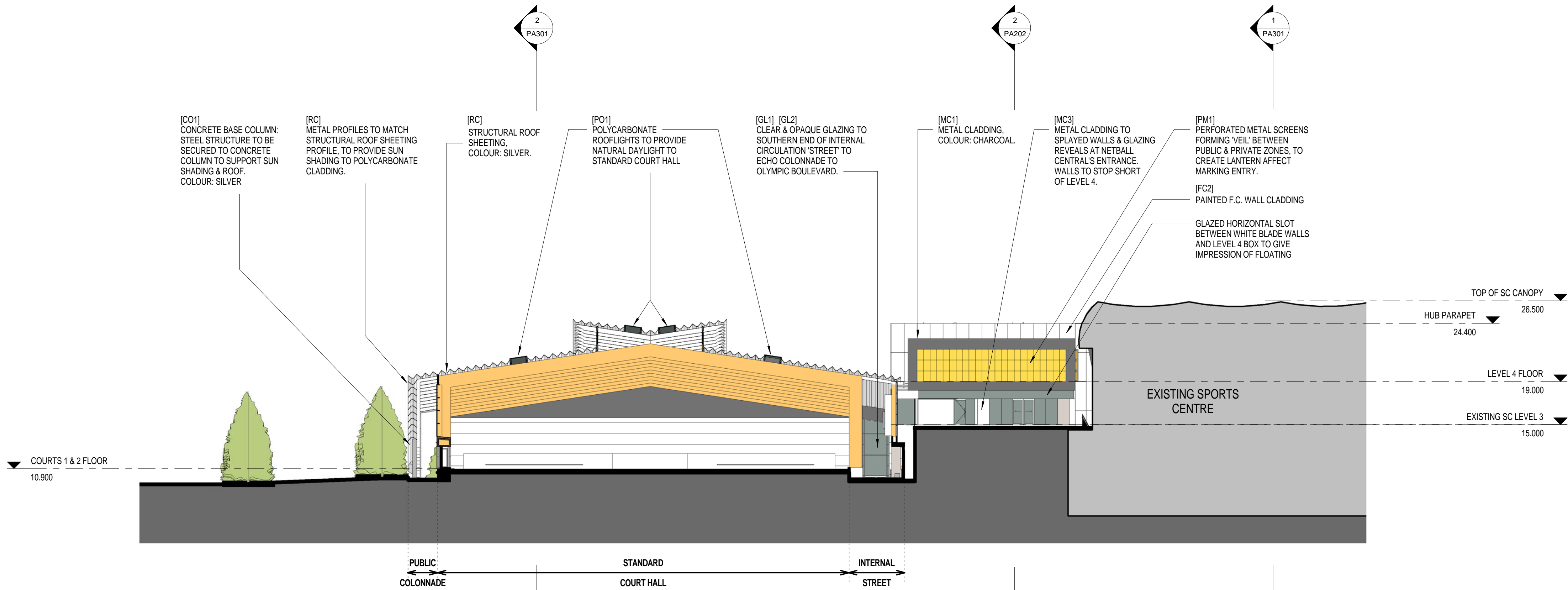
1 Hub North Elevation/ Section CC Through Court 2
