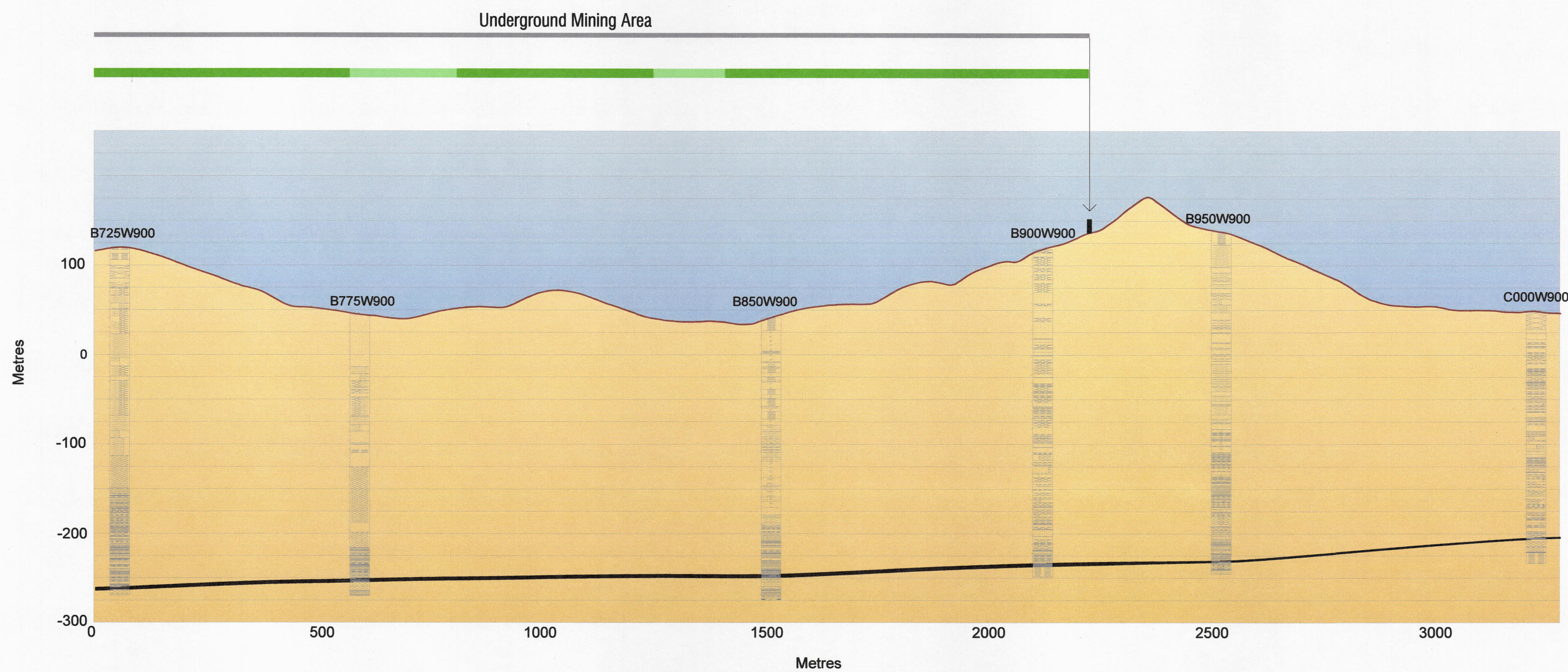
SECTION C - C'
