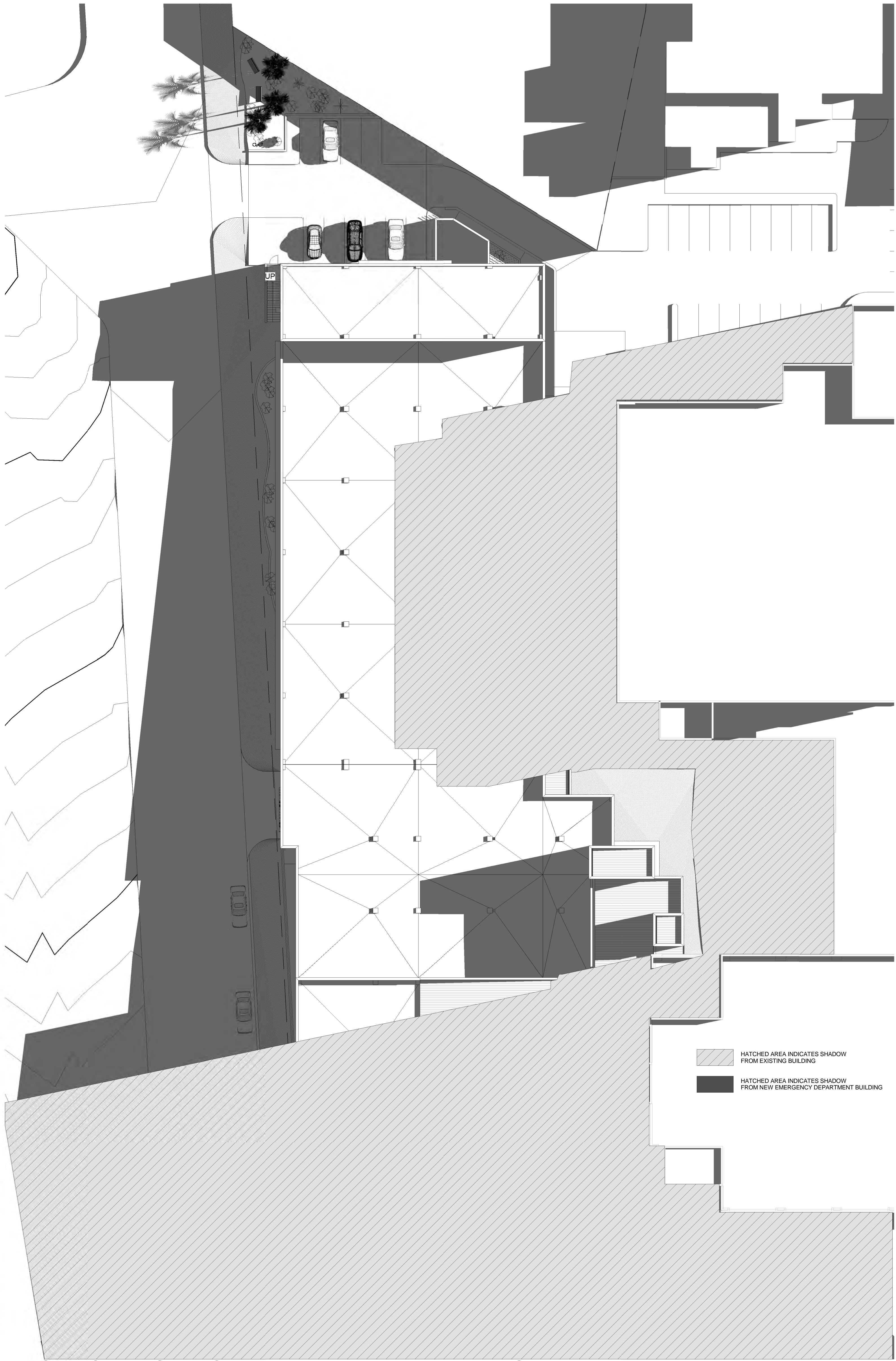
2 SHADOW DIAGRAM ON 21.06.2012 9am ED + EX BUILDING 1 : 250
