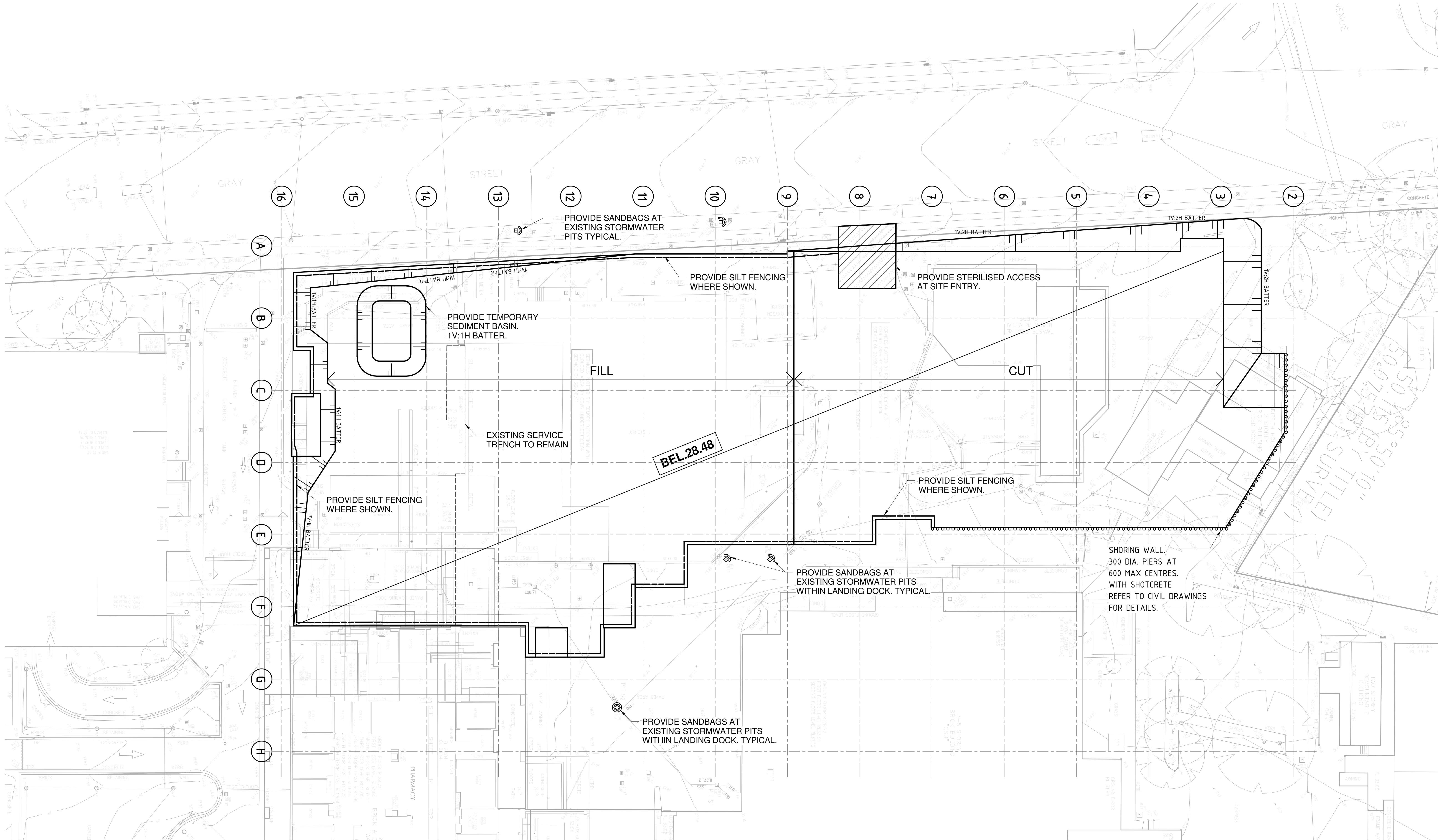
BULK EARTHWORKS PLAN SCALE 1 : 200
