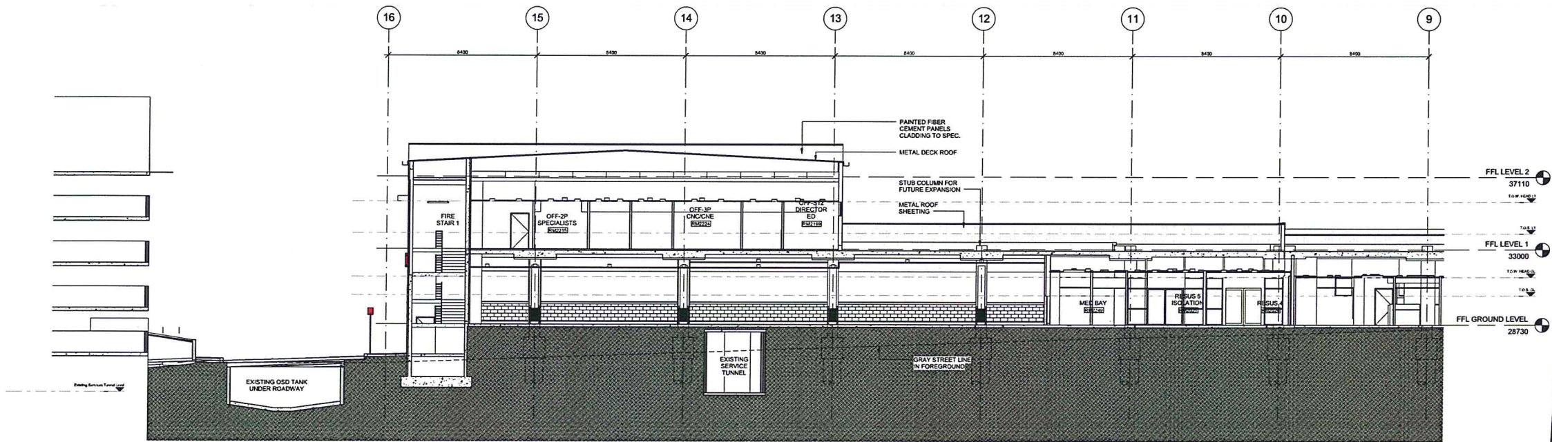
1 SECTION 03 - SOUTH 1:100
