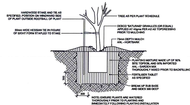
1 TREE PLANTING (75L) TYPICAL SECTION 1:20
