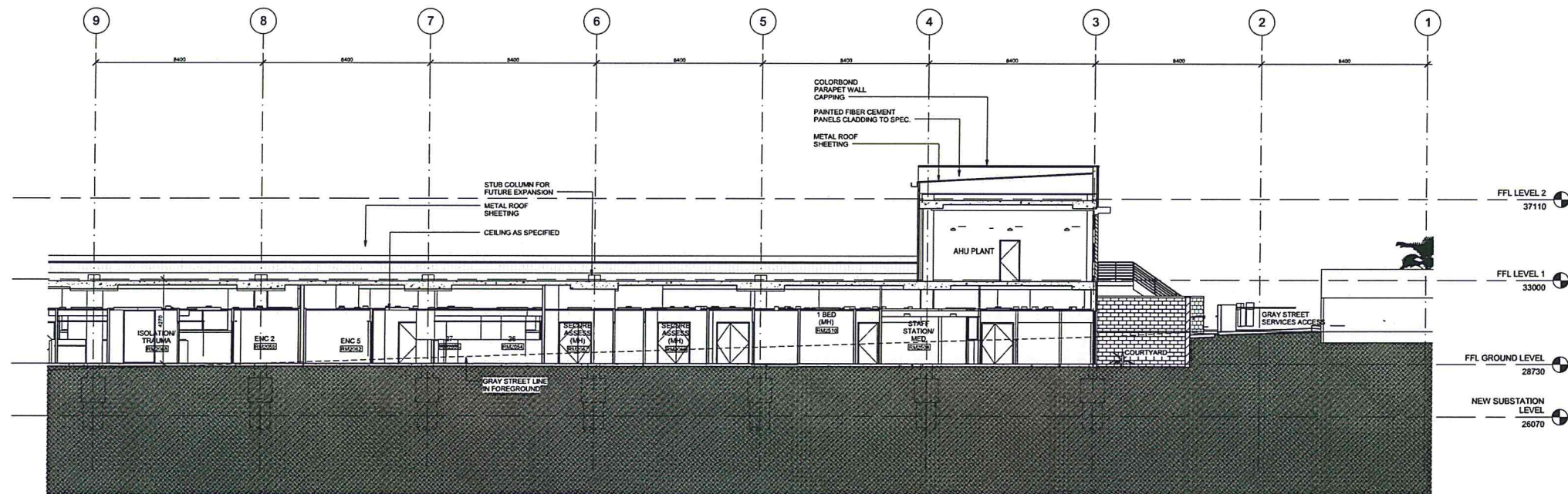
2 SECTION 03 - NORTH 1:100
