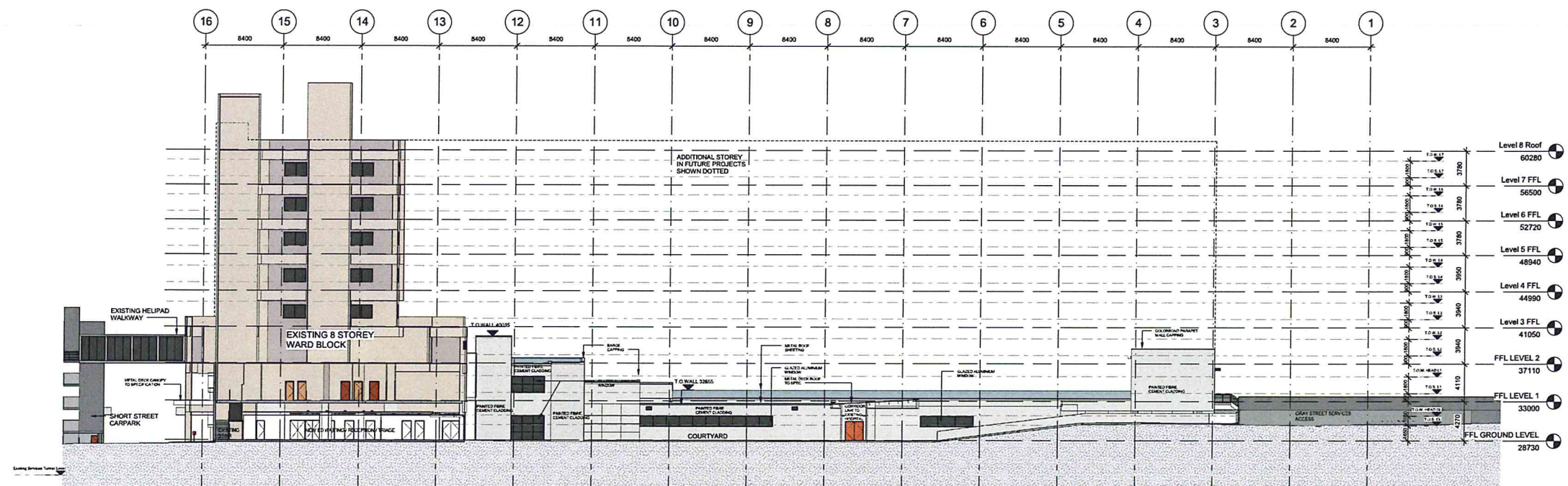
EAST ELEVATION/SECTION FROM EXISTING LOADING DOCK
