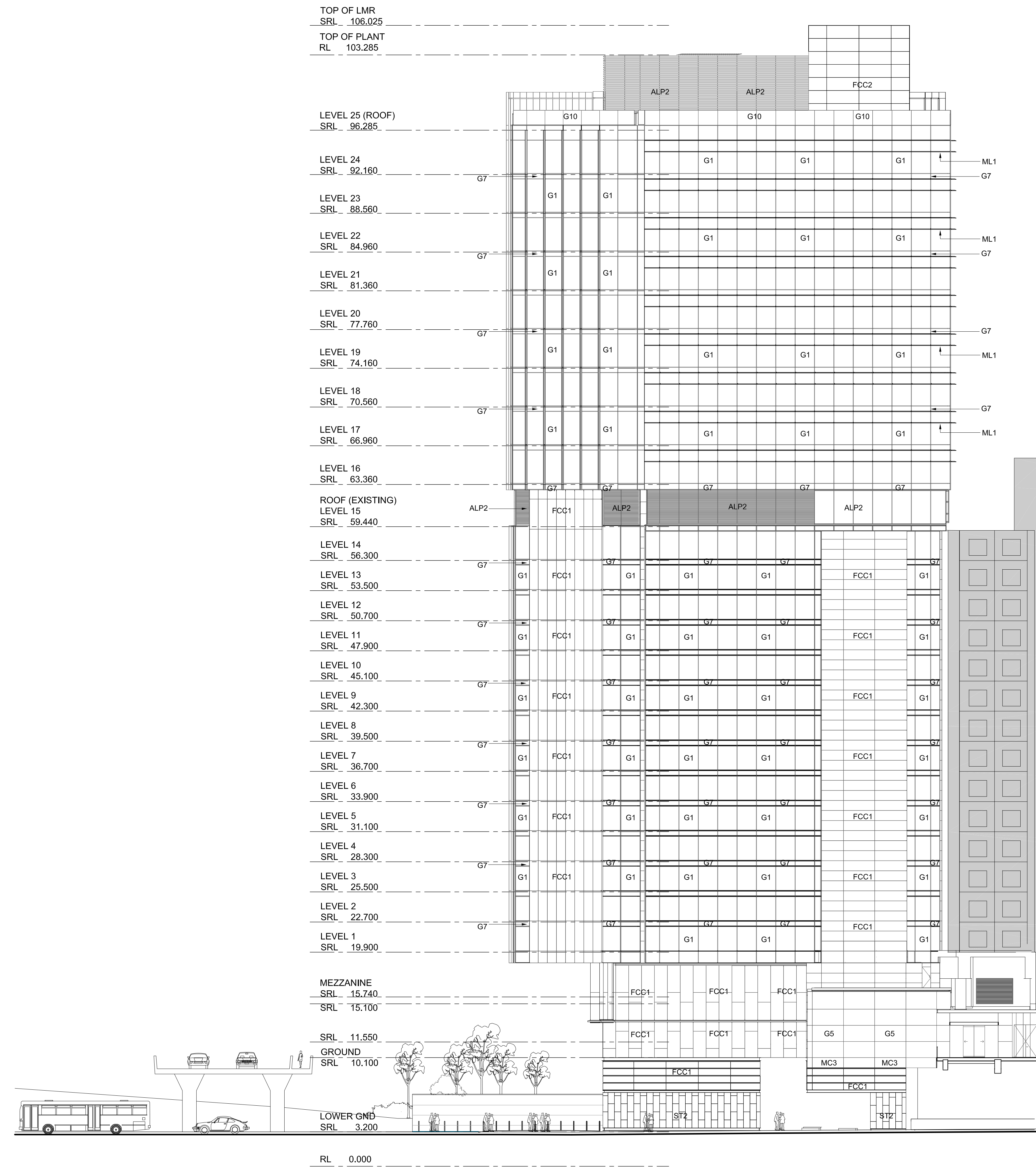
02 SLIP ST ELEVATION
