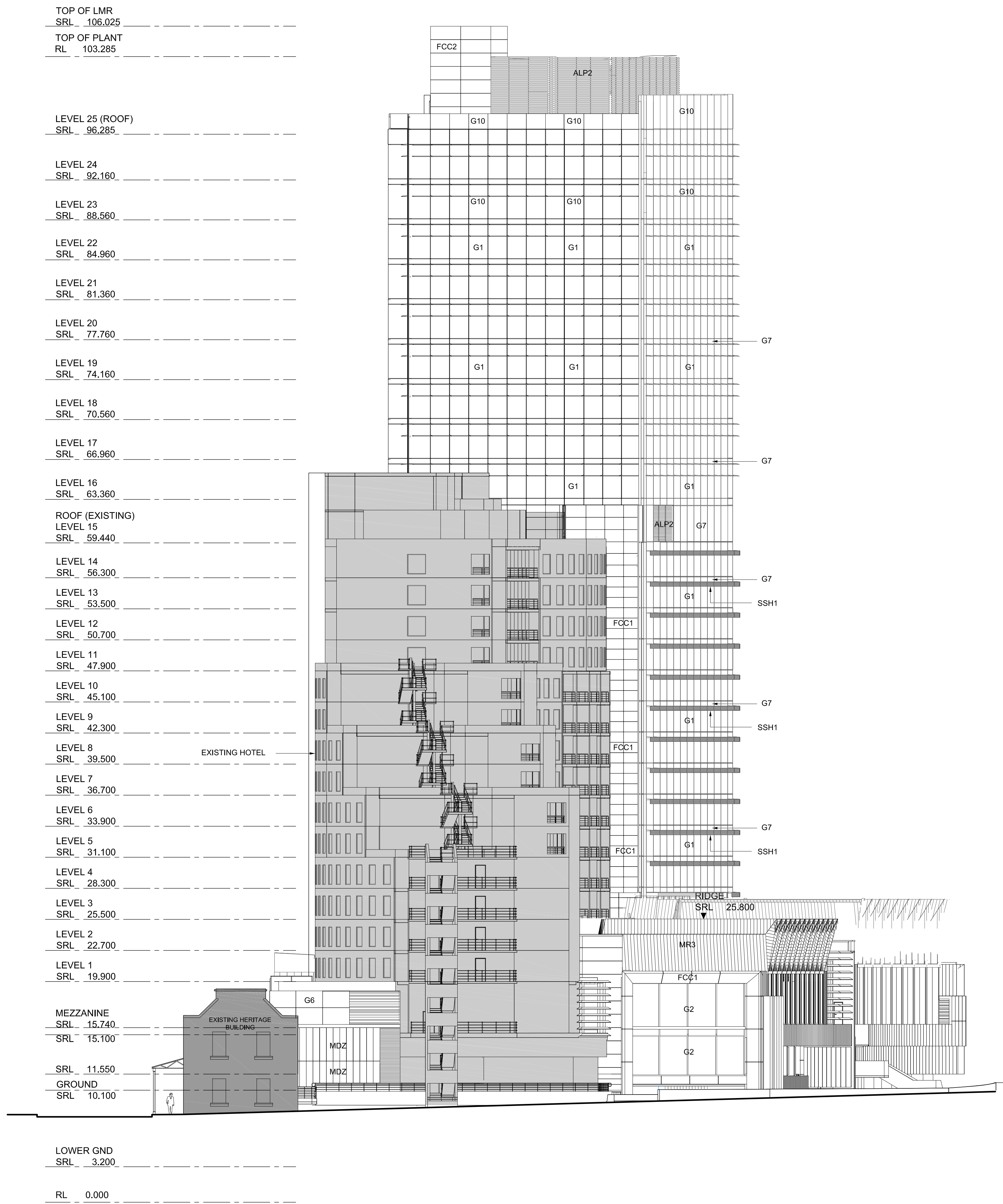
01 NORTH ELEVATION
