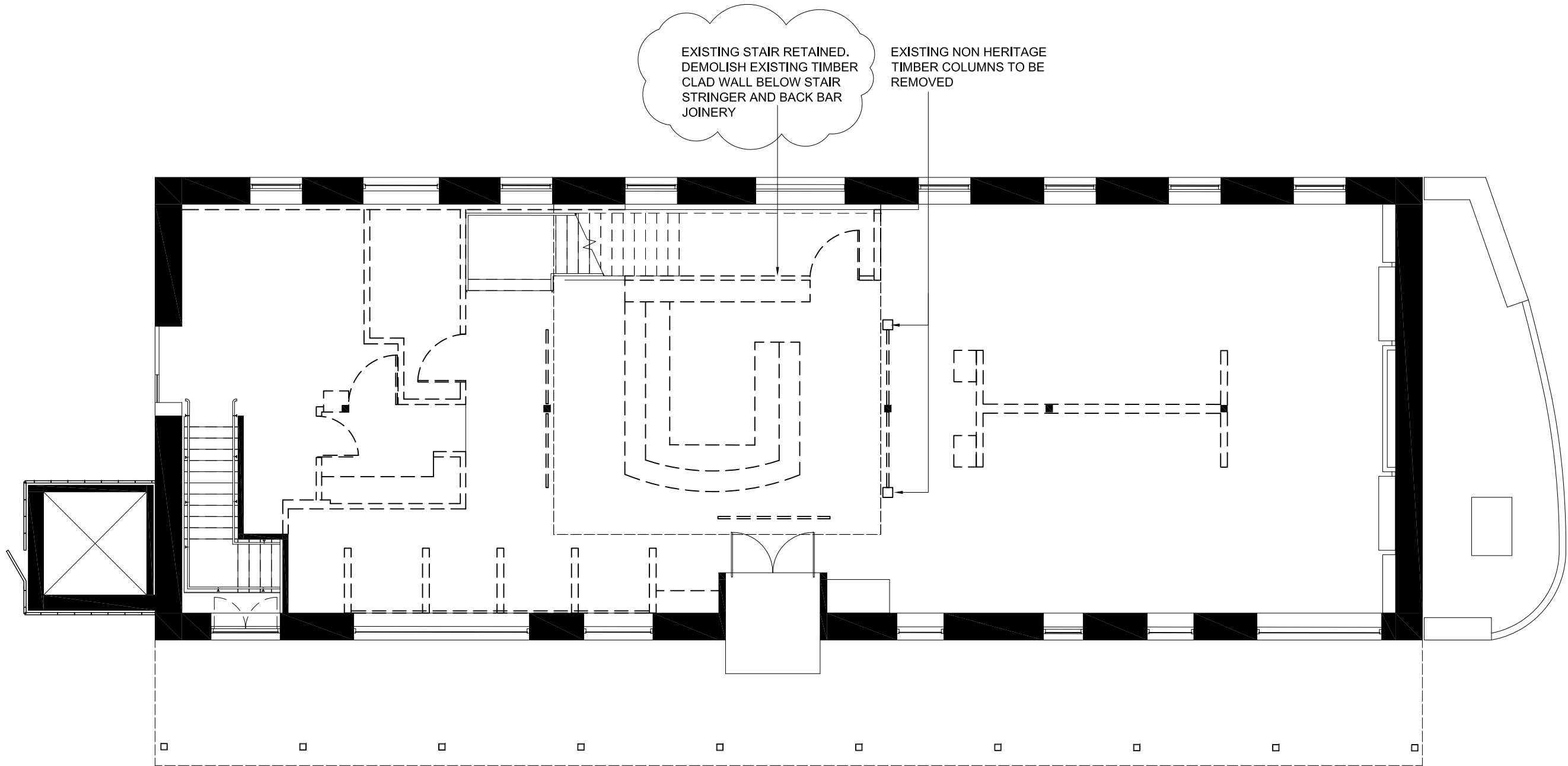
01 - DEMOLITION PLAN
