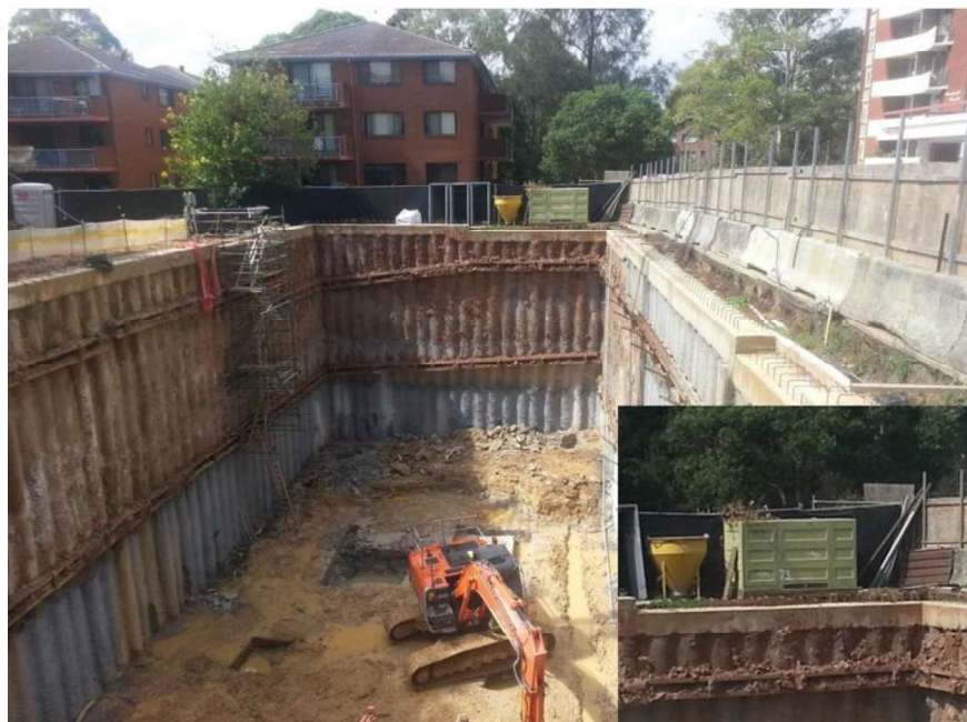
This excavation for a basement at 6 Sorrell Street Parramatta NSW for a mixed use 8 storey development in 2015 was identified by Endeavour Energy's Regional Services North as being unsafe due to the integrity of padmount substation 7858 located on the adjoining lot being compromised and access not being available. This resulted in the 'switching out' of the substation from the network until the site conditions were again deemed to be safe.
