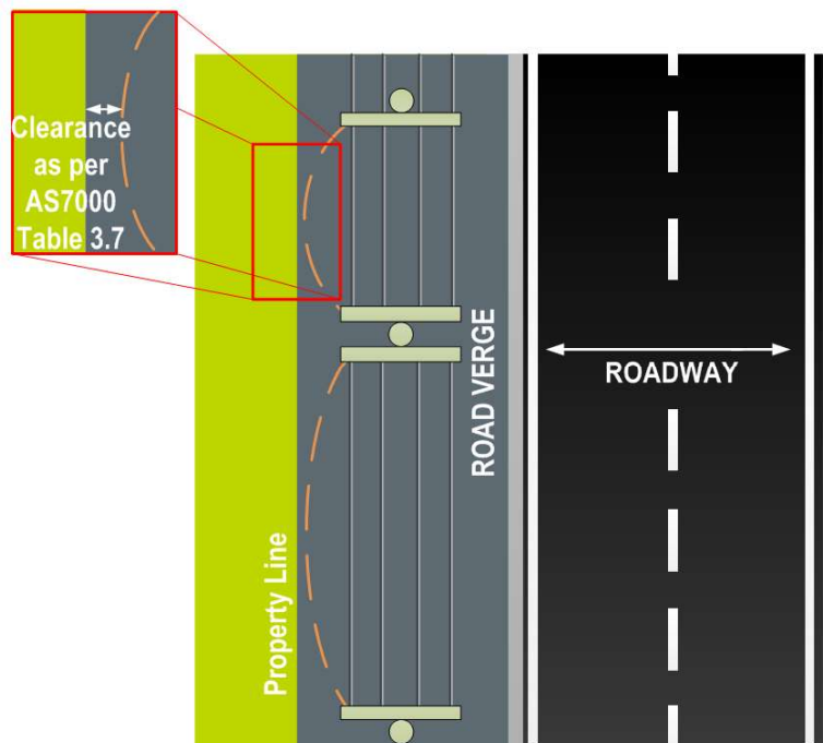
Figure 5 - Roadway requirements
