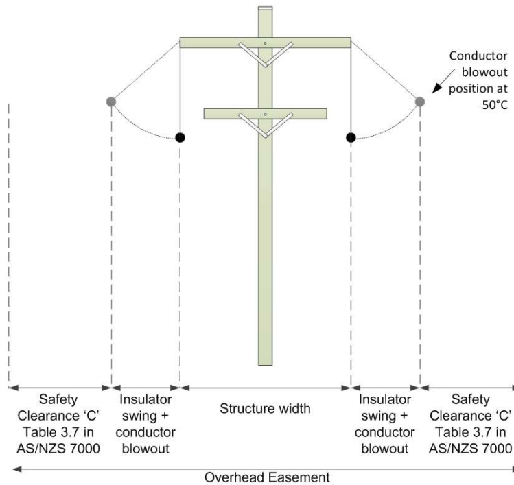
Figure 2 - Minimum overhead easement
