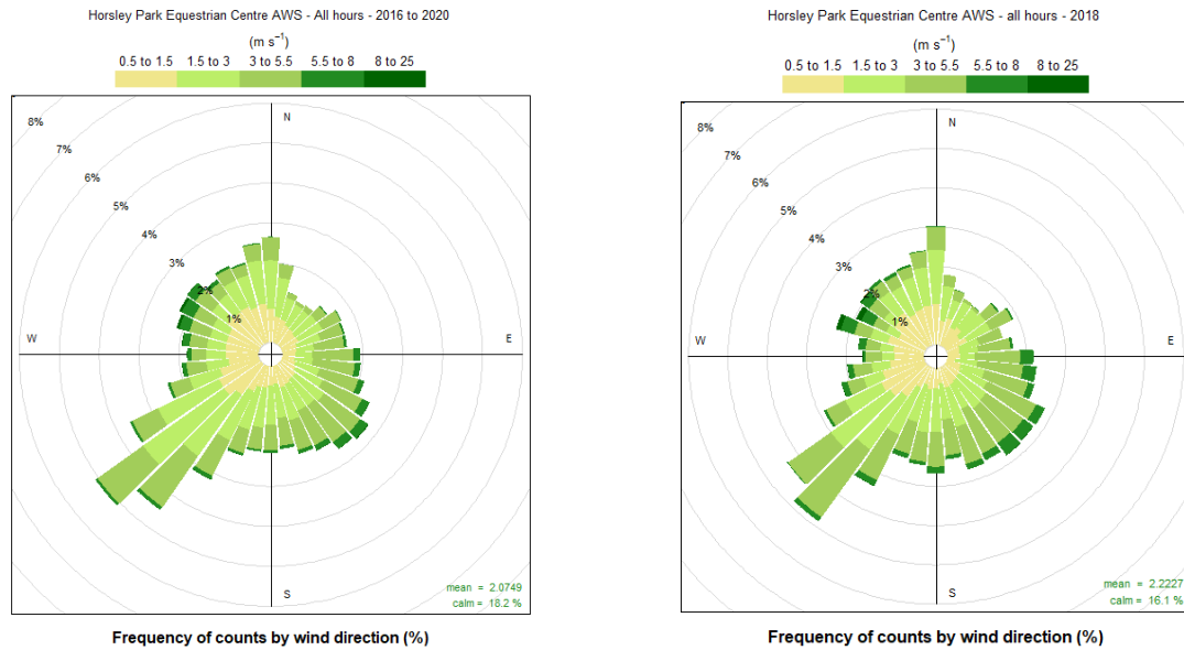
Figure A 3 Annual wind roses 2016 to 2020, and 2018 Horsley Park Equestrian Centre AWS
