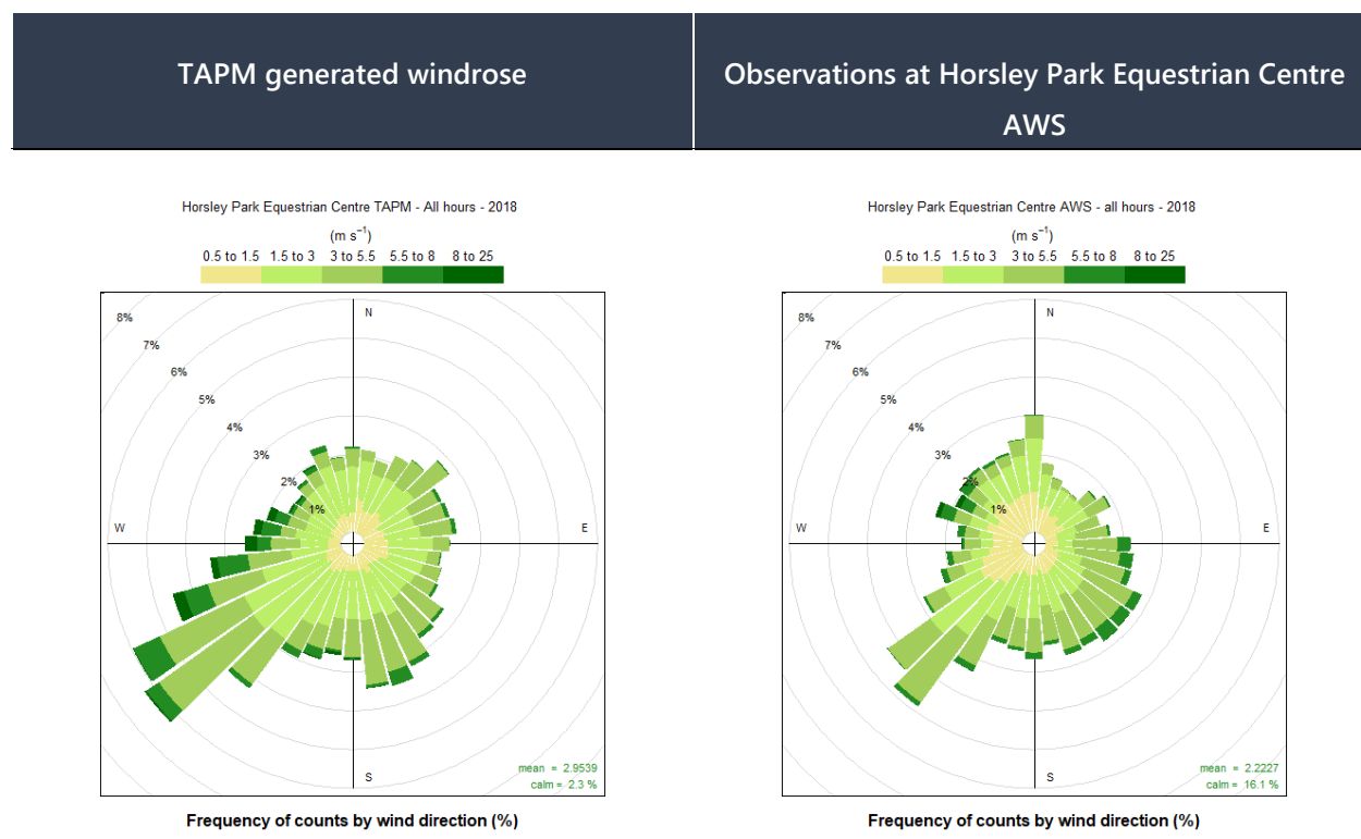
Figure A5 Modelled and observed meteorological data – Horsley Park Equestrian Centre 2018
