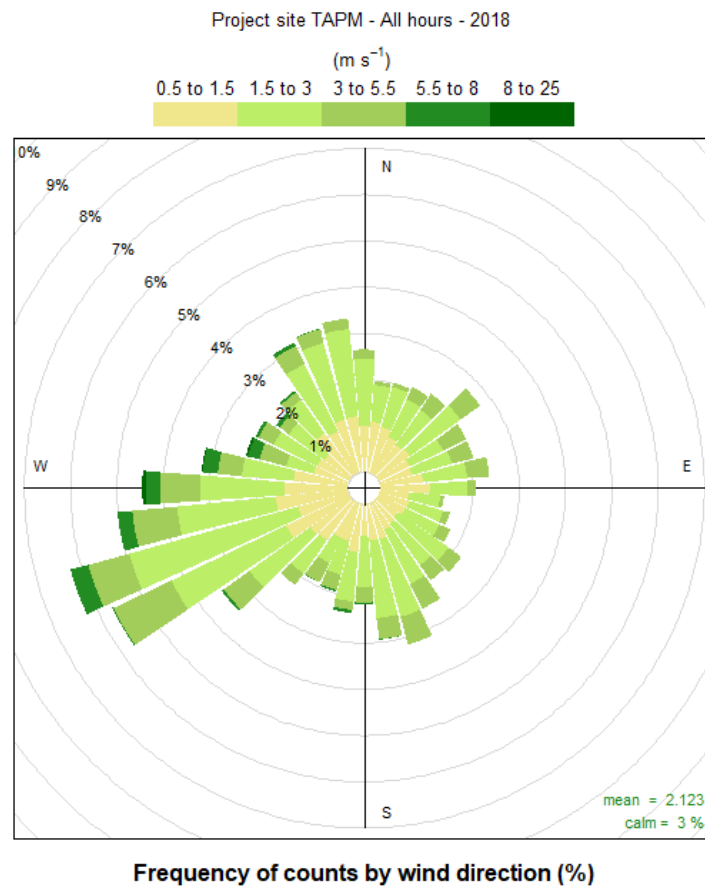
Figure A7 Predicted wind speed and direction – Proposal site 2018
