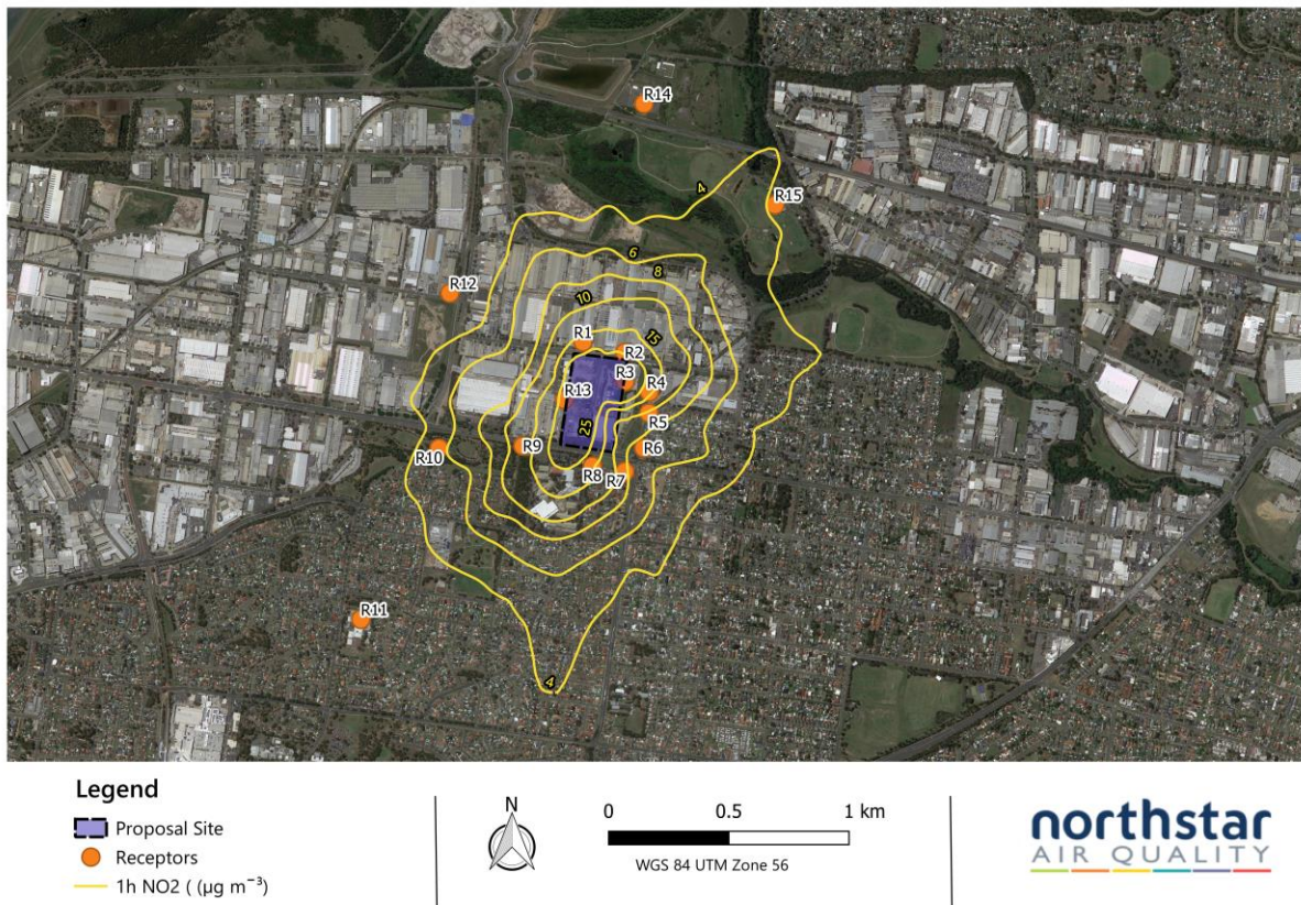
Figure 9 Predicted maximum incremental 1-hour NO 2 impacts
