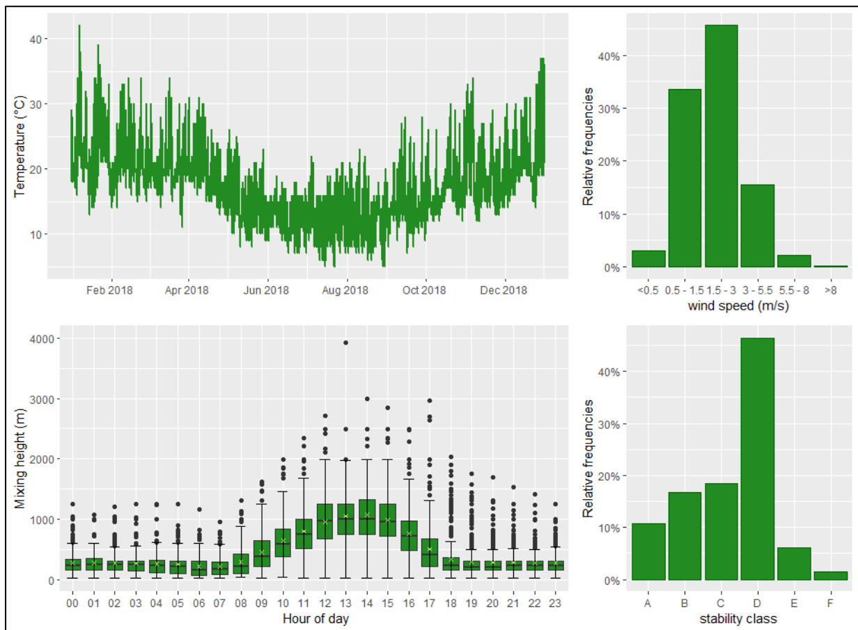
Figure A6 Annual temperature, mixing height and wind speed distribution – Proposal site 2018
