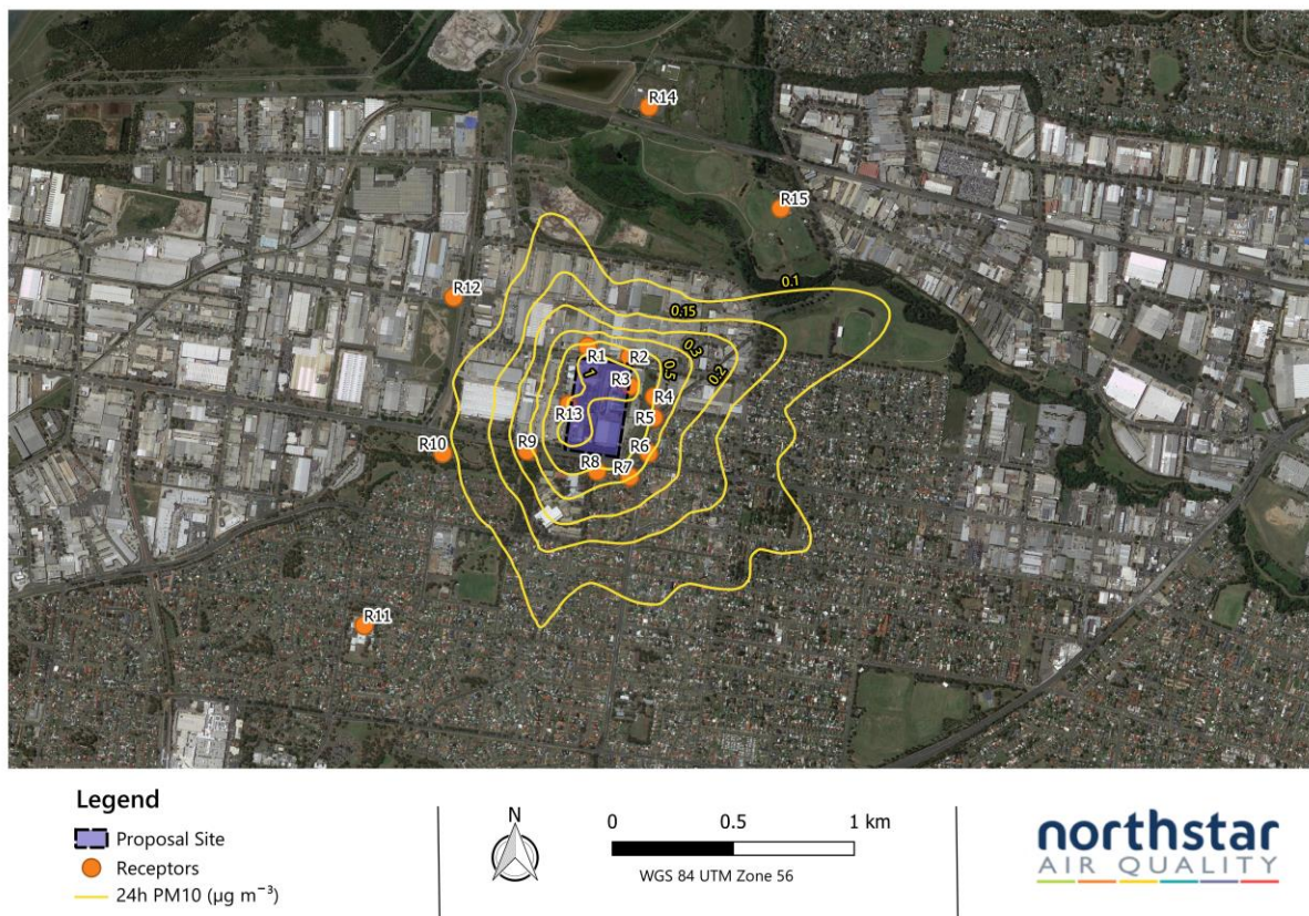
Figure 8 Predicted maximum incremental 24-hour PM 10 impacts
