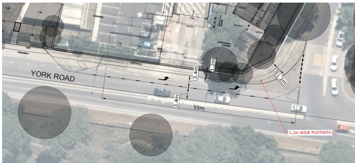
Figure 7.7: Concept Slip-lane Treatment
