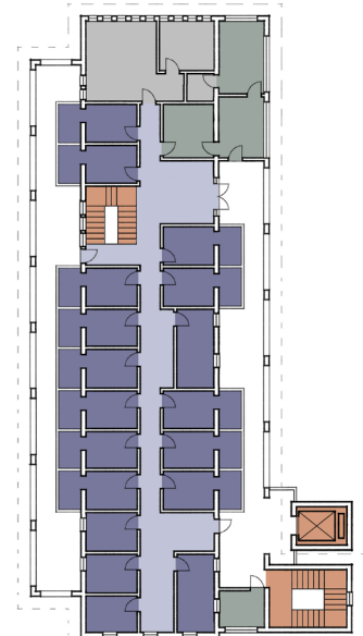
LEVEL 2 MP - 18 BEDS
