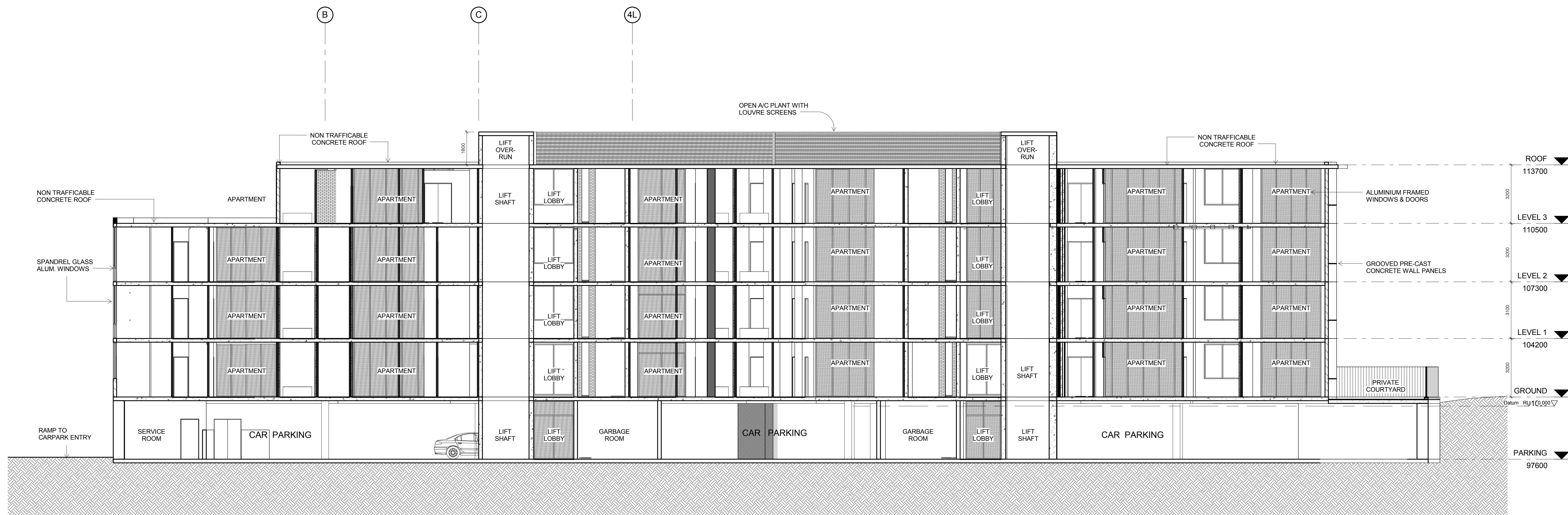
2 SECTION 2 1:100
