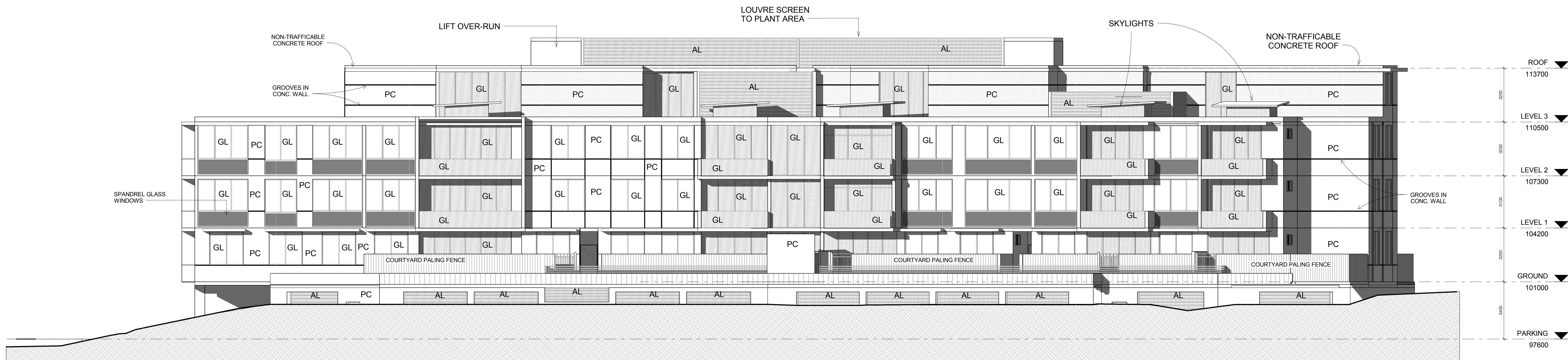
1 SOUTH 1:100
