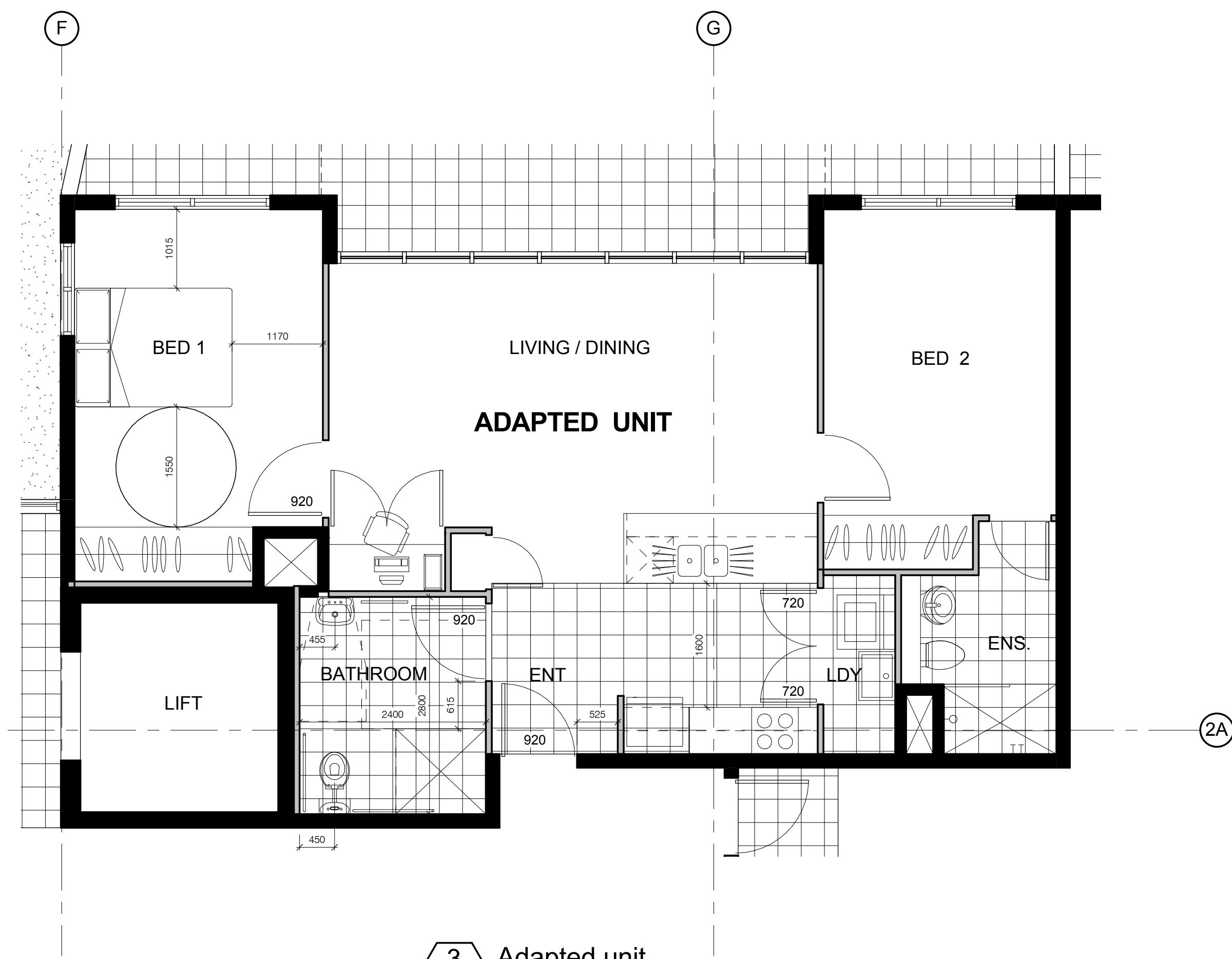
3 Adapted unit 1:50
