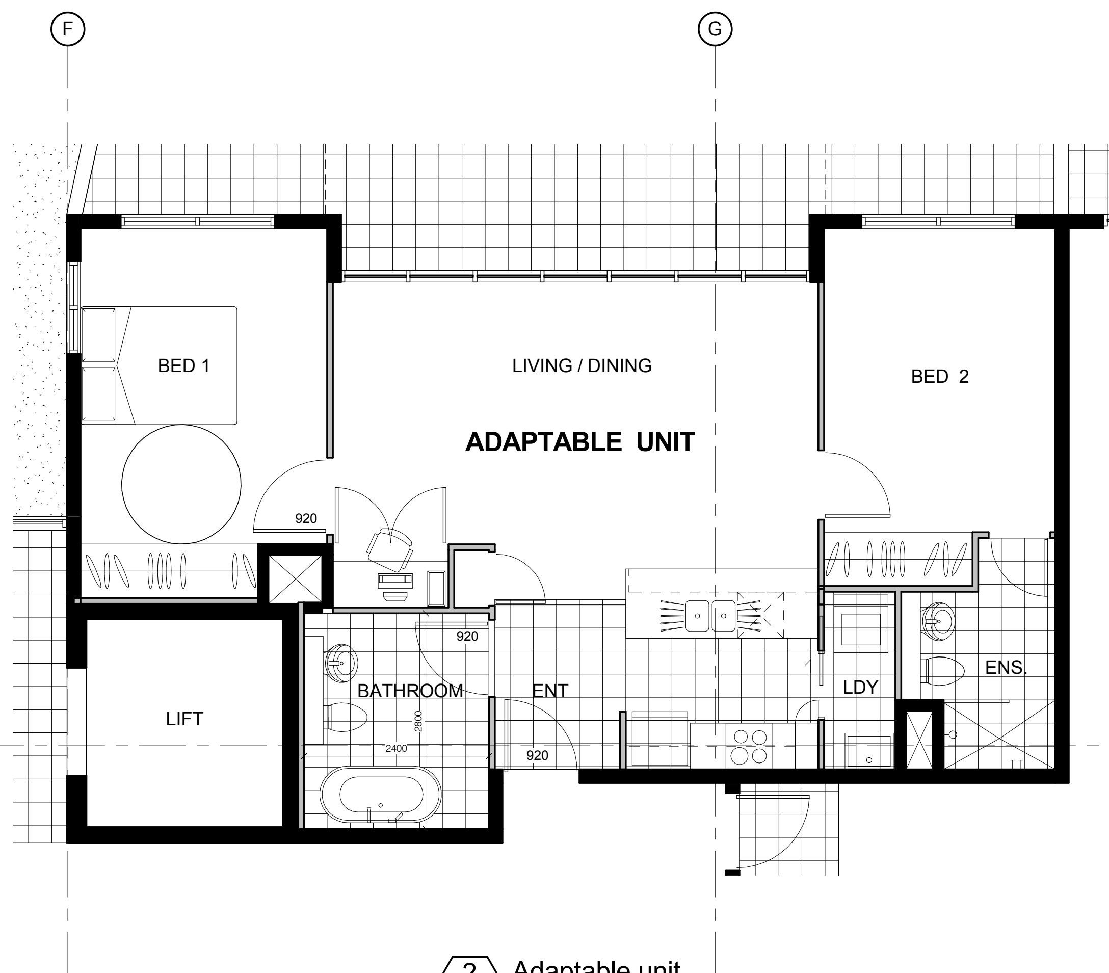
2 Adaptable unit 1:50
