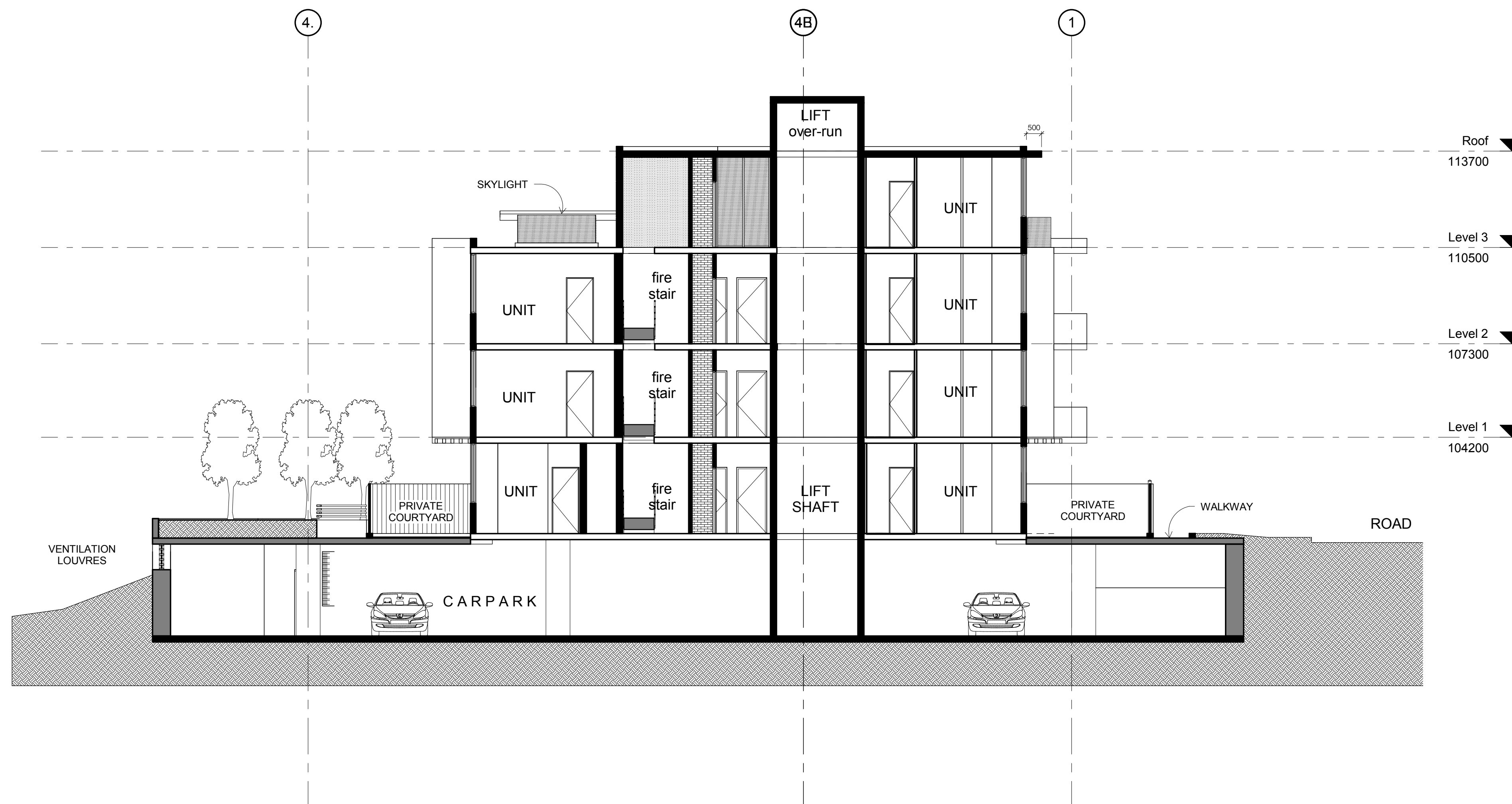
1 SECTION 1 1:100
