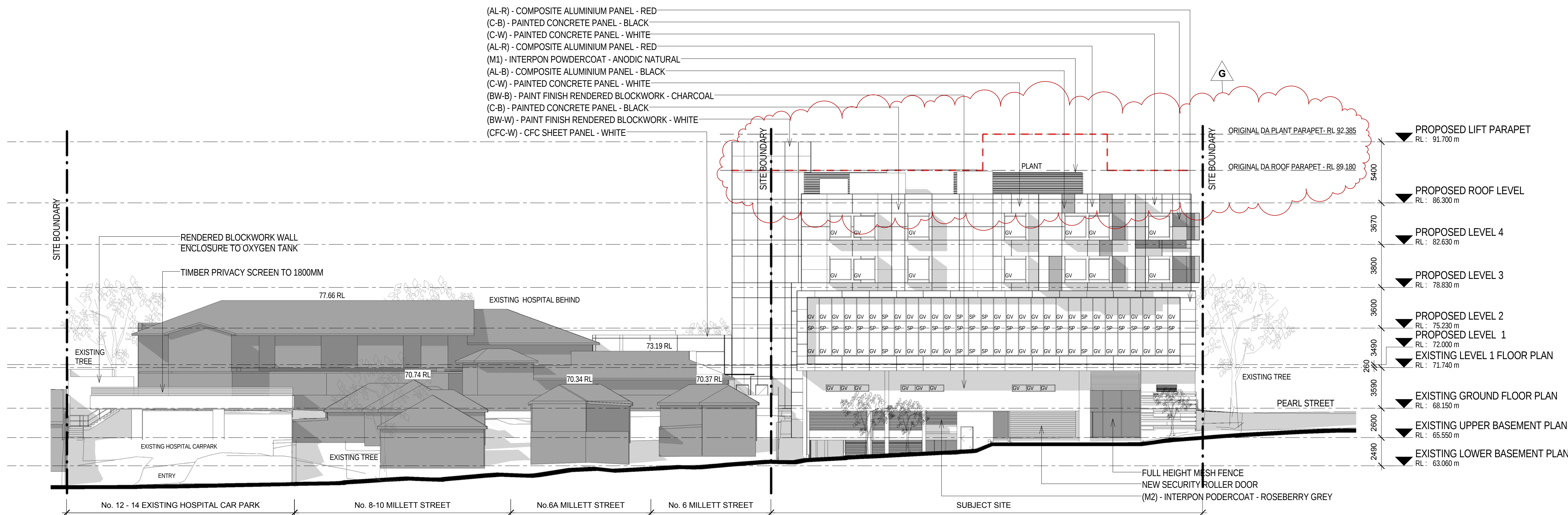
1 GLOUCESTER ROAD - ELEVATION DA-32 Scale 1 : 200
