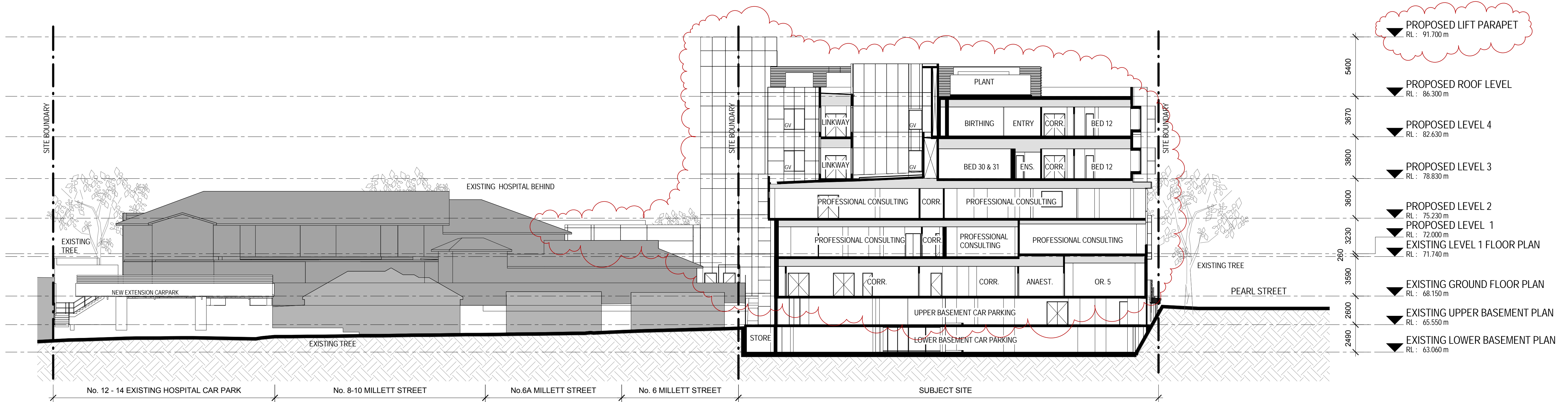
1 SECTION AA DA-32 Scale 1 : 200
