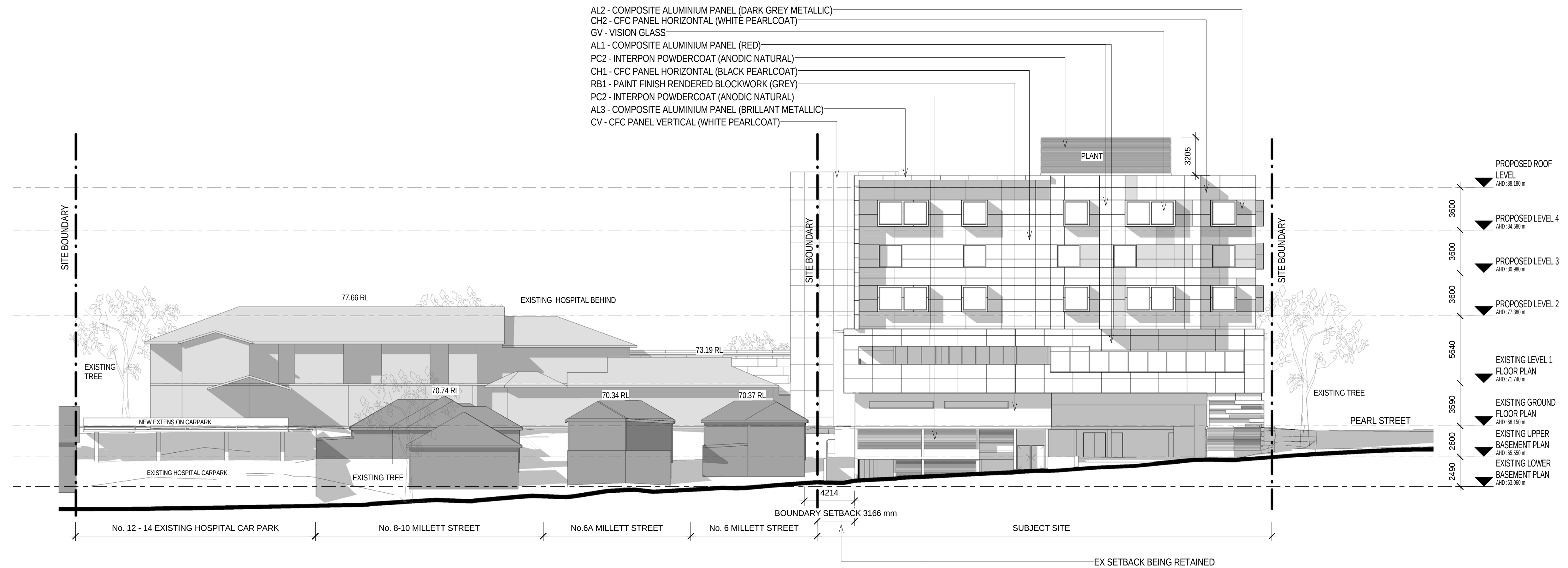
2 MILLETT STREET - ELEVATION DA-32 Scale 1:200
