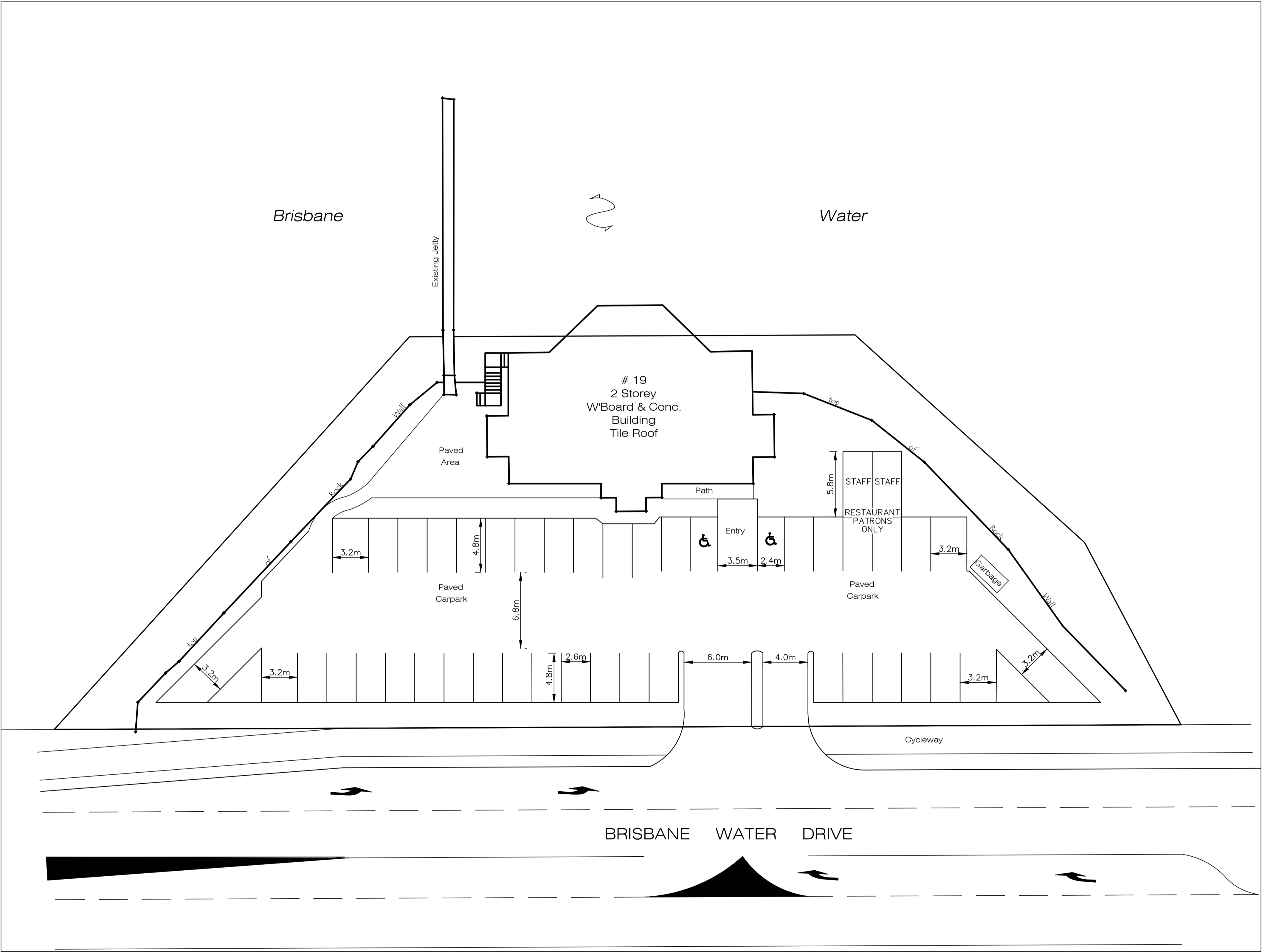
DETAIL PLAN SCALE 1:200
