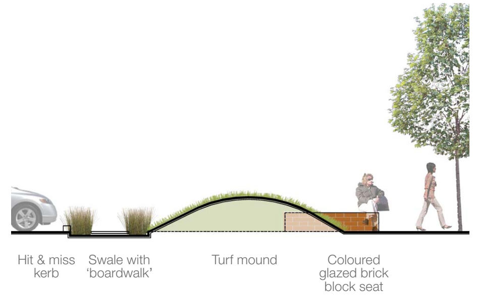
swale / mound
