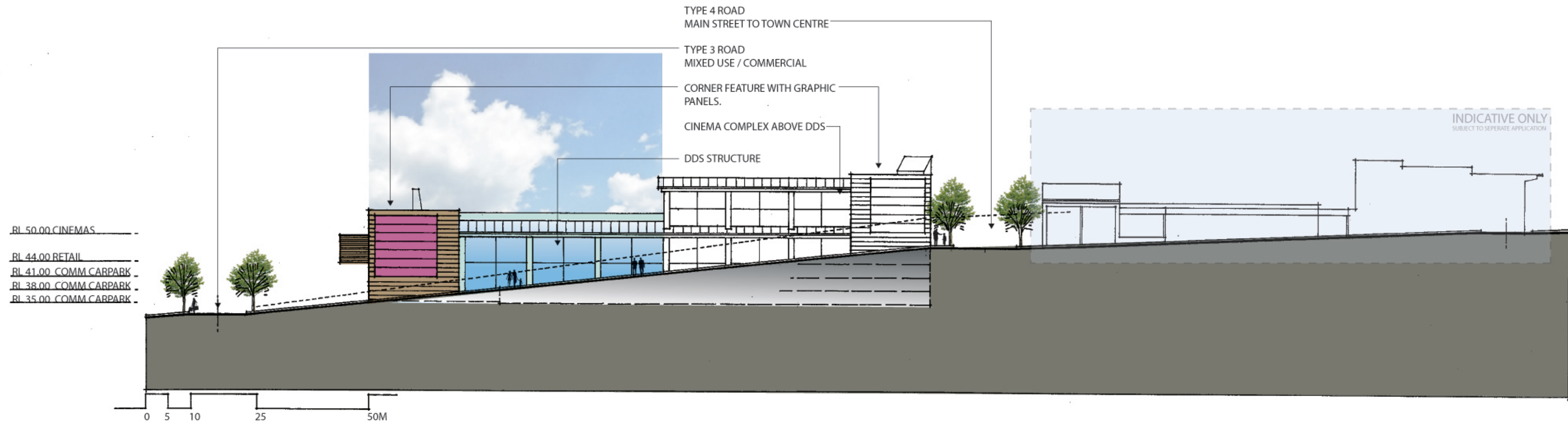
3. EASTERN ELEVATION
