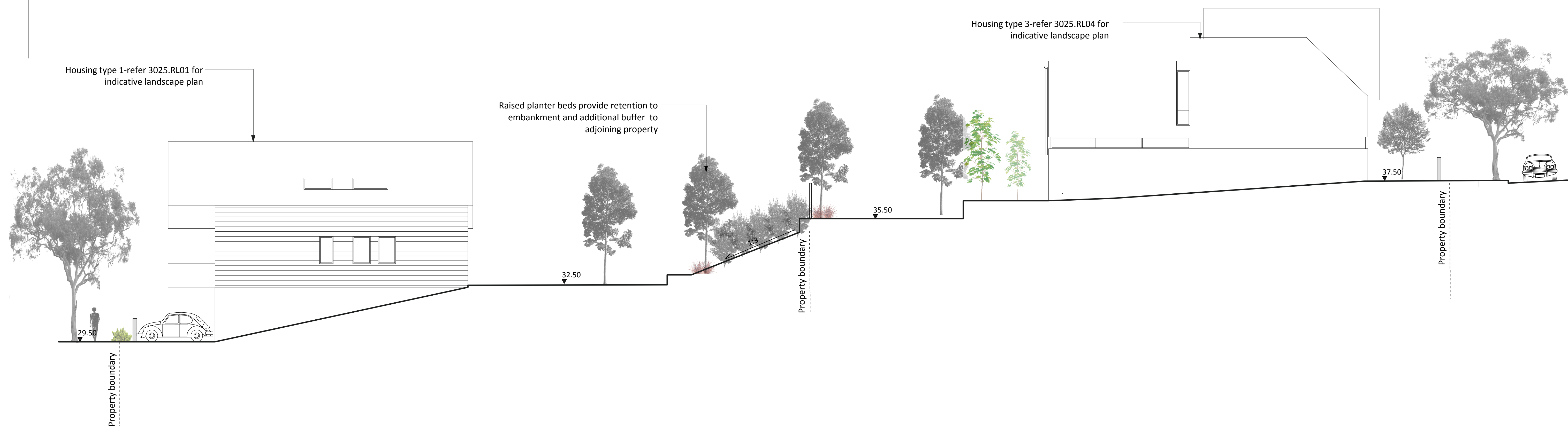
Landscape cross-section AA 1:100
