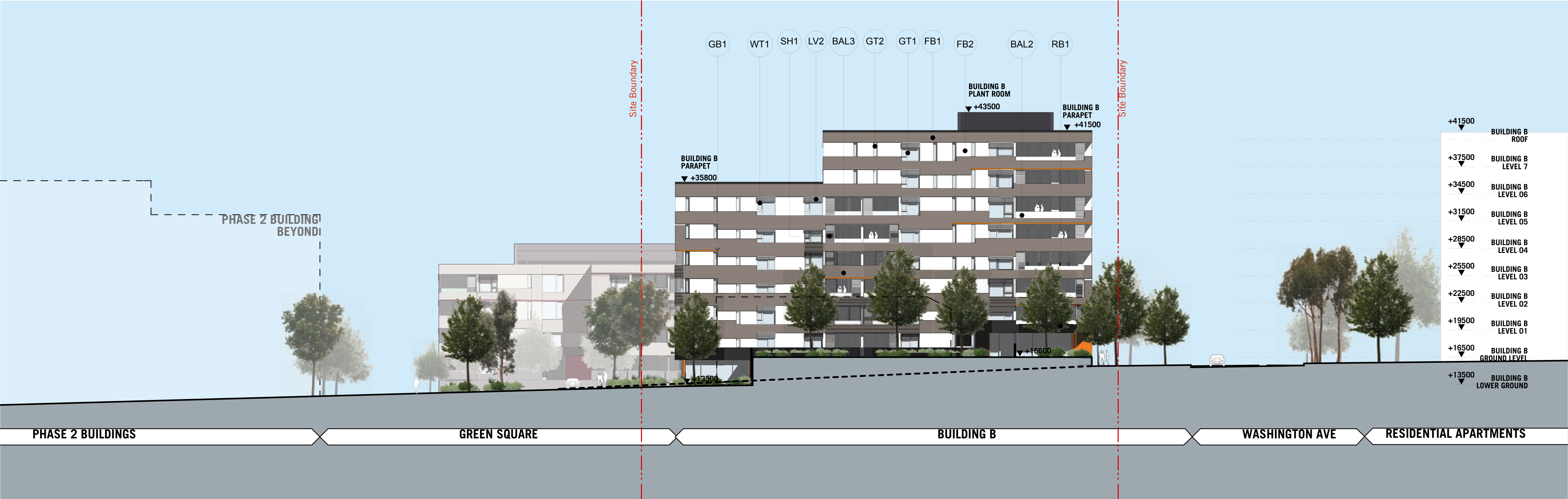
SECTION B-B
