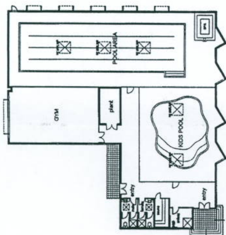
FLOOR PLAN POOL and GYM
