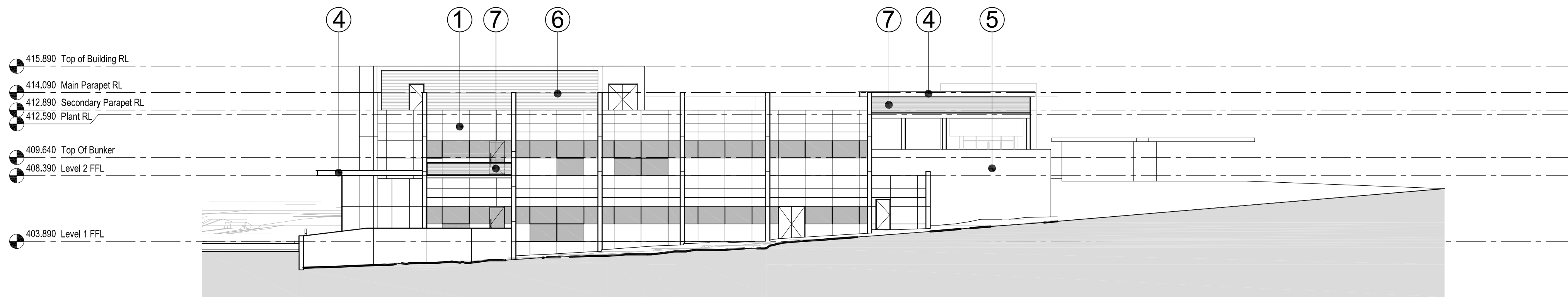
EAST ELEVATION 1:200
