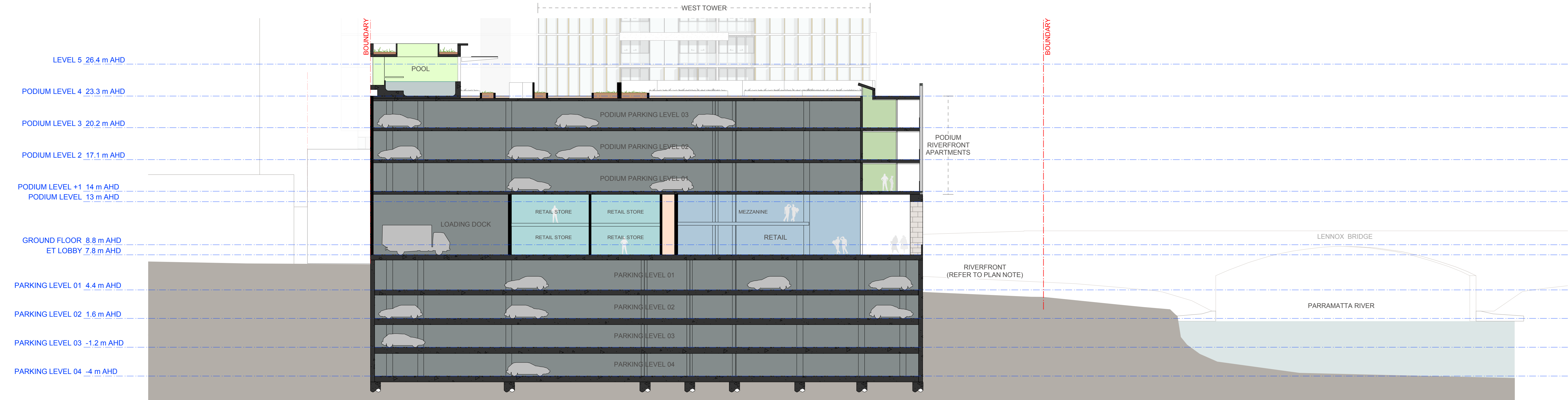
01 SHORT SECTION LOOKING WEST 1:200 @A1
