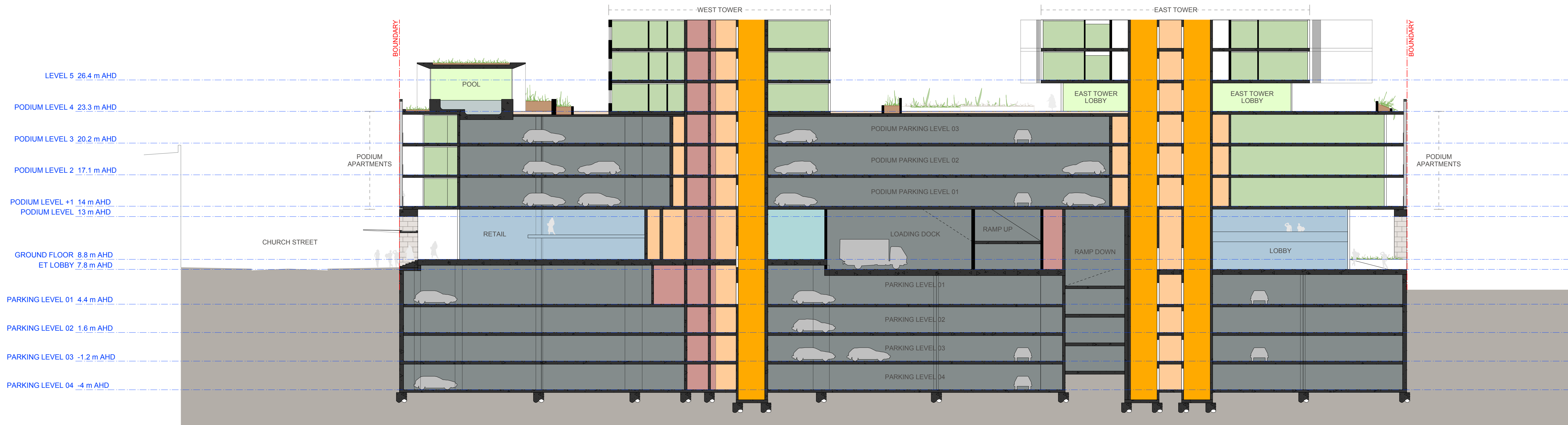
02 LONG SECTION LOOKING NORTH 1:200 @A1
