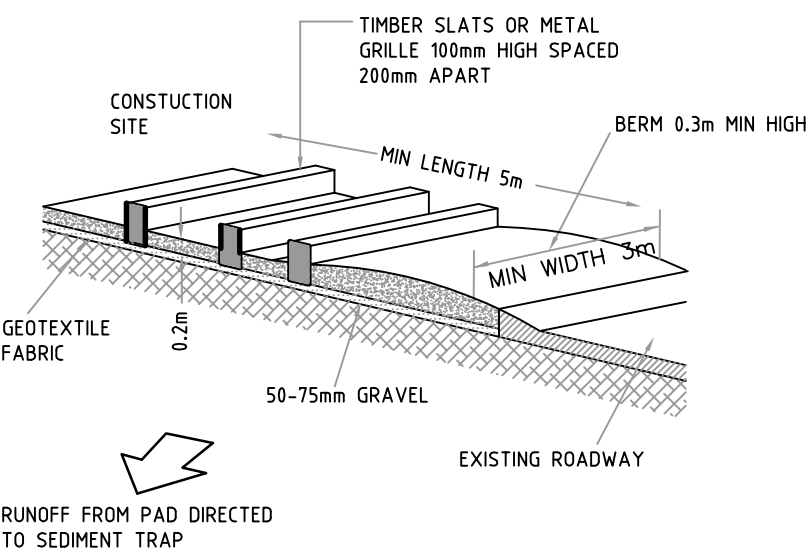
DETAIL C TEMPORARY CONSTRUCTION VEHICLE EXIT
