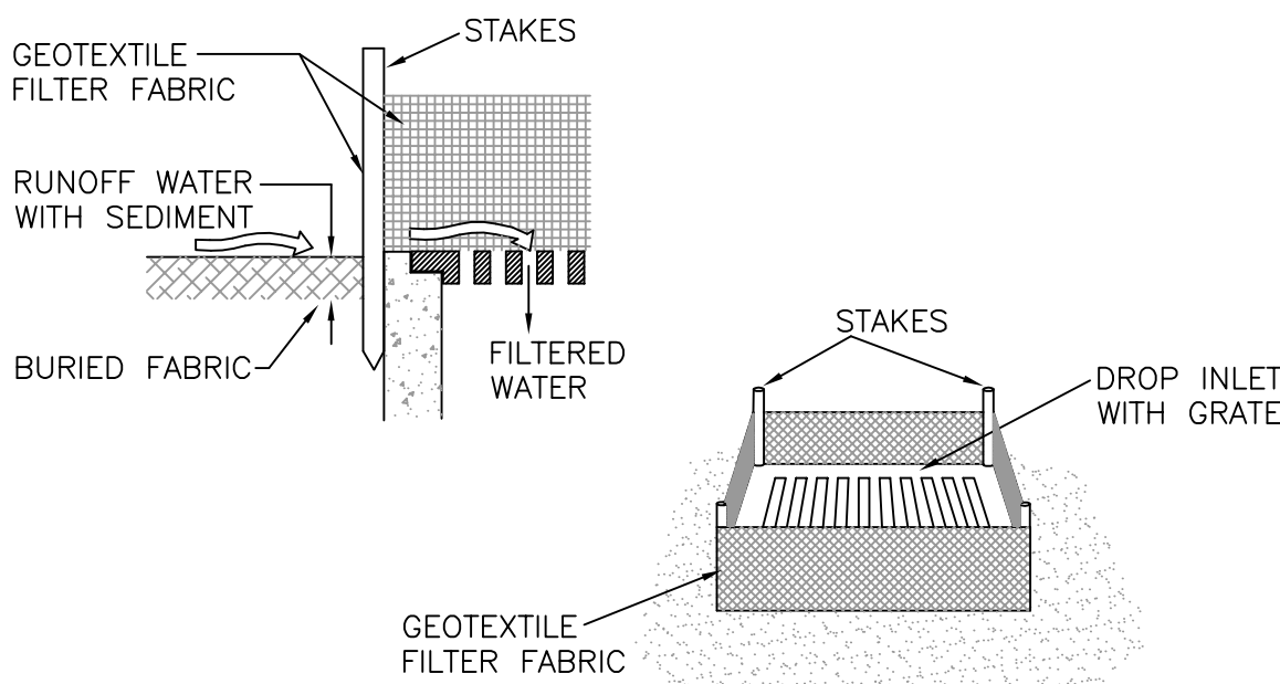
DETAIL B GEOTEXTILE FILTER FABRIC DROP INLET SEDIMENT TRAP
