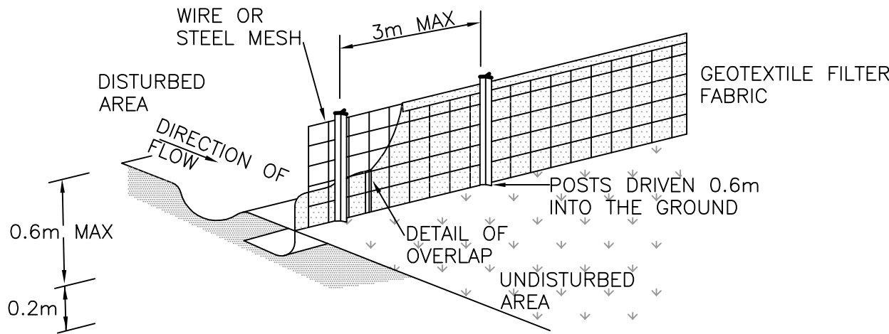
DETAIL A SEDIMENT CONTROL FENCE
