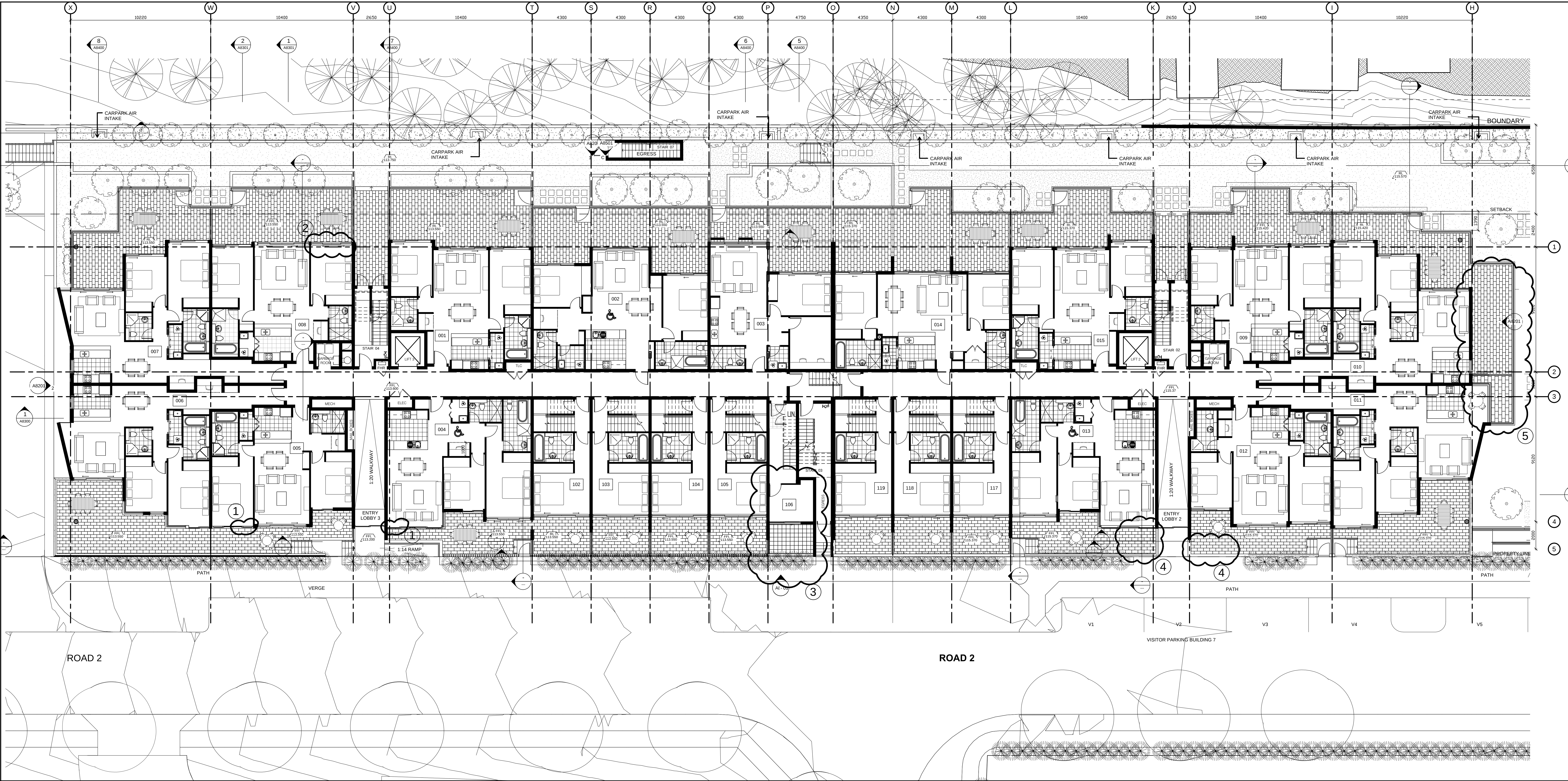
1 BUILDING 8 GROUND FLOOR PLAN 1 : 100
