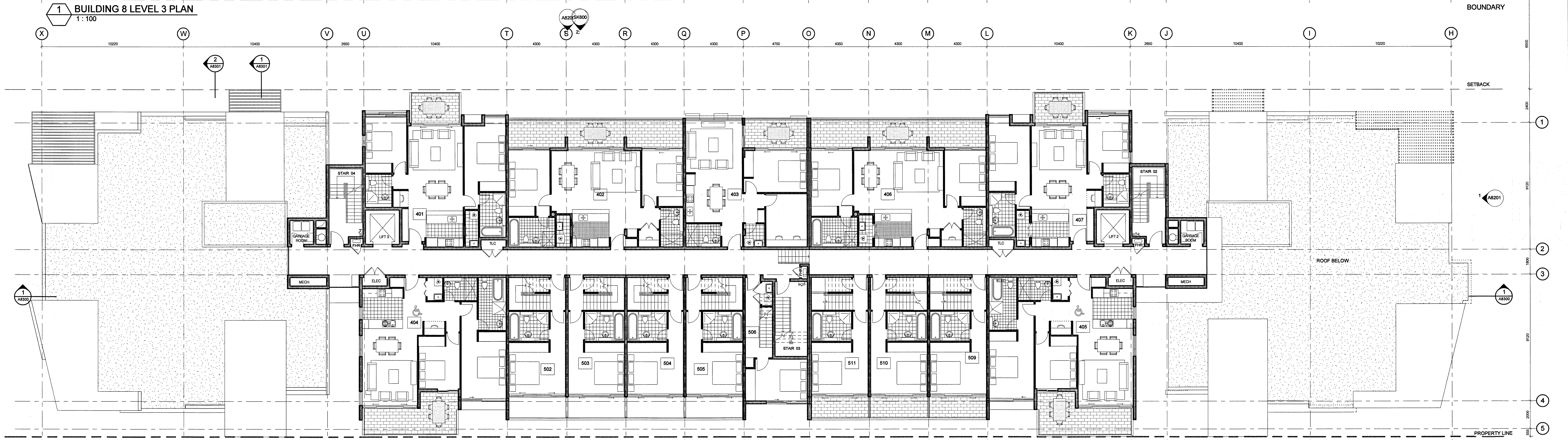
2 BUILDING 8 LEVEL 4 PLAN 1:100
