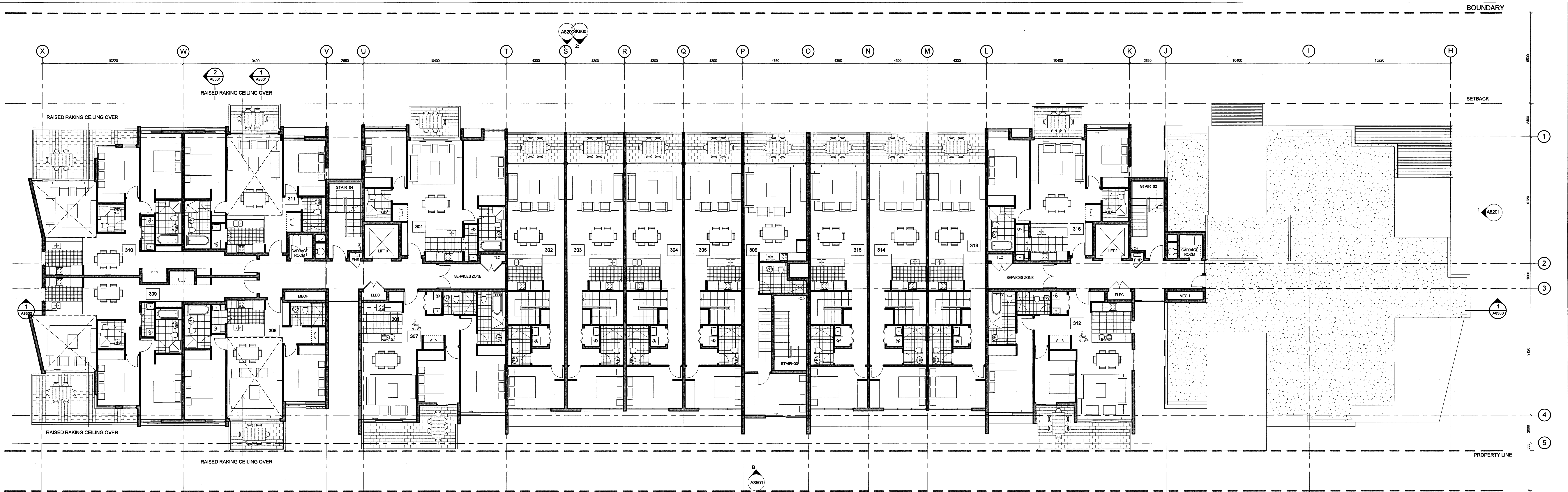
1 BUILDING 8 LEVEL 3 PLAN 1:100
