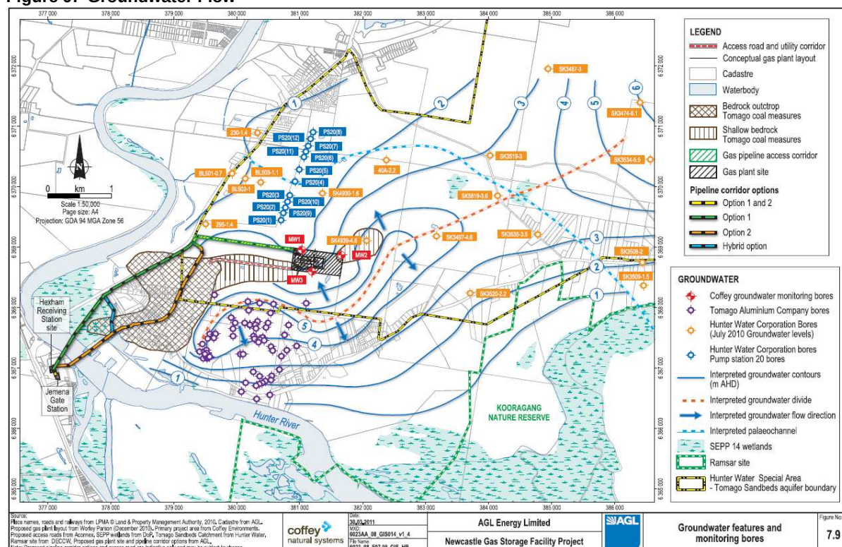
Figure 9: Groundwater Flow
