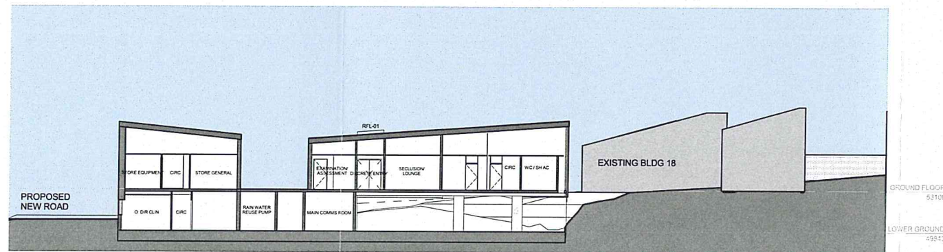
3 SECTION B- NORTH SOUTH DA_F 01 1:200
