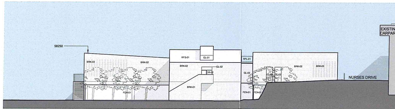
2 ELEVATION NORTH DA_E 02 1:200
