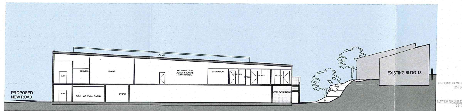
4 SECTION C - NORTH SOUTH-2 DA_F 01 1:200
