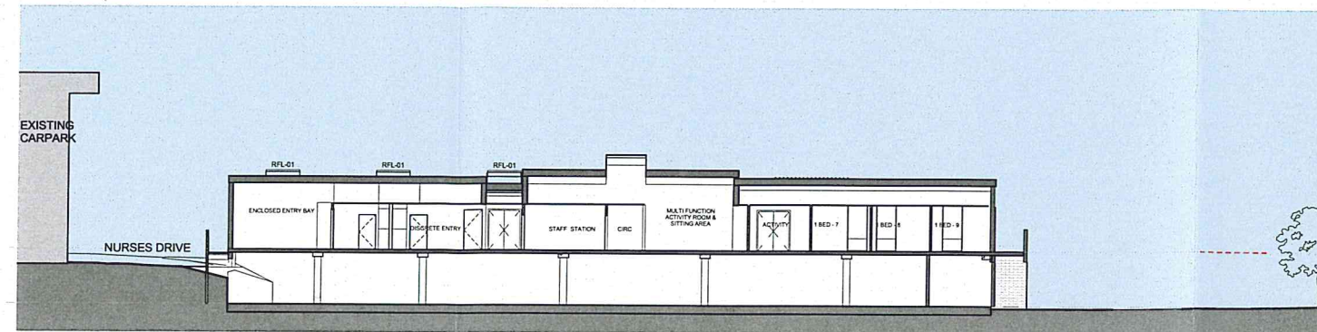
2 SECTION A- EAST WEST DA_F 01 1:200
