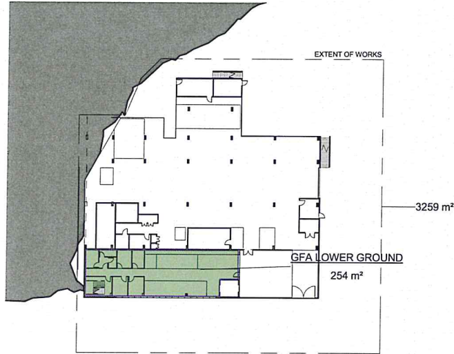
1 LOWER GROUND GFA 1 : 500
